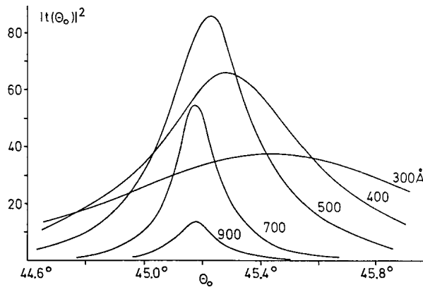
Fig. 2.13. The enhancement factor |t^p|^2 of silver \lambda = 6000 \text{ \AA} for different thickness d . The maximum is reached at I_i = \Gamma_{\text{rad}} (internal damping = radiation damping). \Gamma_{\text{rad}} varies with \exp(-2dk_x^0) . From [2.18]
