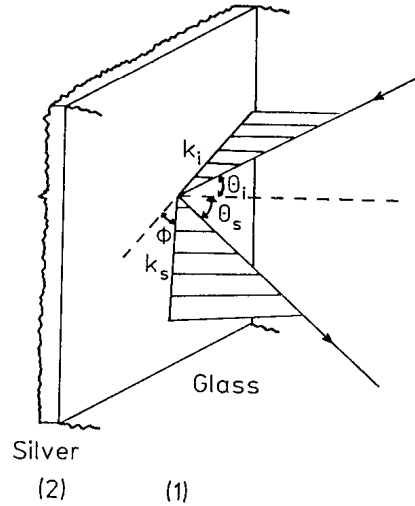
Fig. 3.9. The SP with the wave vector k_x^0 is scattered without changing its absolute value: "directional" scattering
