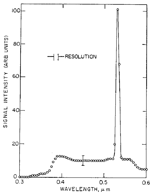
Fig. 4.8. The spectrum of the light signal reflected at a very rough silver film. The incoming light frequency amounts to 1.06\ \mu ; the spectral distribution shows a strong signal at the double frequency. From [4.18]
