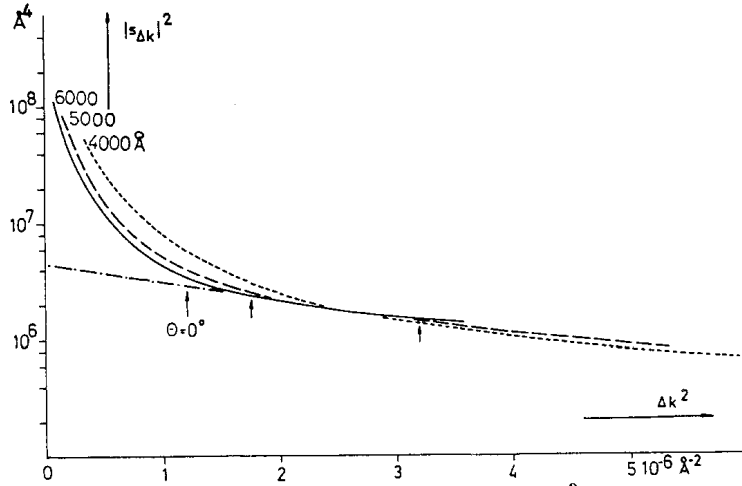
Fig. 3.8. Observed roughness function |s(\Delta k_x)|^2 as a function of (\Delta k_x)^2 for a silver film, 550 Å thickness, at different wavelengths. The arrows indicate \theta = 0^\circ or \Delta k_x = \sqrt{\varepsilon_0}(\omega/c) \sin \theta_0 , the observation is along the normal of the surface. The solid angle of the light detector is \delta\Omega = 4 \times 10^{-3} sr. The back-scattered light, right side of the curve, is determined by the roughness of the silver surface. From [3.1]
