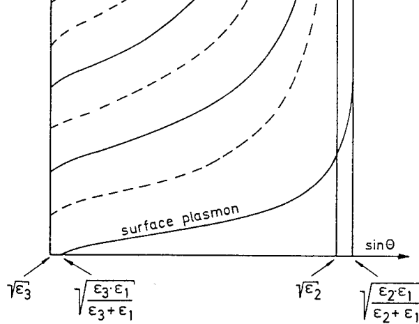
Fig. 2.19. Thickness dispersion: the relation between the thickness ( d_2 ) of the wave-guiding film ( \epsilon_2 ) and the angle of incidence ( \sin \theta ) in an asymmetric layer system: \epsilon_1/\epsilon_2/\epsilon_3 , \epsilon_1 metal film, \epsilon_3 \neq \epsilon_1 , for a given frequency \omega . Between the light lines c/\sqrt{\epsilon_3} and c/\sqrt{\epsilon_2} in a \omega(k_x) diagram or in the present d vs. \sin \theta diagram at k_x/(\omega/c) = \sqrt{\epsilon_3} and \sqrt{\epsilon_2} the light modes exist, except the m_p = 0 or the SP mode which starts at [\epsilon_1 \epsilon_3 / (\epsilon_1 + \epsilon_3)]^{1/2} for d_2 = 0 and converges to [\epsilon_1 \epsilon_2 / (\epsilon_1 + \epsilon_2)]^{1/2} , for d_2 \rightarrow \infty . From [2.3a]
