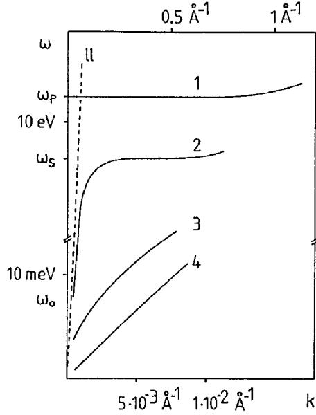
Fig. 1.1. Scheme of the dispersion of plasmons in a solid. (1) volume plasmons, (2) surface plasmons, (3) plasmons in a two-dimensional electron gas, (4) plasmons in a one-dimensional system. The upper scale is valid for (1) and (2), the scale below for (3) and (4). ll is the light line
