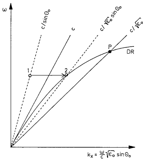
Fig. 2.7. The ATR method: Dispersion relation DR of SPs for a quartz/metal/air system \epsilon_2 = 1 , c : light line in vacuum, c/\sqrt{\epsilon_0} : light line in the medium \epsilon_0 . Since the light line c/\sqrt{\epsilon_0} lies to the right of the DR up to a certain k_x , light can excite SPs of frequencies \omega below the crossing point P on the metal/air side. The SPs on the interface 0/1 metal/quartz cannot be excited, since their DR lies to the right of c/\sqrt{\epsilon_0} because \epsilon_0 > 1
