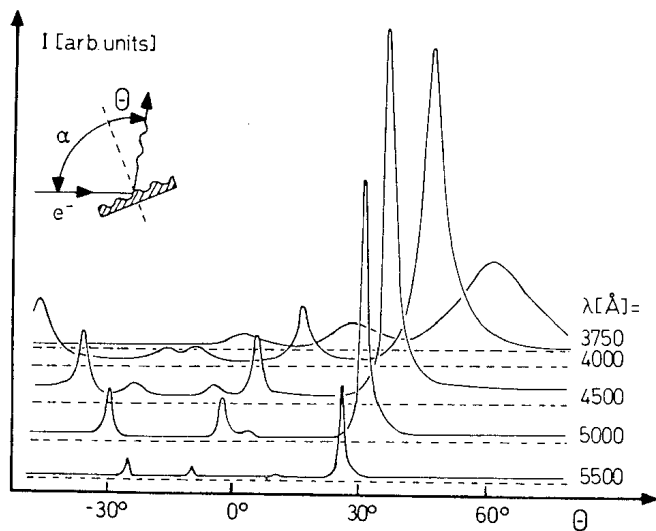
Fig. 6.14. Light of various wavelengths emitted from a sinusoidal grating ( a = 8850 Å, h \sim 500 Å) which is irradiated with 80 KeV electrons at an angle of incidence of \alpha = 70^\circ . From [6.22]
