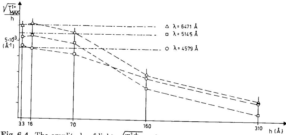
Fig. 6.4. The amplitude of light \sqrt{T_{\max}^{(-1)}} emitted from a grating with a = 5930 \text{ \AA} into the first-order diffraction divided by the amplitude h as a function of h at different wavelengths. The horizontal line (---) represents the result calculated with the first-order approximation. From [6.4]
