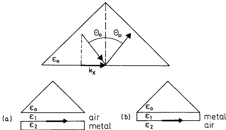
Fig. 2.8a,b. Configuration of the ATR method. (a): The dielectric (air) lies between the prism and the metal surface, Otto configuration. (b): The metal contacts the prism and couples the SPs with the evanescent field of the totally reflected light wave, Kretschmann-Raether configuration. From [2.3a]
