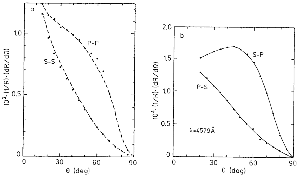
Fig. 5.8. (a) The intensity (1/I_0)dI/d\Omega scattered from a rough silver film as a function of the scattering angle \theta . Normal incidence ( \theta_0 = 0 ). \lambda = 4579 \text{ \AA} . A four parameter fit gives \delta = 40 \text{ \AA} and \sigma = 790 \text{ \AA} and for the waviness 4 \text{ \AA} and 7000 \text{ \AA} . (b) The same sample yields the angular distribution for the s-p and p-s intensities. \lambda = 4579 \text{ \AA} . From [5.12]
