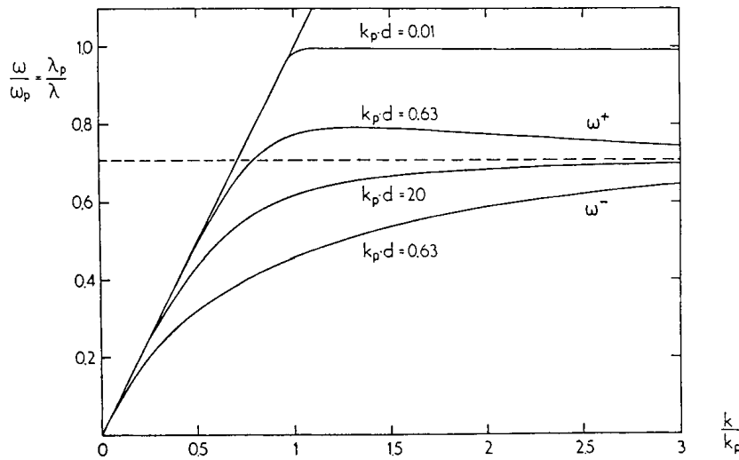
Fig. 2.23. Dispersion relations of nonradiative surface plasmons of films of different thickness d (at constant k_p ). k_p d = 0.63 means, e.g., at a plasma wavelength of \lambda_p = 6000 \text{ \AA} : d = 630 \text{ \AA} ; k_p = 2\pi/\lambda_p . k_p d = 20 represents a very thick film, so that the SPs of both sides are almost decoupled and the curve is identical with the dispersion relation of a single boundary metal/dielectric. The metal is assumed as free electron gas. From [2.3b]
