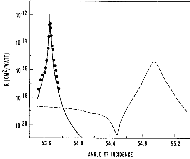
Fig. 2.32. Reflected second-harmonic intensity from the ATR device Fig. 2.29 as a function of the angle of incidence in the prism. The thin metal film ( c ) of 135 \text{ \AA} lies between an oil film ( b ) and a quartz crystal ( d ). By mechanical pressure between ( a ) and ( d ) which changes the thickness of the oil film ( b ), the optimal coupling of the fundamental SP ( \lambda = 1.06 \mu ) into the system can be reached; it is d(b) = 30\,000 \text{ \AA} . The high field at the metal/quartz interface and the nonlinearity of the quartz produce the 2\omega radiation peak (full circles). For comparison the dashed line displays the SH intensity at a single boundary. From [2.50]
