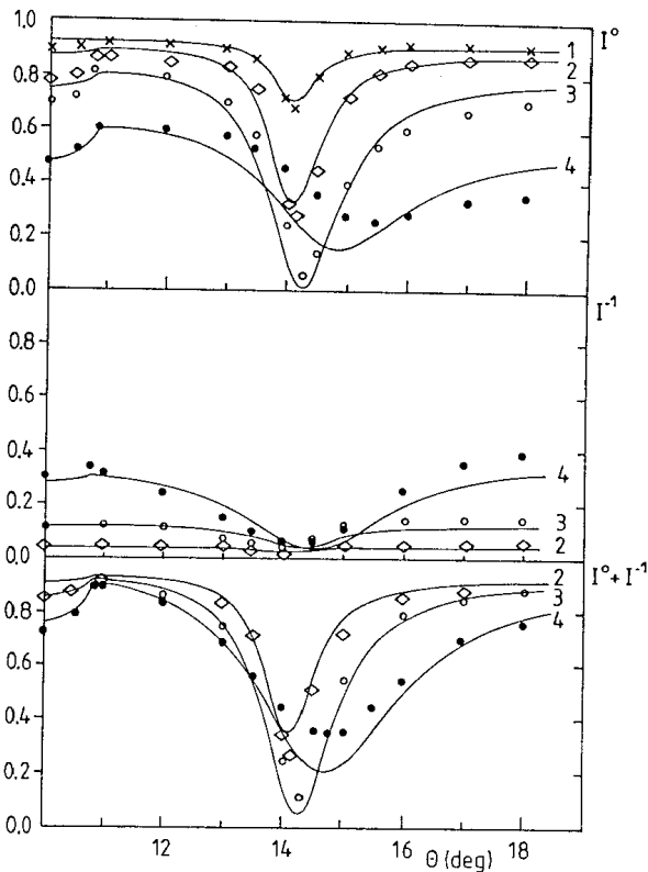
Fig. 6.10. Observed (points) and calculated (full lines) intensity reflected at a sinusoidal gold (interference) grating with a = 7965 \text{ \AA} and \lambda = 6471 \text{ \AA} . I^0 and I^{-1} are the intensities in the zeroth and (-1)st diffraction order; I^0 + I^{-1} means the sum of both light intensities. These are relative intensities referred to the incoming intensity ( I_0 ). The amplitude h of the profile is given as a parameter: (1) 89 \text{ \AA} , (2) 174 \text{ \AA} , (3) 308 \text{ \AA} , (4) 514 \text{ \AA} . The deepest minimum occurs at h = 300 \text{ \AA} , at which an enhancement of |t^p|^2 \approx 59 is calculated using (\epsilon', \epsilon'') = (-9.75; 1.1) . The displacement of the minimum to higher angles and the increasing width of the minimum with larger h display the dependence of the dispersion relation of SP. (o) : amplitude h of the grating. From [6.16]
