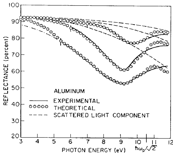
Fig. 5.11. Comparison of measured and calculated reflectivity of rough surfaces of evaporated Al films of 800–1000 Å thickness; angle of incidence 10^\circ . For the calculated curves the parameter (\delta, \sigma) in Å have been taken: (12.1; 918), (14.7; 744), and (37.7; 378), from top to bottom. From [5.17]
