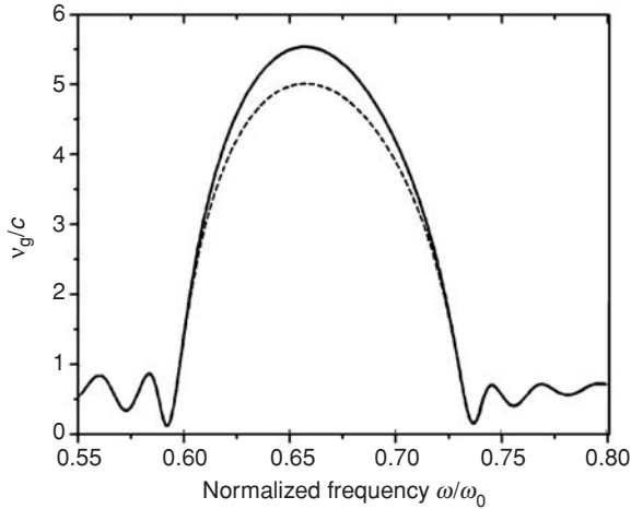
Fig. 10.4 The tunneling velocities defined as v_g = L/\tau_{\text{dwell}} (solid line) and v_g = L/\tau_\varphi (dashed line) in the photonic gap region and adjacent spectral ranges calculated for the 20-period structure discussed in Section 7.11 (see Fig. 7.32) [15].
