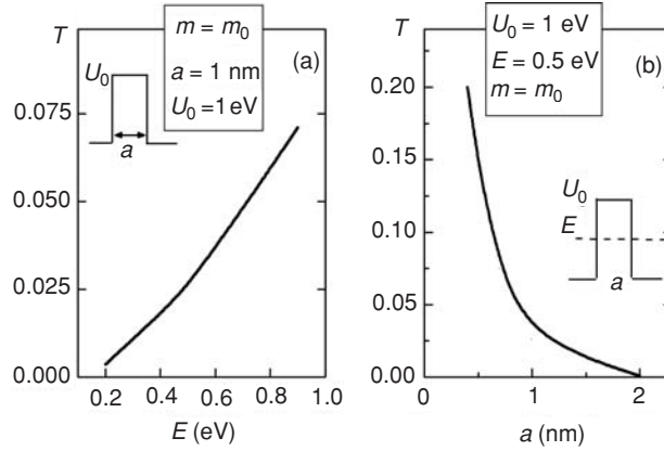
Fig. 3.13 Probability of an electron tunneling through a rectangular barrier with height U_0 = 1 eV as a function of (a) electron energy E and (b) barrier width a .
