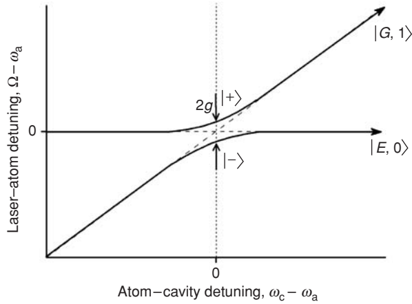
Fig. 15.1 “Atom+field” diagram for the two lowest excited states of the atom-cavity system. |G, 1\rangle is the superposition state with one photon in the cavity and the atom in the ground state. |E, 0\rangle is the superposition state with no photon in the cavity and the atom in the excited state. The dashed lines show the uncoupled states.
