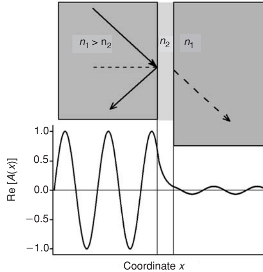
Fig. 3.16 Frustrated total reflection in optics. Evanescent wave behind the high-refraction slab generates the transmitted plane wave provided that the thin (as compared to wavelength) low-refraction layer is followed by the high refraction medium.
