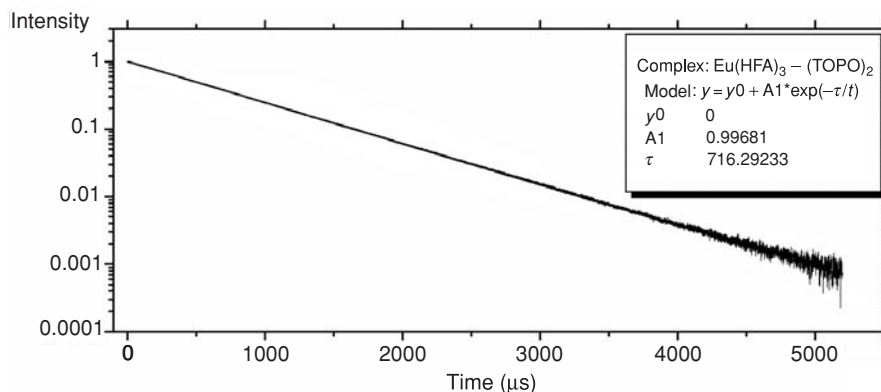
Fig. 13.2 Decay of excited \text{Eu}^{3+} ions in a complex with an organic ligand in toluene solution. It exhibits with high accuracy a single-exponential behavior with lifetime \tau = 716.3\mu\text{s} . Intensity versus time dependence in a semi-logarithmic presentation obeys a straight line with high precision.
