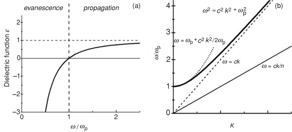
Properties of a gas of charged particles. (a) Dielectric function. (b) Dispersion law.
