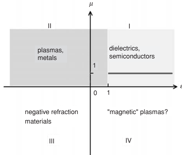
Fig. 11.12 Possible combinations of the dielectric permittivity and the magnetic permeability of materials.
