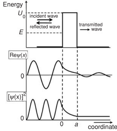
Fig. 3.12 A rectangular potential barrier (top), a particle wave function (middle) and probability density (bottom) for the case when the electron energy E is lower than the potential height U_0 .
