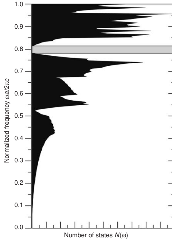
Fig. 14.13 Calculated photon density of states for a three-dimensional photonic crystals whose design and band structure were presented in Figure 7.23. Gray band indicates the band gap. Reprinted with permission from [70]. Copyright 2007, Elsevier B.V.
