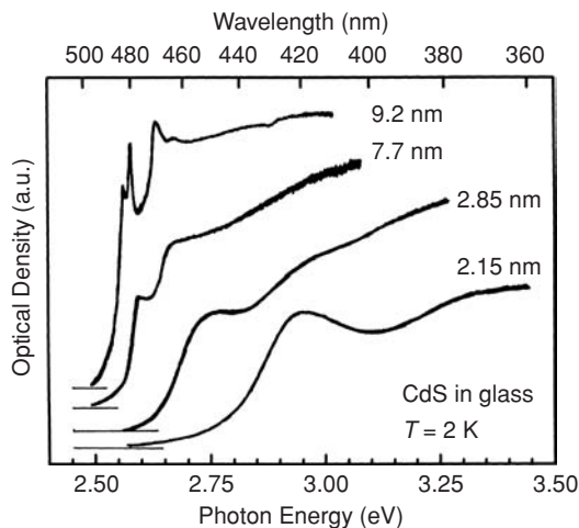
Fig. 5.14 Absorption spectra of CdS nanocrystals in a glass matrix for four different mean radii (9.2, 7.7, 2.85, 2.15 nm) measured at 2 K [8, 34].
