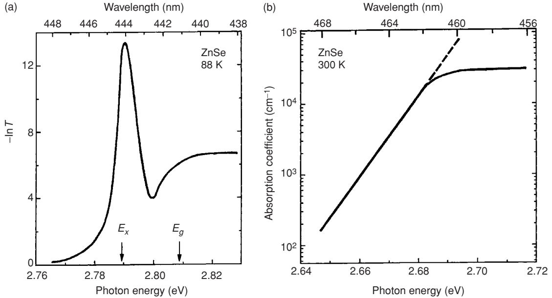
Fig. 4.9 Absorption spectrum of a ZnSe single crystal near the fundamental absorption edge at a temperature equal to 88 K (a) and 300 K (b) [18]. In panel (a) -\ln T = -\ln(I_{\text{out}}/I_{\text{in}}) where T is the optical transmission coefficient, I_{\text{out}}(I_{\text{in}}) is output (input) light intensity.
