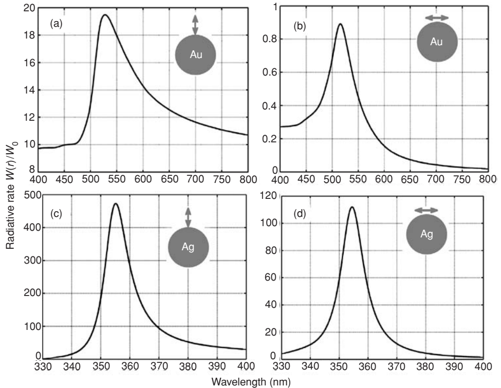
Fig. 16.4 Radiative rate enhancement of a probe dipole near a spherical nanoparticle of (a) and (b) gold and (c) and (d) silver. Dipole orientation is shown by the arrows. Adapted from [5].
