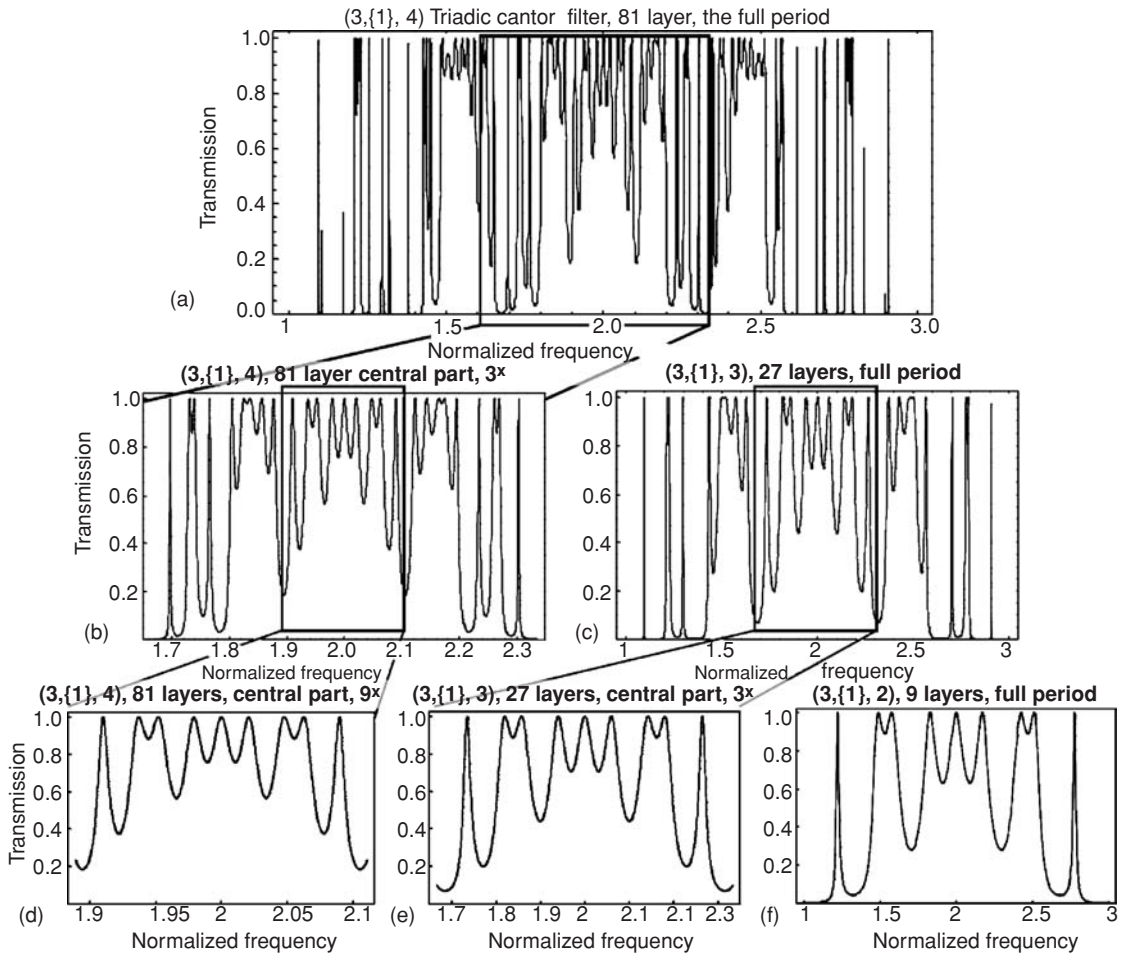
Fig. 8.12 Scalability of optical spectra for triadic Cantor filters (3, \{1\}, N) : (a) the full period for N = 4 ; (b) the central part magnified in the frequency scale by 3 versus (c) the full period for N = 3 ; (d) the central part for N = 4 magnified by 9 = 3^2 ; (e) the central part for N = 3 magnified by 3; (f) the full period for N = 2 . Compare patterns in (b) versus (c) and in (d) versus (e) and (f). All resonance peaks in transmission have the maximal value of unity. Somewhat lower values apparent for a few peaks in (a) are artifacts due to high finesse of resonances and finite-step numerical calculations, as well as finite spatial resolution of the used software and hardware. Adapted from [28].
