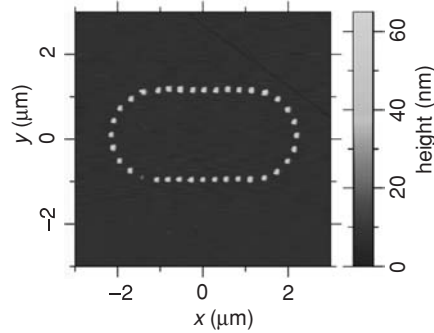
Fig. 14.9 Topographical image obtained by atomic force microscopy of a corral formed by nanometer sized gold pillars [50].
