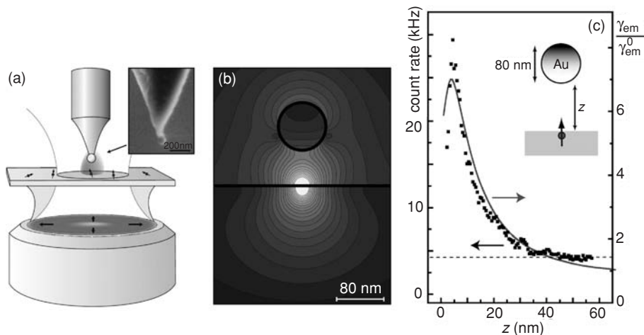
Fig. 16.11 Distance-dependent spontaneous emission rate of a single molecule in the presence of a gold spherical nanoparticle [40]. (a) Sketch of the experimental arrangement. Inset: SEM image of a gold particle attached to the end of a pointed optical fiber. (b) Field distribution |E|^2 (factor of 2 between successive contour lines) of an emitting dipole (wavelength is 650 nm) located 2 nm beneath the surface of a glass substrate and faced by a gold particle separated by a distance of z = 60 nm from the glass surface. (c) Fluorescence rate as a function of particle–surface distance z for a vertically oriented molecule (solid curve: theory, dots: experiment). The horizontal dashed line indicates the background level.
