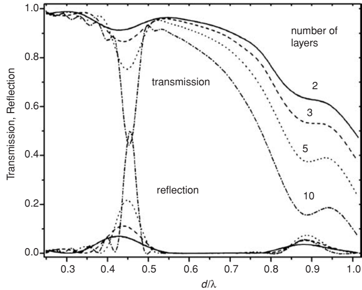
Fig. 7.14 Optical transmission and reflection spectra for a set of sequential layers consisting of close-packed spherical particles with cubic symmetry as a function of a dimensionless parameter d/\lambda , where d is the sphere diameter and \lambda is the wavelength in a vacuum. Numbers on the curves indicate the number of layers. Refractive index of spherical particles versus voids is 1.26. Adapted from [30].
