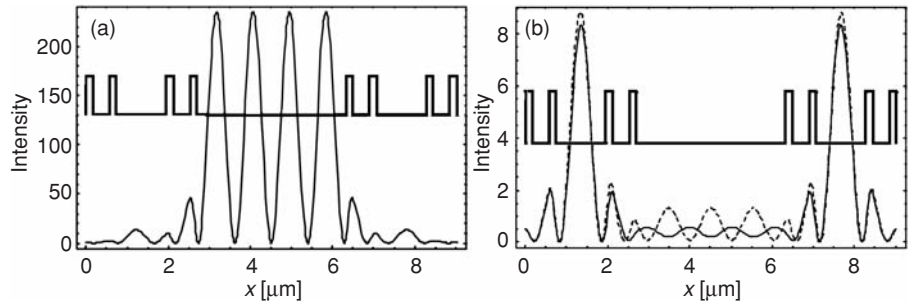
Fig. 8.18 Electric field profiles superimposed with the refraction index profile for a third-order Cantor filter [28]. (a) Normalized frequency is 0.705; (b) normalized frequency is 0.775 and 0.785.
