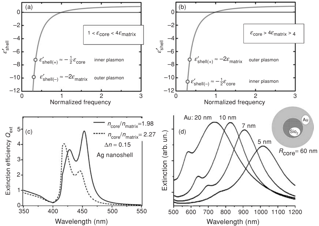
Fig. 6.16 Optical properties of spherical nanoparticles with a dielectric core and a metal shell. (a), (b) The real part of the dielectric function of an ideal metal and the relative positions of the inner and outer surface plasmon resonances, according to the solutions of Eq. (6.93), the normalized frequency is \omega/\omega_p . (c) Extinction spectra calculated for the two combinations of refractive indices of core and matrix corresponding to the different mutual positions of the inner and outer resonances for silver nanoshells [36]. Core radius is 10 nm, silver shell thickness is 7.9 nm. (d) Calculated extinction spectra of a number of core-shell silica/gold particles in air with core radius 60 nm and varying shell thickness between 5 to 20 nm (indicated near every curve). Adapted from. Reprinted with permission from [39]. Copyright 1998, Elsevier B.V.
