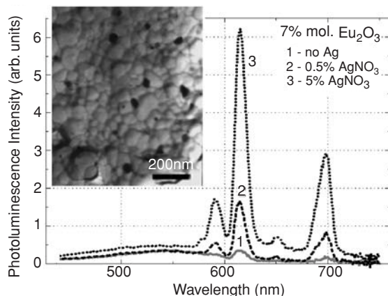
Fig. 16.9 Photoluminescence spectra of \text{Eu}^{3+} ions in sol-gel films containing silver nanoparticles. Successive growth of Ag salt content gives rise to a considerable increase in photoluminescence intensity correlating with formation of silver nanoparticles. These are seen in the inset as dark spots. Adapted from [30].
