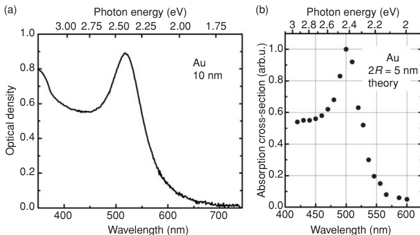
Fig. 6.11 (a) Measured optical density spectrum of sol of Au nanoparticles imaged in Figure 6.8 in a liquid solution and (b) the absorption cross-section calculated by Kreibig and Vollmer [1].
