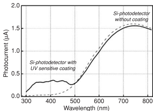
Fig. 5.39 The spectral sensitivity of a silicon commercial photodiode as made (dashed line) and enhanced by a CdS:Mn nanocrystalline spectral transformer (solid line).
