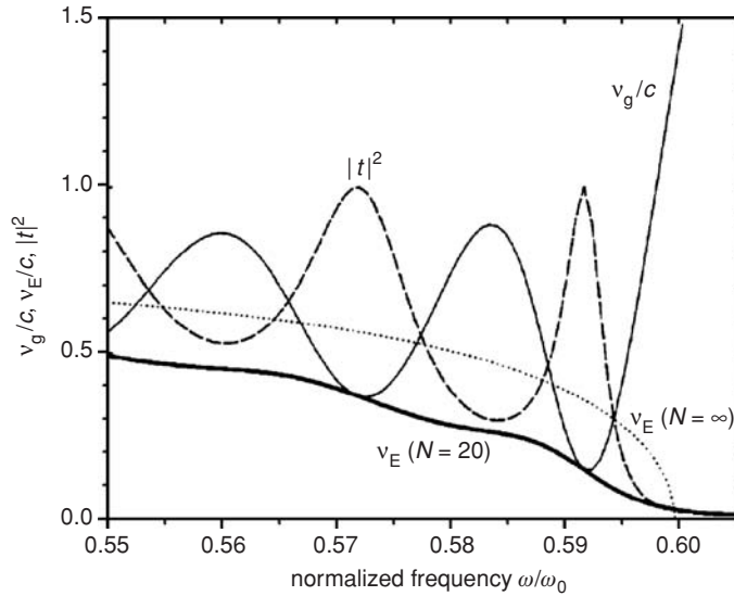
Fig. 7.32 Normalized group velocity ( v_g/c ), energy velocity ( v_E/c ), and transmittance ( |t(\omega)|^2 ) for a 20-period slab along with the energy velocity of the relevant infinite periodic medium [78]. See text for detail.
