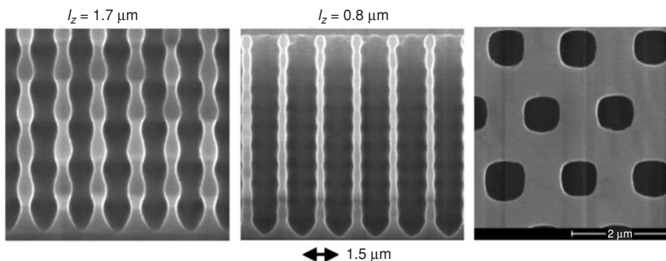
Fig. 7.21 Three-dimensional periodicity in electrochemically derived silicon structures using surface pre patterning and etching current alteration [59].
