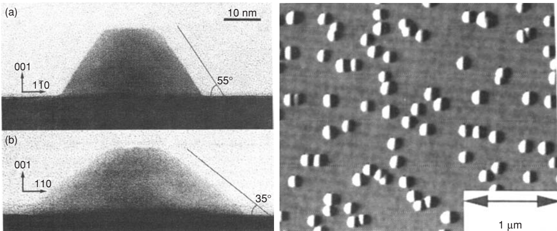
Fig. 5.13 InP nanocrystals on a GaInP substrate: high-resolution transmission electron microscope image of a single nanocrystal for two cross-sections (left) [46], atomic force microscope image on a larger scale (right) [47]. Copyright 1995 AIP[46]. Copyright 1995 Elsevier Science B.V. [47].
