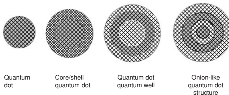
Fig. 5.11 Nanoengineering options offered by “inorganics-in-organics” chemistry: nanocrystals capped with organic groups (quantum dots), binary core/shell quantum dot structures, ternary quantum dot/quantum well structures, and onion-like multilayer composite systems. Darker circles and layers are active components whereas lighter circles and layers are wider-band-gap materials constituting potential barriers. Lines show, approximately, the atomic planes.
