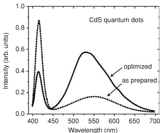
Fig. 5.45 White light emission spectrum from CdS quantum dots. The dashed line shows the original spectrum, the solid line shows the optimized spectrum by means of plasmon-assisted enhancement of the long-wave band using silver nanoparticles. Adapted from [113].
