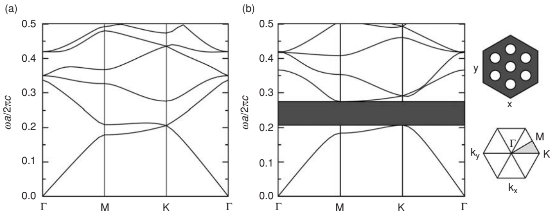
Fig. 7.11 Photonic band structure for (a) E -polarized and (b) H -polarized light in a 2D photonic crystal created by a triangular lattice of air holes ( \varepsilon = 1 ) with the radius r = 0.3a (where a is the lattice period) in a dielectric with permittivity \varepsilon = 12 ; the band gap is darkened. The top right inset shows a cross-sectional view of a fragment of the 2D photonic crystal. The bottom right inset shows the corresponding Brillouin zone, with the irreducible zone shaded. Reprinted with permission from [12]. Copyright 2007, Elsevier B.V.
