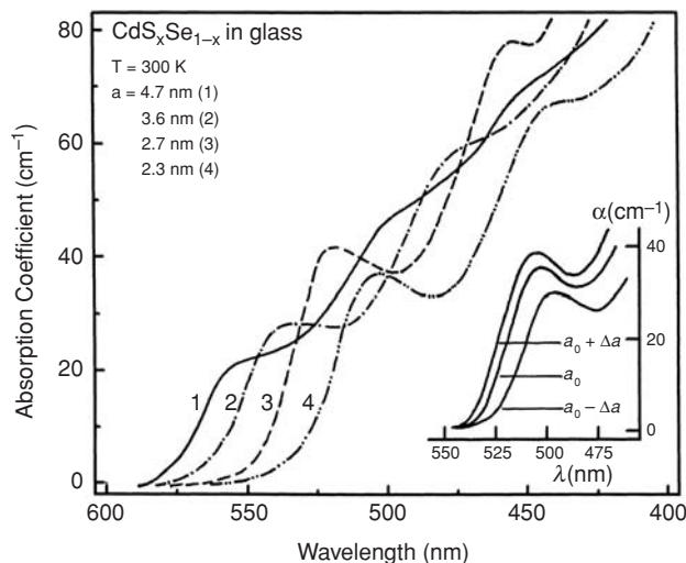
Fig. 5.10 Absorption spectra of \text{CdS}_x\text{Se}_{1-x} nanocrystals in a glass matrix at room temperature [35]. Insert shows absorption spectra for small deviations of mean size around \bar{a}_0 = 2.3 nm. The spectra show a clear blue shift with decreasing mean radius \bar{a} due to the quantum confinement effect. The absolute values of the shift is one order of magnitude larger than the exciton Rydberg energy which is indicative of the strong confinement regime. For smaller \bar{a} values the shift of the first band with growing \bar{a} systematically results in an increase in the total absorption (see data for \bar{a} = 2.3, 2.7 and the insert) which is indicative of the normal growth stage. At this stage, mean size growth occurs due to increase in the total volume of the semiconductor phase in the matrix. Therefore, absorption spectra at this stage do not overlap.
