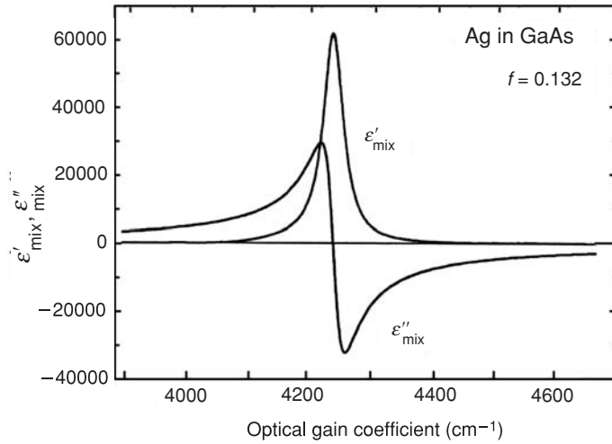
Fig. 11.9 Real ( \epsilon'_{\text{mix}} ) and imaginary ( \epsilon''_{\text{mix}} ) parts of the dielectric function for GaAs gain medium ( n = 3.6 ) with silver nanoparticles (adapted from [30]). Metal volume fraction is f = 0.132 , wavelength \lambda = 800 nm.
