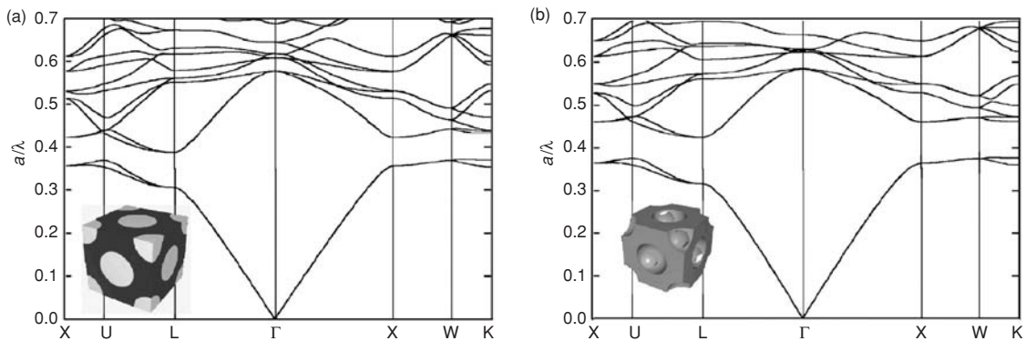
Fig. 7.13 Photonic band diagrams of (a) a silicon/silica composite diamond structure and (b) structure made of air spheres in silicon resulting from the removal of the silica spheres from the former. The filling fraction for silicon is 50%. The insets show the corresponding real space structures. Reprinted with permission from [28]. Copyright 2001 AIP.
