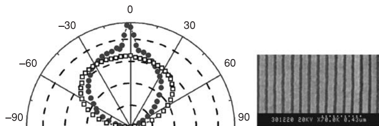
Fig. 14.11 Luminescence indicatrices of \text{Eu}^{3+} ions in titania xerogel embedded in a nanoporous alumina slab (black circles) and on a silicon surface (squares). Right-hand panel shows a portion of cross-section of the nanoporous alumina slab. Adapted from [61].
