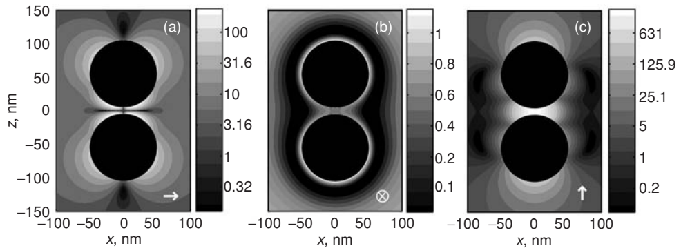
Fig. 16.5 Mapping of spontaneous decay rates of an atomic dipole placed near a pair of silver spherical nanoparticles [6]. Radiative decay rate is normalized with respect to radiative rate in a vacuum. Nanoparticle diameter is 100 nm. Dipole momentum orientation is shown by the arrows and corresponds to (a) x , (b) y , and (c) z axes.
