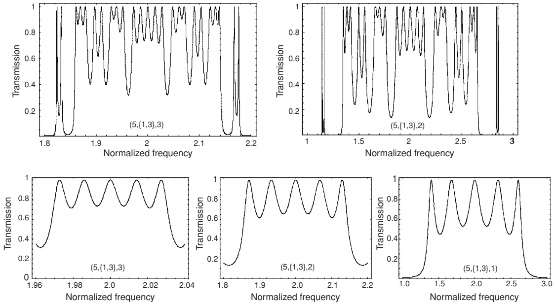
Fig. 8.13 Spectral scalability of Cantor pentadic filters. Top row: G = 5 -fold stretched central part of the 3rd generation is compared with the full spectrum of the 2nd generation. Bottom row: G^2 = 5^2 = 25 -fold stretched central part of the 3rd generation is compared with the five-fold extended central part of the 2nd generation and with the full period of the 1st generation [28].
