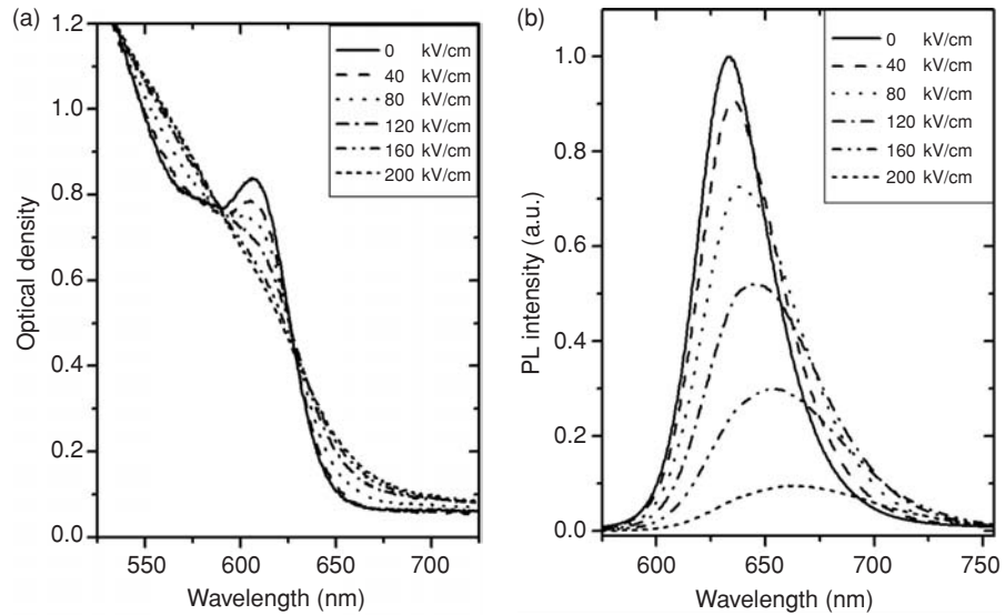
Fig. 5.50 Electric field effect on (a) optical absorption and (b) emission spectra of CdSe nanocrystals in a polymer film [124]. The mean radius of nanocrystals is 2 nm, temperature is 300 K.
