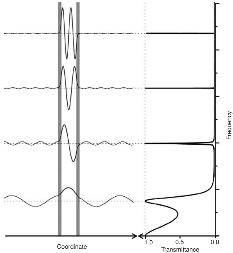
Fig. 3.19 Accurate numerical solutions for the electric field amplitude (left) and transmission spectrum (right) of a Fabry-Perot resonator consisting of two metal films with thickness d_2 , refraction index i\chi_2 , separated by a dielectric spacer of thickness d_0 and refraction index n_0 , coinciding with that of the ambient environment. Parameters used in calculations are, d_0 = 200 nm, n_0 = 1 , d_2 = 40 nm, \chi_2 = 2 [18].
