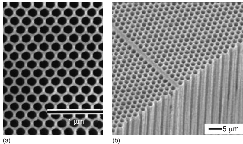
Fig. 7.17 Two-dimensional periodic structures developed by means of lithographical pre patterning and anodization. (a) SEM micrograph of regular pore configuration in an alumina layer with intervals of 200 nm, the film thickness is approximately 3 \mu\text{m} [47]. (b) Electron micrograph of a two-dimensional hexagonal porous silicon structure with a lattice constant a = 1.5 \mu\text{m} and a pore radius r = 0.68 \mu\text{m} , fabricated by anodization of p-type silicon [48]. Copyright 1997 AIP [47]. Copyright 2007 Elsevier B.V. [48].
