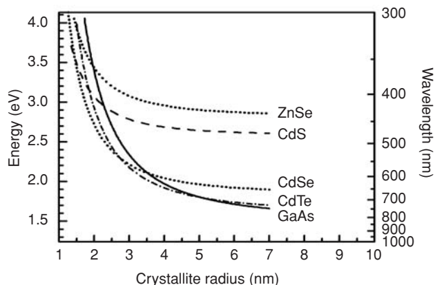
Fig. 5.7 Size-dependent photon energy and light wavelength of the first absorption resonance for nanocrystals of various semiconductor materials (ZnSe, CdS, CdSe, CdTe, GaAs) calculated using Eq. (5.11).
