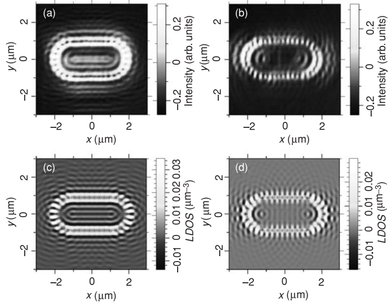
Fig. 14.10 SNOM images of a corral taken for (a) dipole orientation along x -axis, and (b) dipole orientation along y -axis. polarizations: (c), (d) the relevant calculated local DOS distribution at the height of z = 120 nm over the surface [50].
