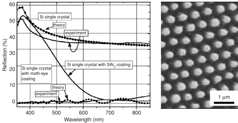
Fig. 7.28 Effect of moth-eye surface relief on reflection at the Si/air interface. Left: reflection spectra of various structures. Right: Scanning electron microscope image of moth-eye silicon antireflection coating. Adapted with permission from [69]. Copyright 2008 AIP.
