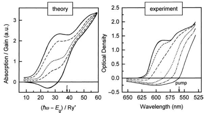
Fig. 5.35 Calculated (left) and observed (right) absorption spectra of CdSe nanocrystals [95]. Upper curves in each panel are the linear absorption spectra. The other curves correspond to successively growing (theory) population and (experiment) excitation intensity, from top to bottom. The mean nanocrystal radius is \bar{a} = 2.5 nm, the Gaussian size distribution in calculation was given to be \Delta a = 0.1\bar{a} .
