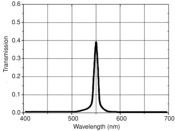
Fig. 3.20 Experimentally observed resonant transmission spectrum for a commercial Fabry-Perot interferometer with metal mirrors. Maximal transmission is noticeably less than 1 because of losses in the metal films.
