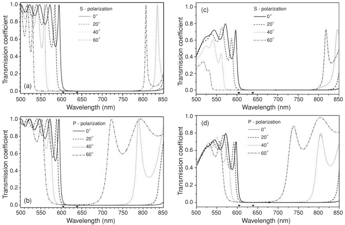
Fig. 7.25 Omnidirectional reflection in a periodic multilayer structure. (a), (b) Calculated and (c), (d) measured transmission spectra of a \text{Na}_3\text{AlF}_6/\text{ZnSe} 19-layer structure for (a), (c) s -polarized (TE-mode) and (b), (d) p -polarized (TM-mode) light at different angles of incidence ( 0^\circ -solid line, 20^\circ -dashed line, 40^\circ -dotted line, 60^\circ -dash-dotted line). The lower triangles indicate the edges of the calculated absolute omnidirectional band gap [19].
