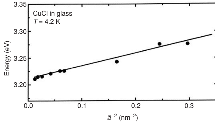
Fig. 5.4 The size dependence of the Z_3 -exciton band for CuCl nanocrystals in a glass matrix [8, 22]. The dots are experimental data, the curve corresponds to Eq. (5.5) with an additional coefficient for the third term accounting for the size distribution function.
