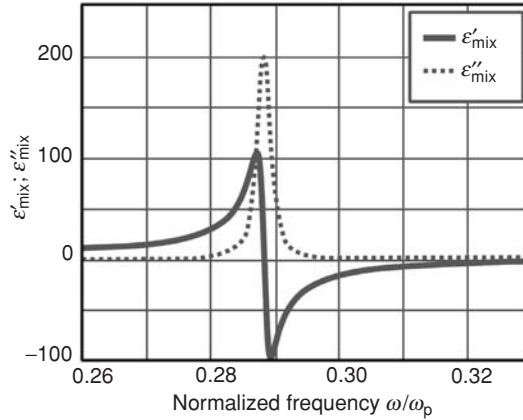
Fig. 6.10 The real (solid line) and the imaginary (dots) parts of the complex dielectric function of a composite medium consisting of Ag nanoparticles dispersed in a medium with \varepsilon = 2.56 with volume fraction f = 0.2 [26]. The silver dielectric function obeys Eq. (6.30) with parameters \varepsilon_\infty = 5 , \hbar\omega_p \approx 9 eV, \hbar\Gamma = 0.02 eV.
