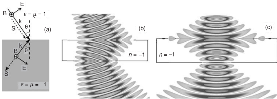
Fig. 11.13 Propagation of electromagnetic waves impinging a slab of negative refractive index material from air. (a) Negative refraction at a matched interface; (b) calculated Gaussian beam propagation for oblique incidence [38]; (c) calculated Gaussian beam propagation at normal incidence with focusing effect [38].
