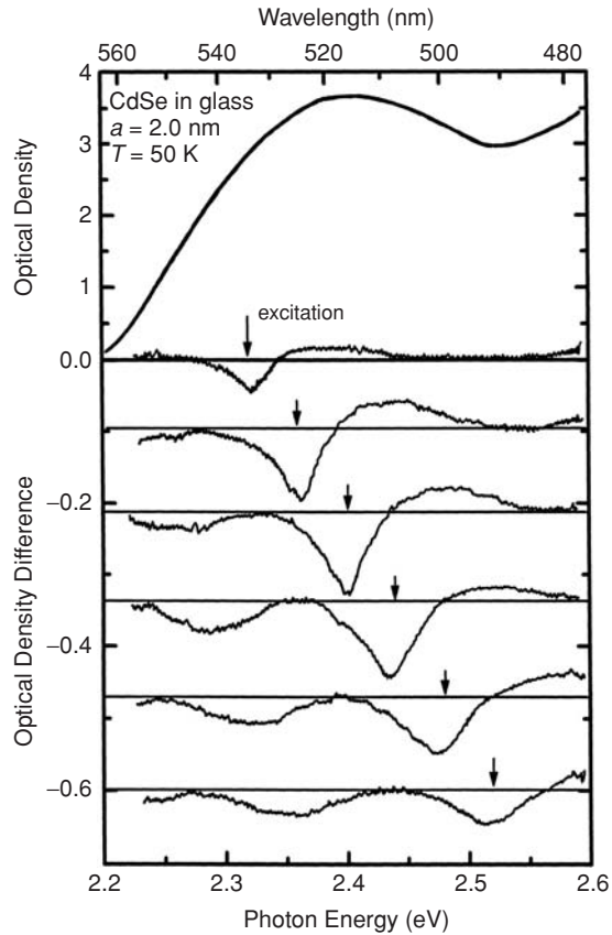
Fig. 5.16 Doublet structure of the first absorption feature of CdSe nanocrystals in glass elucidated by means of a nonlinear pump-and-probe technique [8, 49]. Mean crystallite radius is 2.0 nm, temperature is 50 K. The upper panel presents the linear absorption spectrum. The lower panel presents differential absorption spectra recorded under monochromatic excitation by a tuneable laser (pulse duration is 5 ns, intensity is 100 \text{ kW/cm}^2 ) with simultaneous read-out by a weak broad-band probe beam. Negative differential optical density corresponds to bleaching.
