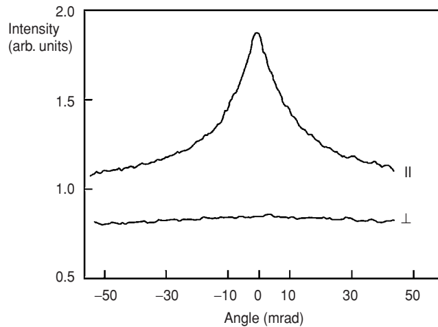
Fig. 8.5 The backscattering peak for a reflective filter composed of randomly-oriented \text{BaSO}_4 microparticles typically used as a white reflectance etalon [8]. The analyzing polarizer is oriented either parallel ( \parallel ) or perpendicular ( \perp ) to the incident laser radiation polarization.
