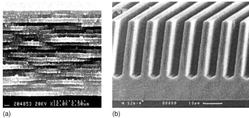
Fig. 7.16 Periodic structures with one-dimensional periodicity. (a) A multilayer dielectric mirror, period is about 500 nm [45]. (b) A silicon comb developed by means of templated etching. The period is about 10 \mu\text{m} [46].
