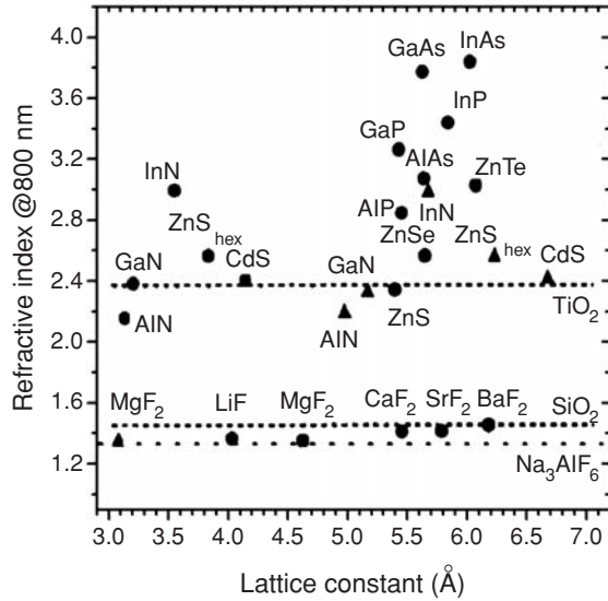
Fig. 7.24 Refractive index versus lattice constant for a number of crystals (dots and triangles) along with refractive index for optical polycrystalline films \text{TiO}_2 , \text{SiO}_2 , and \text{Na}_3\text{AlF}_6 (dashed lines). All data are taken from [65] except \text{Na}_3\text{AlF}_6 [19]. Copyright 2000 AIP.
