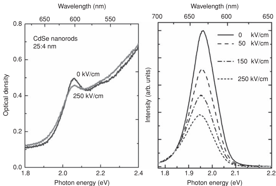
Fig. 4.20 Optical properties of CdSe nanorods with length 25 nm and diameter 4 nm in a polymer matrix. Left: Absorption spectrum with and without an external electric field applied. Right: Photoluminescence emission spectra of nanorods for various applied voltages.
