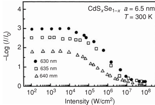
Fig. 5.30 Absorption saturation in commercial glasses doped with CdS x Se 1-x nanocrystals at the room temperature measured with nanosecond laser pulses [85]. I_0 is the incident intensity, I is the transmitted power density.
