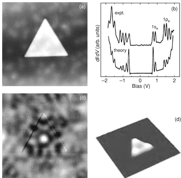
Fig. 5.22 Imaging electron local density of states in an InAs quantum dot by means of scanning tunneling spectroscopy [67, 68]. (a) a scanning tunneling microscope image of a triangular InAs quantum dot, image size is 93.8 \text{ nm} \times 93.8 \text{ nm} ; (b) measured and calculated differential conductance dI/dV ; (c) dI/dV mapping for bias voltage V = 0.08 \text{ V} ; (d) calculated local density of electron state for the lowest state of an InAs quantum dot.
