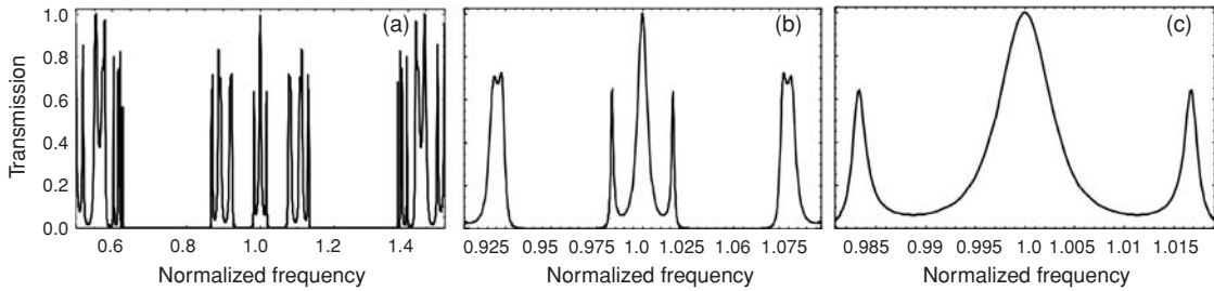
Fig. 8.22 Apparent self-similarity of transmission spectra for a Fibonacci filter [31]. (a)–(c) show the central portions of the transmission spectrum for the 10th generation filter with (b) single and (c) double 5.11-fold stretching of the frequency axis. Note a self-similar ternary pattern of the spectrum at different scales.
