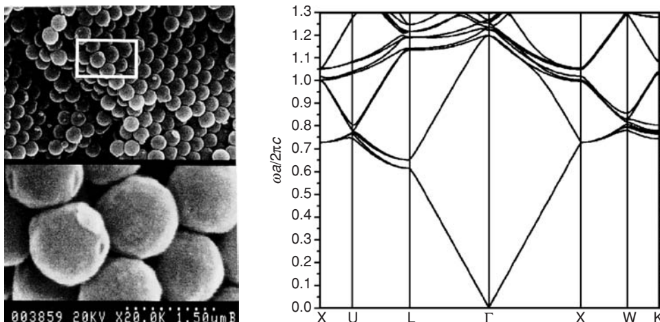
Fig. 7.22 Opal-based periodic structures. Left: Scanning electron microscopy image of a synthesized silica colloidal crystal. Lower panel shows the magnified image of a portion of the crystal inside a white frame [61]. Globule diameter is 250 nm. Right: Photonic band structure diagram according to calculations by Reynolds et al. [63].
