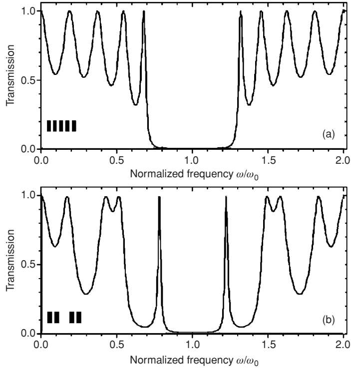
Fig. 8.11 Transmission spectra of (a) a nine-layer periodic quarter-wave stack and (b) a nine-layer Cantor triadic filter. The structures are shown in the left bottom corners of each graph. Adapted from [28].
