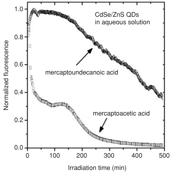
Fig. 5.48 Photoluminescence intensity of CdSe/ZnS core-shell quantum dots in aqueous solution with mercaptoundecanoic and mercaptoacetic acids for prolonged excitation by a cw Nd:YAG laser ( 5 \text{ mW/mm}^2 at 530 \text{ nm} ) [122].
