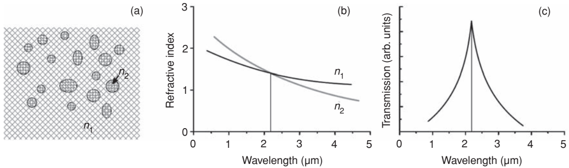
Fig. 8.31 Christiansen's filters: (a) a dielectric powder in an ambient medium with different refraction properties, (b) refraction spectra of two media, (c) transmission spectrum of a slab featuring a maximum at the wavelength where n_1 = n_2 .
