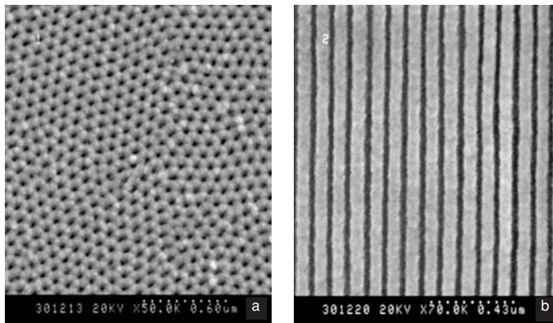
Fig. 7.18 SEM micrographs of (a) top and (b) cross-sectional views for the representative sample of nanoporous alumina developed by means of self-organisation without prepatterning [51]. The pore diameter is approximately 30 nm.
