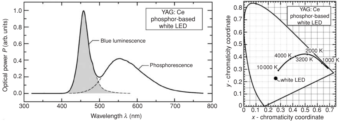
Fig. 5.43 Emission spectrum of a commercial white diode manufactured by Nichia corporation (left) and position of its spectrum on the chromaticity diagram along with the line indicating the black body spectrum with indicated temperatures (right) [111].
