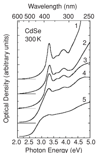
Fig. 5.27 A set of absorption spectra of CdSe nanoparticles, average radius is 1.6 nm. Nanoparticle concentration progressively rises from upper to lower curves. Curve 5 corresponds to a CdSe film consisting of close-packed clusters capped with organic groups, curves 1–4 correspond to cluster/polymer composition, polymer volume fraction being 37%, 18%, 3%, 1%, respectively. Adapted from [77].
