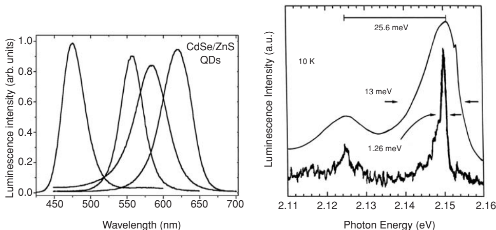
Fig. 5.20 Photoluminescence of CdSe colloidal quantum dots in the strong confinement regime. Left panel: a set of emission spectra for a quantum dot ensemble with different mean sizes at room temperature under excitation by near UV light [55]. Right panel: Low-temperature luminescence data collected under conditions of ensemble-averaged red-edge excitation (upper curve) and single dot excitation (lower curve) [59]. The bar of 25.6 meV indicates the longitudinal optical phonon energy.
