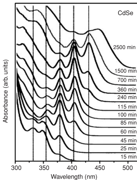
Fig. 5.18 Sequential (from bottom to top) absorption spectra of CdSe colloidal nanocrystallites observed in the course of their growth in a solution. Numbers indicate growth time in minutes for every spectrum. Reproduced with permission from [51]. Copyright Wiley-VCH.
