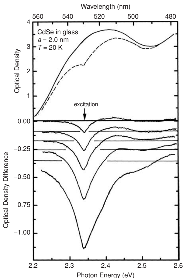
Fig. 5.15 Spectral hole-burning due to selective absorption saturation in an ensemble of CdSe nanocrystals in a glass matrix [8, 48]. Mean nanocrystal radius is 2.0 nm, temperature is 20 K. The upper panel shows the absorption spectrum of the unexcited sample (solid line) and the spectrum recorded under excitation by a laser pulse (photon energy 2.34 eV, duration is 5 ns, intensity is 7 \text{ MW}/\text{cm}^2 , dashed line). The lower panel shows differential absorption spectra for successively growing excitation intensity from 90 \text{ kW}/\text{cm}^2 to 7 \text{ MW}/\text{cm}^2 . Negative change in optical density corresponds to bleaching.
