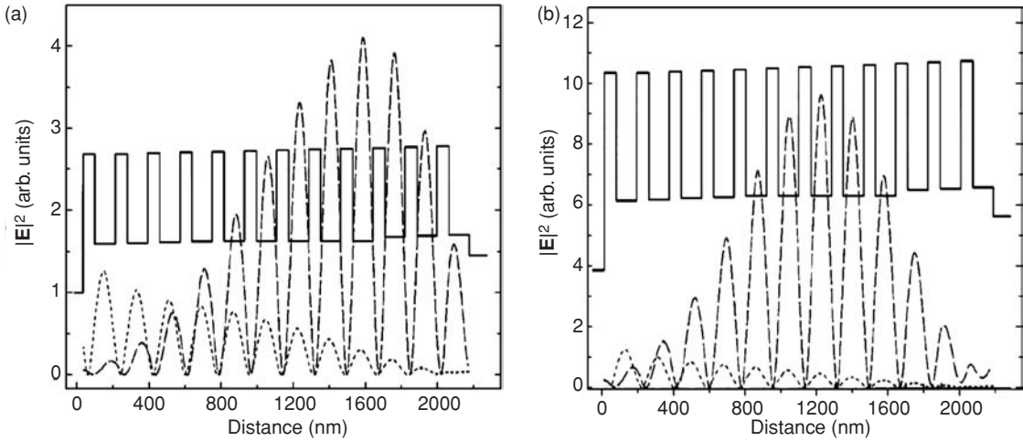
Fig. 7.34 |E|^2 profile, normalized to an incident vacuum value of |E|^2 = 1 , inside the index ramp structure for (a) very low incident intensity (linear case) and (b) high incident intensity. The dotted line represents light incident from the left, and the dashed line represents light incident from the right. The index profile of the structure is plotted (solid line) for reference. The light wavelength is (a) 640 nm and (b) 641 nm and corresponds to the long-wave edge of the transmission band. Reprinted with permission from [82]. Copyright 1995 AIP.
