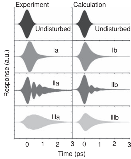
Fig. 8.25 Experimental data and calculation of the transmission through a Fibonacci filter at four different frequencies [43]. The reference pulse is also plotted for comparison. The time offset corresponding to the total optical thickness of the sample has been subtracted in all cases. When the laser pulse is resonant with one band-edge state the transmitted intensity is strongly delayed and stretched. When two band-edge states are excited, mode beating is observed.
