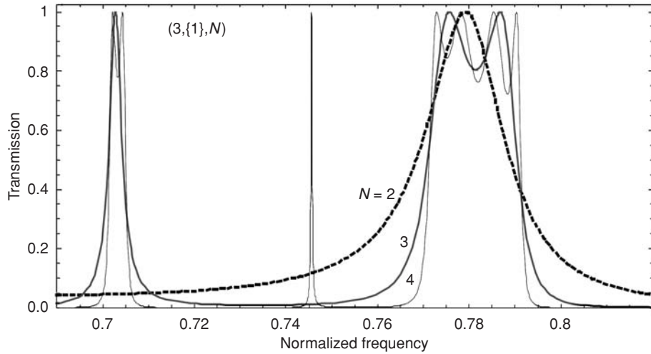
Fig. 8.17 A portion of the frequency scale with transmission bands of triadic Cantor filters of second, third and fourth generations [28].
