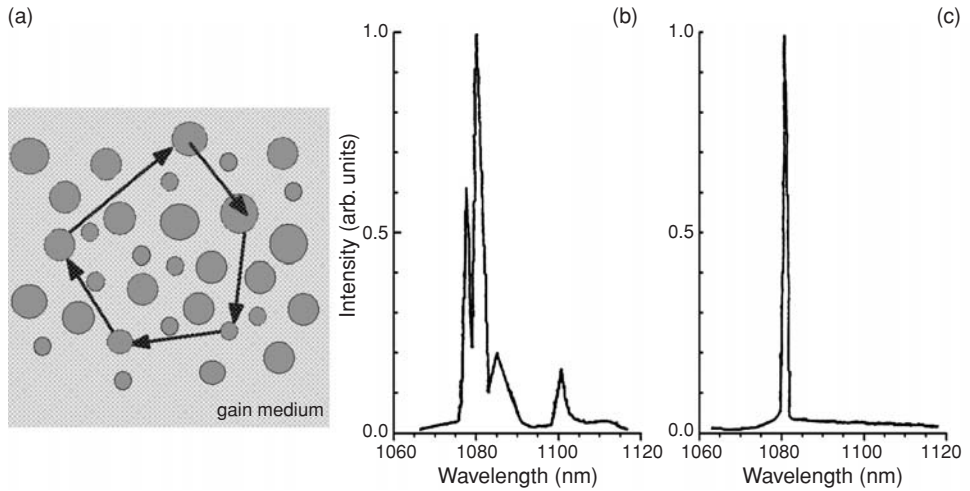
Fig. 8.32 A Letokhov's laser: (a) the general idea, (b) emission spectrum of \text{Nd}^{3+} -containing powder below the threshold, and (c) above-threshold pumping [66].
