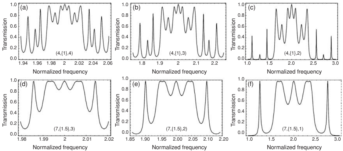
Fig. 8.14 Spectral scalability of non-Cantor fractal structures [31]. (a)–(c) show spectra for three different generations of the asymmetric structure (4, \{1\}, N) . (c) presents the full spectrum whereas (a) and (b) represent the central portions with (a) G^2 = 4^2 = 16 -fold stretching and (b) G^1 = 4 -fold stretching with respect to (c). (d)–(f) show spectra for three different generations of the symmetric (7, \{1, 5\}, N) fractal structure. (f) presents the full spectrum whereas (d) and (e) represent the central portions with (d) G^2 = 7^2 = 49 -fold stretching and (e) G^1 = 7 -fold stretching with respect to (f).
