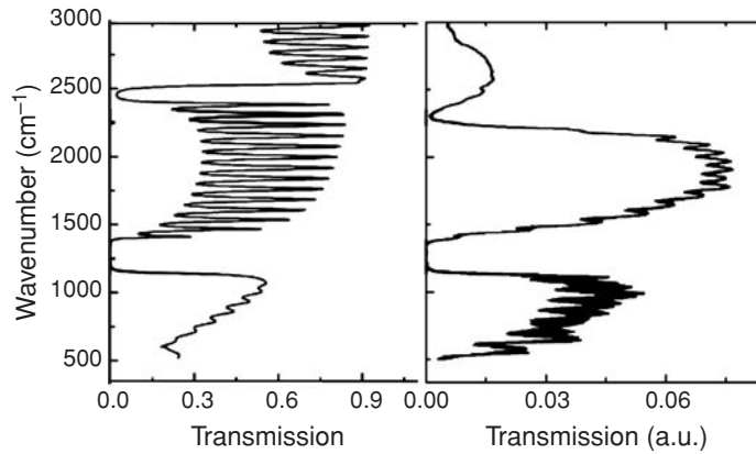
Fig. 7.30 Calculated (left panel) and measured (right panel) transmission spectra of a three-dimensional periodic silicon photonic crystal slab. Adapted from [59]. Transmission is calculated and measured along pore axis for a structure with a = 1.5 \mu\text{m} , l_z = 2 \mu\text{m} , whose image was presented in Figure 7.21.
