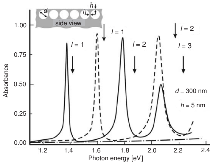
Fig. 11.16 Absorption spectra of light incident normally onto a silver surface with spherical inclusions of a material with dielectric constant \varepsilon = 4.5 (solid curve) and \varepsilon = 3.3 (dashed curve) [46]. The absorption of light on the surface of bulk silver is shown by dash-dotted curve. Vertical arrows mark the energies of the fundamental ( l = 1 ), second ( l = 2 ) and third ( l = 3 ) plasmon modes of a single void in bulk silver.
