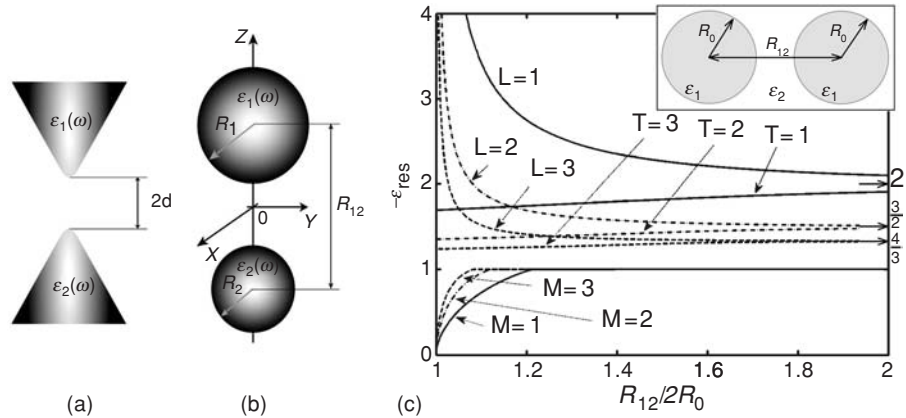
Fig. 6.15 Plasmonic molecules. (a), (b) possible designs [23]; (c) resonances of dielectric function for a pair of two identical metal spherical particles (adapted from [37]).
