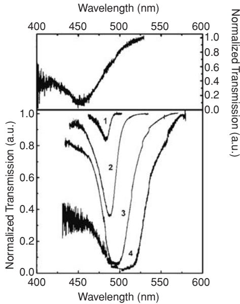
Fig. 7.31 Optical transmission spectra of an artificial opal sample with (upper panel) empty voids and (lower panel) impregnated with various fillers: (1) methanol ( n = 1.328 ), (2) ethanol ( n = 1.361 ), (3) cyclohexane ( n = 1.426 ) and (4) toluene ( n = 1.497 ) [30].
