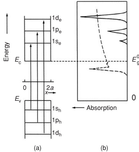
Fig. 5.5 The optical properties of an ideal spherical quantum dot with isotropic scalar effective masses of a non-interacting electron and hole. (a) A sketch of electron-hole energy levels, optical transitions and (b) reduction of original bulk absorption spectrum (dashed curve) to discrete bands (solid curves).
