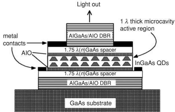
Fig. 5.37 Design of a vertically emitting microcavity laser with vertically coupled InGaAs quantum dots reported by Ledentsov et al. [105]. DBR stands for Distributed Bragg Reflector.
