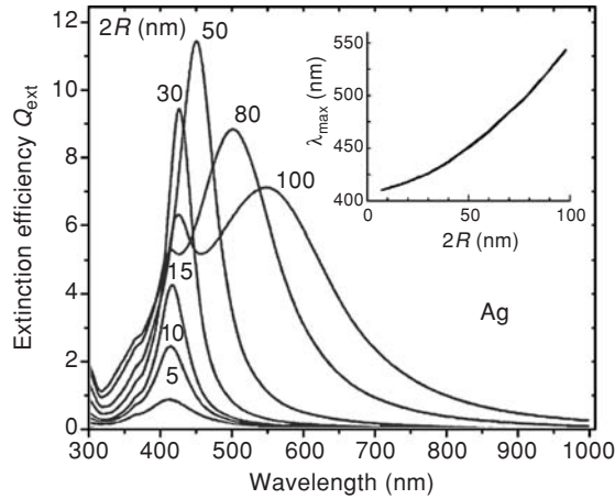
Fig. 6.14 Extinction efficiency for identical silver particles dispersed in a medium with refractive index 1,5 for various diameters indicated near every curve (adapted from [36]). The insert shows absorption peak wavelength dependence on particle diameter.
