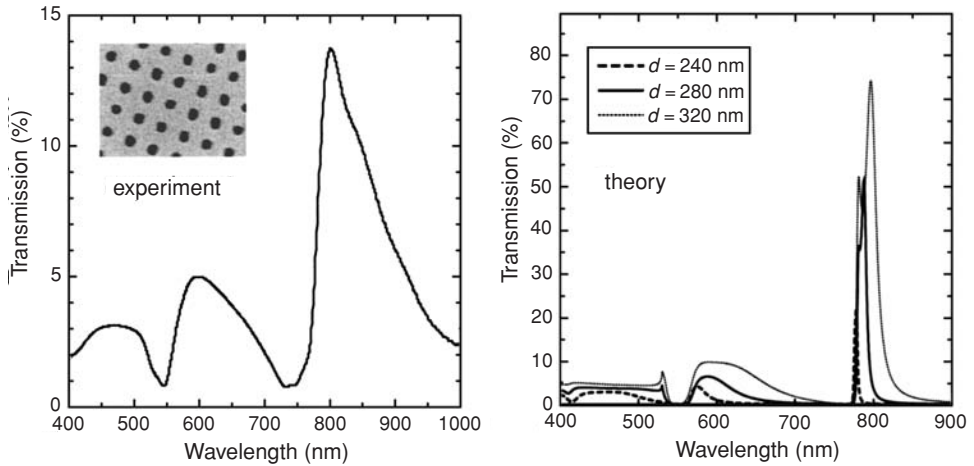
Fig. 11.7 (Left) Experimental power transmittance at normal incidence for a square array of holes (lattice constant is 750 nm, average hole diameter is 280 nm) in a freestanding Ag film (thickness is 320 nm). Inset: electron micrograph of the perforated metal film. (Right) Calculated transmittance at normal incidence for an array of holes in a Ag film, defined by the lattice constant 750 nm, thickness 320 nm and three different hole diameters d indicated in the inset. Adapted from [24].
