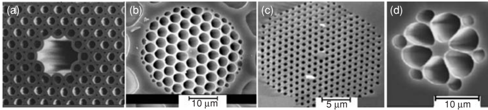
Fig. 9.7 Various design of PC-fibers: (a) fiber with hollow core [29], and (b)–(d) fibers with solid cores and holey structures used for generation of white light, short-pulse compression, non-linear-optical interactions enhancement [30, 31].
