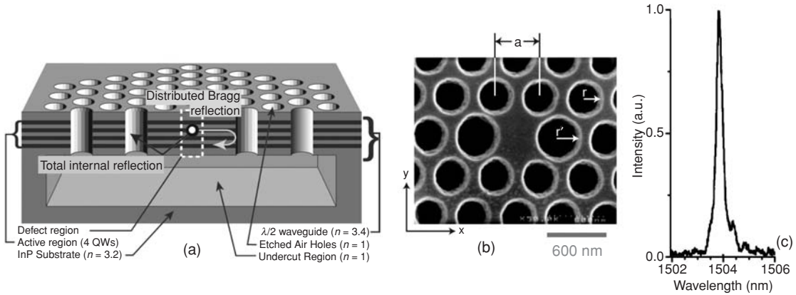
Fig. 9.2 A microcavity photonic crystal laser: (a) design, (b) implementation and (c) performance. Semiconductor material is InGaAsP. Triangular lattice period a = 515 nm, pore radius r = 180 nm. The two enlarged holes have a radius r' = 240 nm. These are designed to split the dipole mode degeneracy. The InGaAsP membrane is 220 nm (half-wavelength) in thickness. Adapted from [3]. Reprinted with permission from AAAS.
