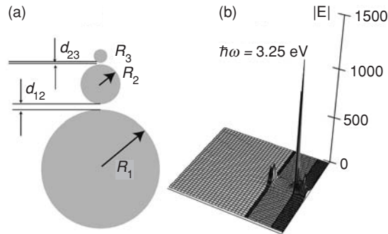
Fig. 11.3 Local field enhancement in a self-similar chain of metal nanoparticles. (a) Geometry of a nanolens consisting of three silver nanospheres is shown in cross-section through its plane of symmetry. Nanosphere radii are: R_1 = 45 nm, R_2 = 15 nm and R_3 = 5 nm. The separations between the nanosphere surfaces are d_{12} = 4.5 nm and d_{23} = 1.5 nm. (b) Local electric field enhancement coefficient as a function of the position in the cross-section through the plane of symmetry. Adapted from [13].
