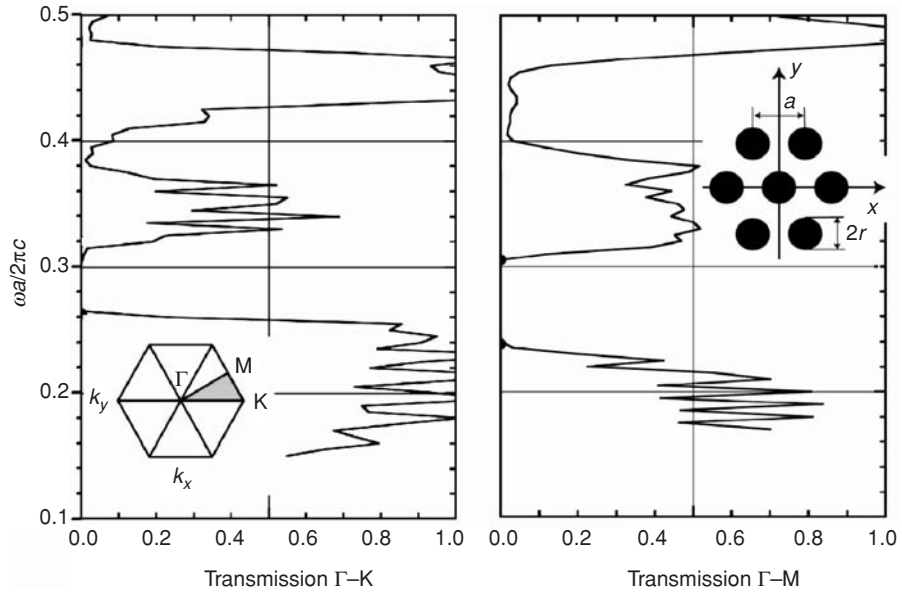
Fig. 7.26 Transmission spectra of a 10-period slab of a two-dimensional photonic crystal with triangular lattice of silicon rods. Left-hand part corresponds to the \Gamma -K direction of the wave vector, right-hand part corresponds to the \Gamma -M direction. The inset on the left shows the first Brillouin zone in k -space with the irreducible zone shaded. The inset on the right shows a portion of the lattice in space. Adapted from [66].
