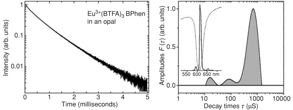
Fig. 14.6 Luminescence decay of \text{Eu}^{3+} ions in \text{Eu}^{3+}(\text{BTFA})_3\text{-BPhen} complexes embedded in an opal by means of sol-gel reactions (left) and the elucidated decay time distribution (right). The insert shows the \text{Eu}^{3+} emission spectrum (solid line) superimposed with the reflection spectrum of an opal at normal incidence (dots). Adapted from [24, 26].
