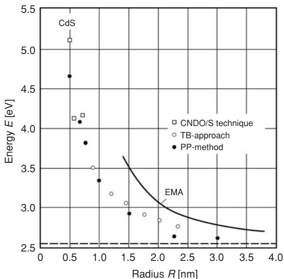
Fig. 5.8 Calculated energy of the first allowed optical transition versus crystallite radius for CdS clusters/dots [8,12]. (□) CNDO/S-technique; (○) tight-binding approach; (●) pseudopotential method; solid line – particle-in-a-box model (Eq. (5.11)). The dashed line shows the energy of the first exciton resonance in the bulk crystal.
