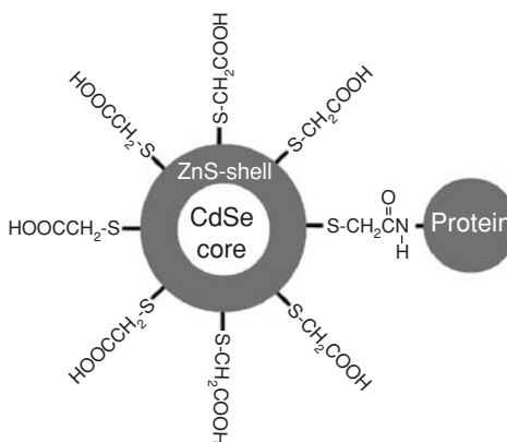
Fig. 5.46 A CdSe/ZnS core-shell quantum dot linked to a protein molecule via organic groups as proposed by Chan and Nie [118].
