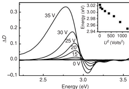
Fig. 5.49 Change in optical density of a 200 nm PMMA film containing 1.8 nm diameter CdSe nanocrystals at applied external voltage U from 0 to 35 V [79]. Positive change in optical density corresponds to decrease in transmission. Temperature is 300 K.
