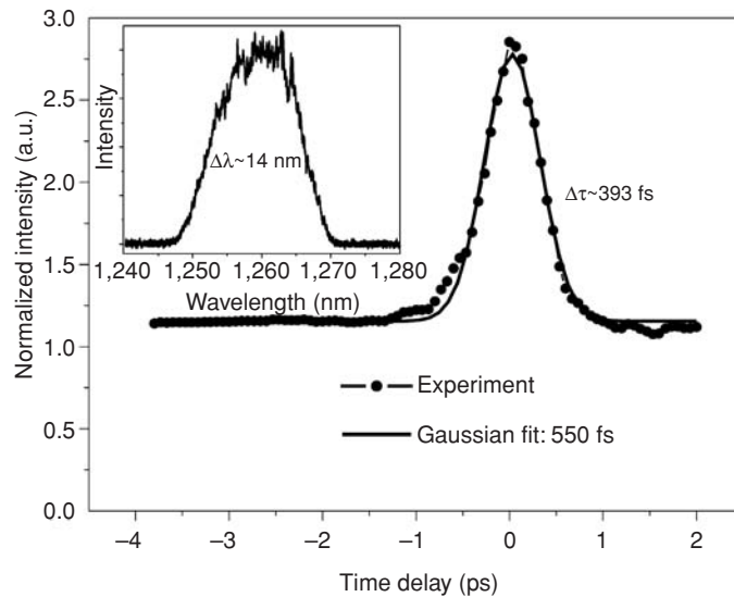
Fig. 5.38 The measured intensity autocorrelation trace and the optical spectrum (insert) of a passively mode-locked quantum dot injection laser using a quantum dot saturable absorber for mode-locking. Reprinted with permission from [109]. Copyright 2005, AIP.
