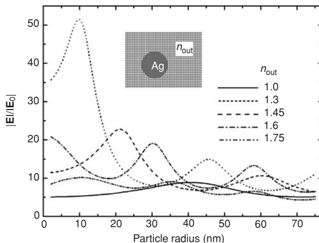
Fig. 11.1 Local electric field enhancement factor |E|/|E_0| near a spherical silver particle embedded in the medium with refractive index n_{\text{out}} . Wavelength is 400 nm. Adapted from [11].
