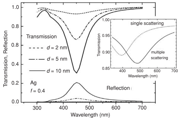
Fig. 11.5 Transmission and reflection spectra for a monolayer of identical silver spherical particles with various diameters d = 2, 5, 10 nm in a medium with refractive index n_{\text{out}} = 1.4 . Silver volume filling factor f = 0.4 . The inset shows transmission spectra calculated based on single scattering (dashes) and multiple scattering (solid line) approach (particle diameter d = 2 nm, volume filling fraction f = 0.6 , ambient refractive index n_{\text{out}} = 1.4 ). Adapted from [19].
