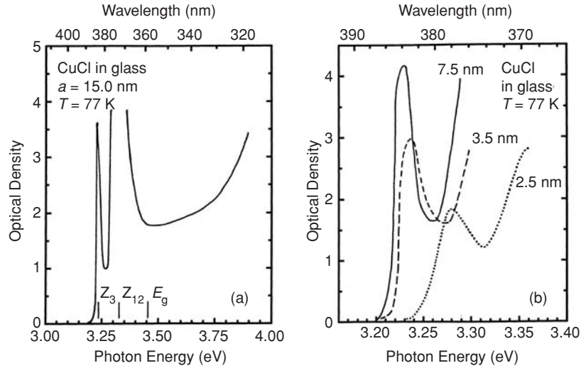
Fig. 5.3 The quantum size effect on exciton absorption of CuCl nanocrystals in a glass matrix [8]. Panel (a) shows an absorption spectrum of larger nanocrystals ( a = 15 nm) in a wide spectral range. The sharp increase in absorption at \lambda < 340 nm is due to glass matrix absorption. Panel (b) shows in detail the Z_3 -exciton absorption band for a = 7.5, 3.5, 2.5 nm.
