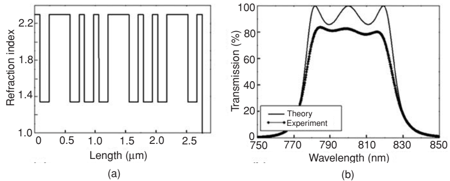
Fig. 3.24 A three-cavity dielectric structure and its transmission spectrum [22]. (a) Refraction index profile of an experimentally developed multilayer film. Wider portions form cavities whereas alternating thinner layers form dielectric reflectors. (b) Calculated and measured central part of a transmission spectrum.
