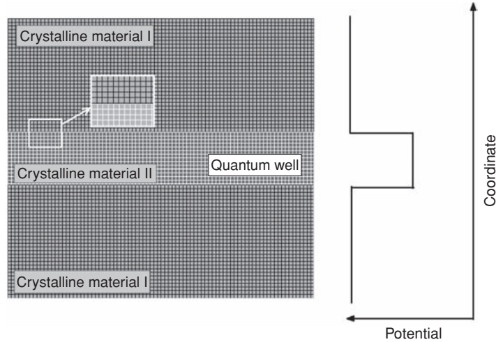
Fig. 4.16 A heterostructure containing a narrow-band quantum well between two crystalline materials with wider band gaps (left) and the corresponding potential profile for an electron.
