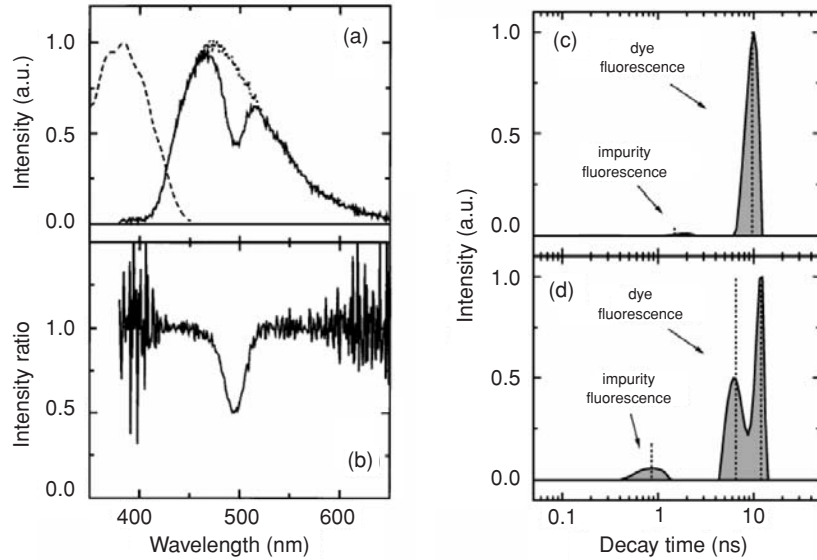
Fig. 14.5 Spontaneous emission of 1,8-naphthoylene-1',2'-benzimidazole (NBIA) dye molecules in poly(methylmethacrylate) (PMMA) impregnated into an artificial opal [25]. (a) Emission spectrum in opal (solid line), in a reference PMMA film (dots), and excitation spectrum (dashes). (b) Difference of emission spectra in an opal and in the reference film. (c) Decay time distribution in the reference film. (d) Decay time distribution in an opal.
