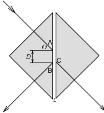
A two-prism geometry to observe frustrated total internal reflection.
