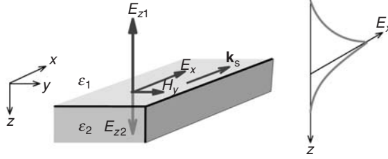
Fig. 6.5 The interface of two media with dielectric functions \varepsilon_1 and \varepsilon_2 and the x -component of electric field vector E_x evanescently in both media along the z -axis from the point z = 0 . k_s stands for the wave vector of the surface plasmon polariton.
