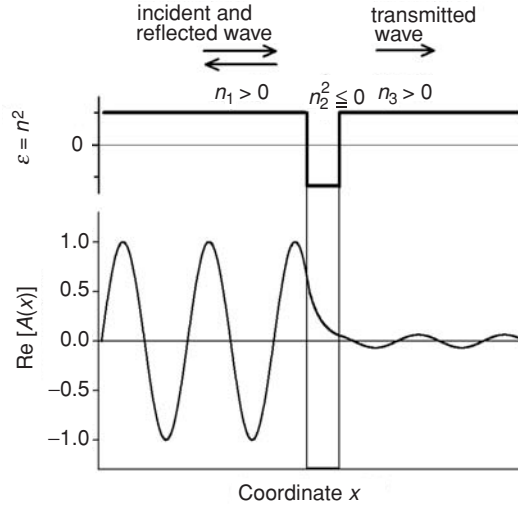
Fig. 3.14 Propagation of an electromagnetic wave through a rectangular well of dielectric permittivity \varepsilon , reaching negative values in the finite interval of x . Such a well develops if a metal film is embedded in a dielectric environment. Evanescent waves give rise to the transmitted plane wave behind the film.
