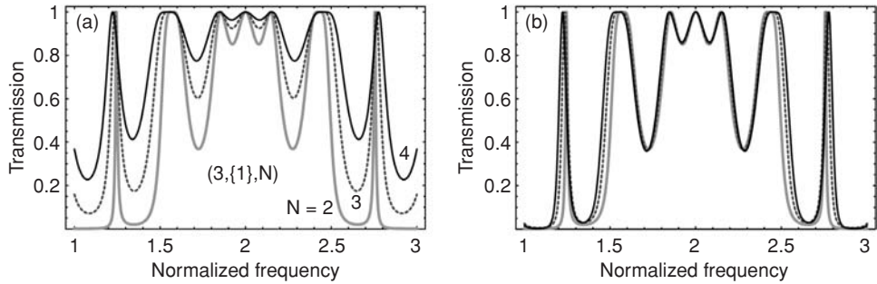
Fig. 8.16 Exact comparison of the scaled spectra for triadic Cantor structures: (a) unchanged, (b) raised to a power \gamma [29].
