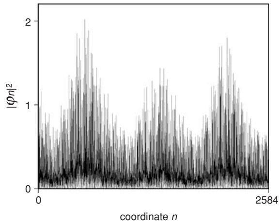
Fig. 8.20 Electron charge profile for a Fibonacci stepwise potential in a finite slab containing F_{17} = 2584 cells [36]. The graph presents the probability of finding an electron at the site with number n .
