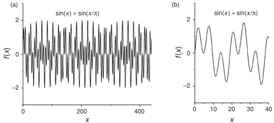
Fig. 8.19 An example of a quasiperiodic function (8.44) plotted for (a) larger and (b) smaller range in the x scale.
