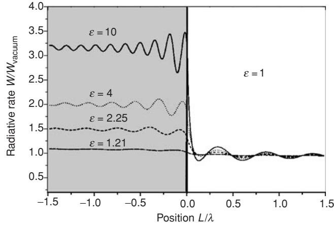
Fig. 14.8 Calculated decay rate of an atom near a dielectric vacuum interface for four different values of dielectric permittivity. The dielectric area is shaded with gray. Adapted from [40].
