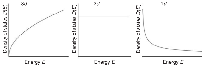
Fig. 4.14 Density of states functions for a quantum particle with non-zero rest mass in spaces with different dimensionalities.
