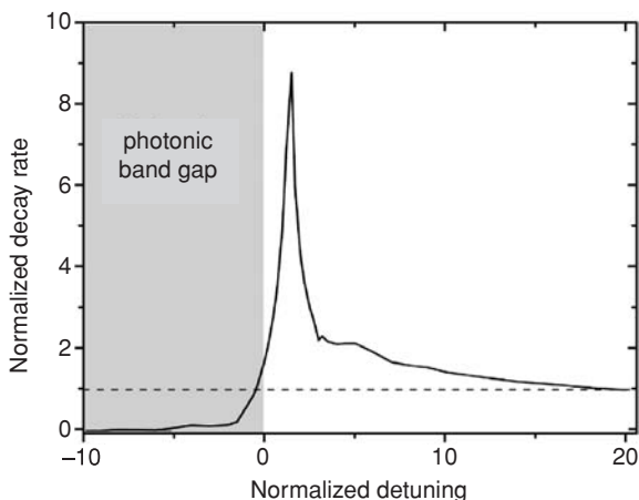
Fig. 14.4 Calculated decay rate within the assumption of the perturbative approach of a two-level quantum system in a photonic crystal normalized with respect to vacuum rate versus normalized dimensionless detuning of the transition frequency with respect to photonic band gap edge. Dashed line shows vacuum rate. Adapted from [21].
