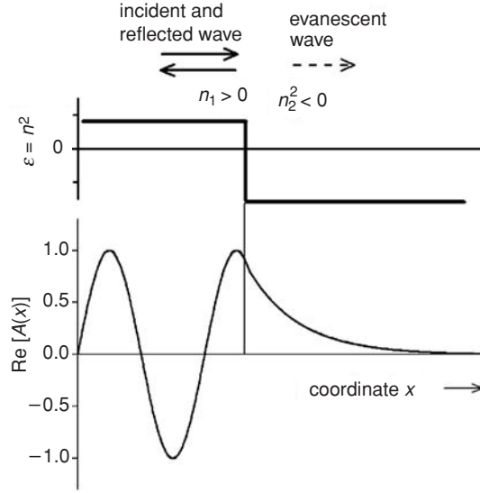
Fig. 3.11 Dielectric permittivity profile (top) and electric field amplitude (bottom) at a dielectric-metal interface. There are incident and reflected electromagnetic waves in front of the interface and an evanescent field inside the metal.
