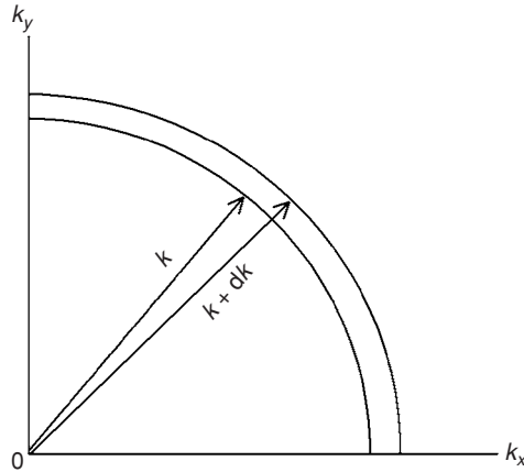
An elementary layer in 2d k -space.
