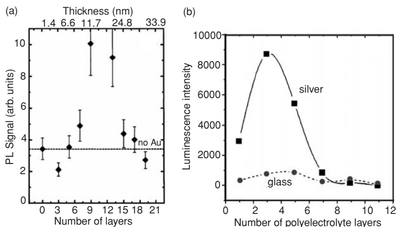
Fig. 16.10 Photoluminescence intensity as a function of the number of polyelectrolyte layers forming a dielectric spacer over a metal surface. (a) Core-shell CdSe/ZnS semiconductor nanocrystals with mean diameter 4 nm on a nanotextured gold surface [31]; (b) Albumin-fluorescein isothiocyanate conjugate of bovine serum on a nanotextured silver surface [32].
