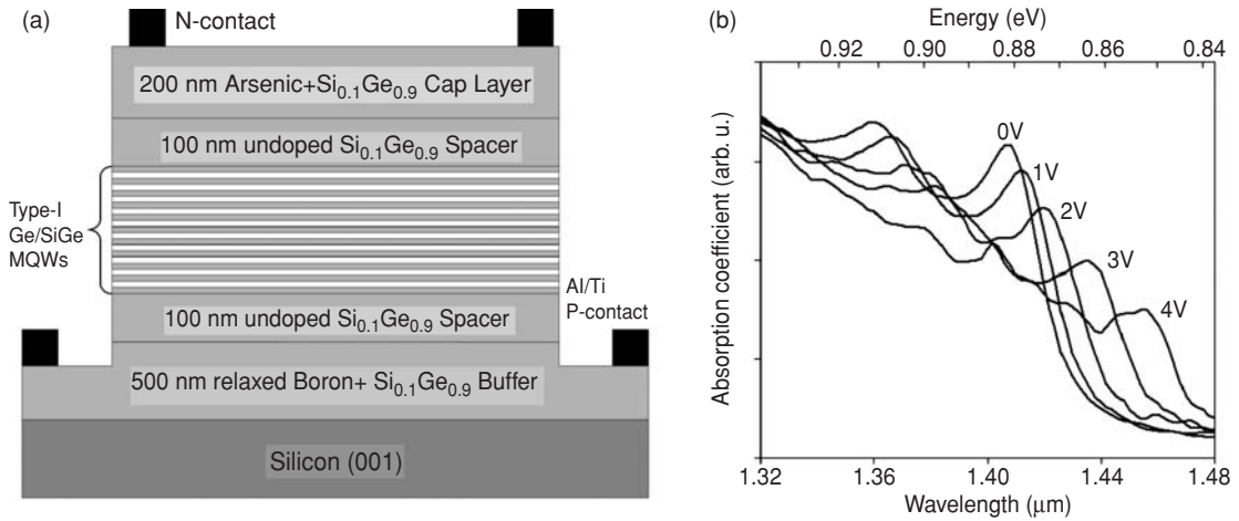
Fig. 4.18 (a) Electro-absorptive multiple quantum well structure and (b) its absorption spectra at various applied voltages. Reprinted with permission from [25]. Copyright 2005 Nature Publ. Group.
