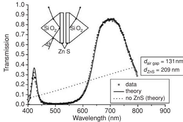
Fig. 10.3 Transmission spectra of light waves traversing an air gap between two silica prisms under conditions of total internal reflection with and without a pair of thin ZnS layers. The experimental configuration is shown in the inset. Angle of incidence \theta = 68.2^\circ . Adapted from [6].
