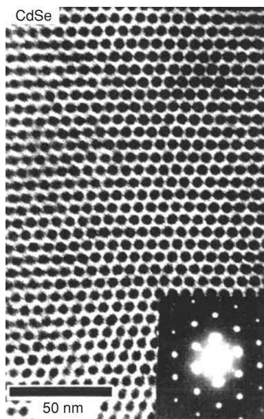
Fig. 5.23 A high-resolution transmission electron microscopy image and small-angle electron diffraction pattern (insert) of a three-dimensional quantum dot superlattice [73]. The superlattice consists of CdSe nanocrystals of 4.8 nm diameter each. Nanocrystals are assembled in a face-centered cubic lattice. Image corresponds to (101) crystallographic plane of the array.
