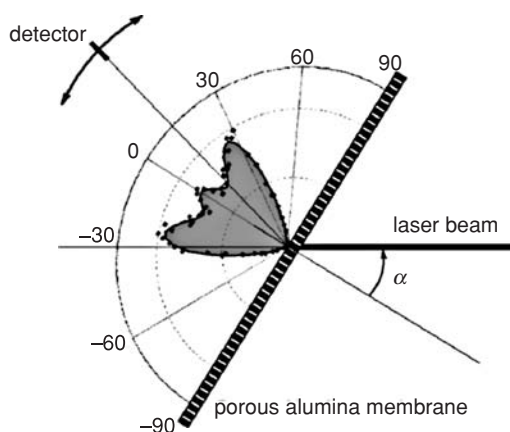
Fig. 14.12 Anisotropic scattering of light in a nanoporous alumina slab. A slab and pores geometry are presented along with transmitted light indicatrix for laser light incident at an angle 30^\circ with respect to the pore axes [68]. See text for detail.
