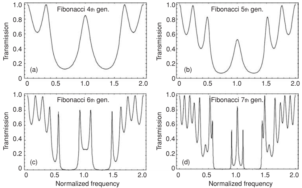
Fig. 8.21 Calculated transmission spectra of quarter-wave Fibonacci filters of (a) 4th, (b) 5th, (c) 6th and (d) 7th generations [31].
