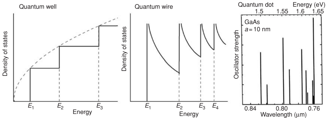
Fig. 4.15 Electron density of states in a quantum well, in a quantum wire and calculated probabilities for optical transitions in a realistic GaAs quantum dot with size 10 nm. Data for GaAs dots are taken from Ref. [20].
