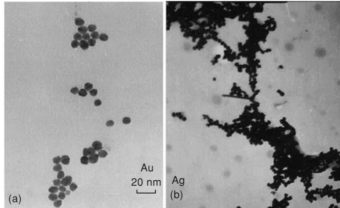
Fig. 6.8 Images of (a) gold and (b) silver nanoparticles obtained by means of transmission electron microscopy.
