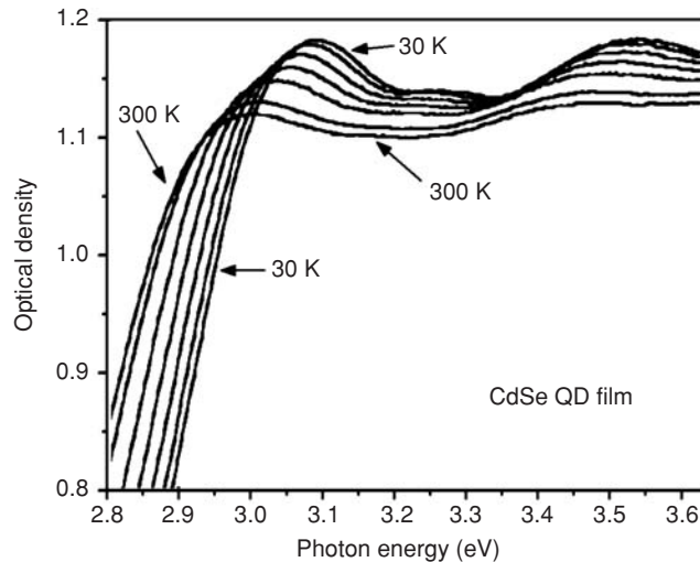
Fig. 5.28 A portion of the absorption spectrum of close-packed CdSe quantum dots measured at different temperatures ranging from 300 K to 30 K. The insert shows spectra at 300 and 30 K in a wider range [79].
