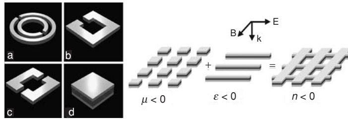
Fig. 11.15 Examples of elementary building units to get magnetic permeability in a regular array (a-d) and design of a negative refraction material by means of combined arrays with negative permeability and negative permittivity. Reprinted with permission from [6]. Copyright 2007, Elsevier B.V.
