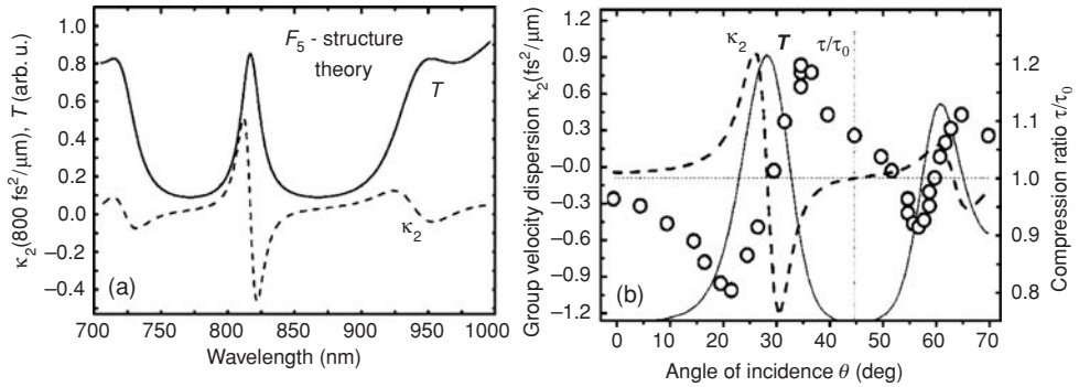
Fig. 8.26 Application of a Fibonacci filter for chirped pulse compression (adapted from [46]). (a) Calculated transmission T and group velocity dispersion \kappa_2 for a 5th order Fibonacci ZnS/Na 3 AlF 6 filter. (b) Measured compression ratio \tau/\tau_0 (circles) superimposed with calculated group velocity dispersion \kappa_2 and transmission T (not scaled) for that filter as a function of the angle of incidence. Compression corresponds to \tau/\tau_0 < 0 .
