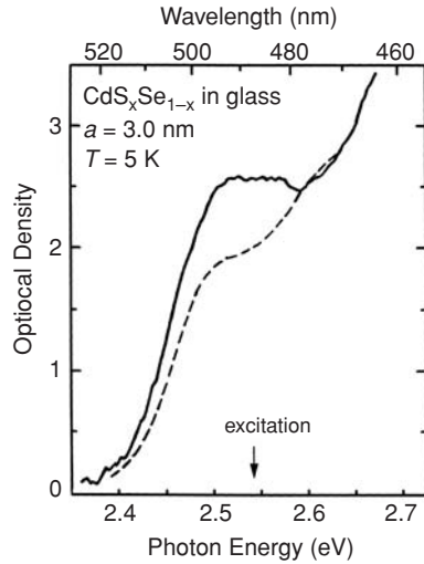
Fig. 5.29 Modification of the absorption spectrum of a typical commercial-based semiconductor-doped glass under conditions of laser excitation [84]. Solid line – original spectrum, dashed line – spectrum of excited sample, arrow indicates position of the laser wavelength. Laser pulse duration is 10 ns, intensity is about 1 MW/cm 2 .
