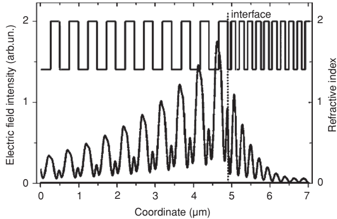
Fig. 8.29 Formation of a localized state at the interface of two periodic media with different periods but with overlapping gaps. Shown are the refractive index profile (upper curve) and electric field profile (lower curve). Adapted from [56].
