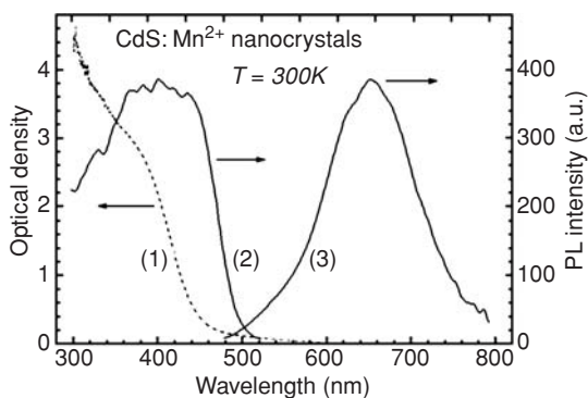
Fig. 5.40 Optical properties of CdS : Mn 2+ nanocrystals in a polymer film [110]: (1) absorption, (2) excitation (emission at 650 nm) and (3) emission spectra (excitation at 415 nm).
