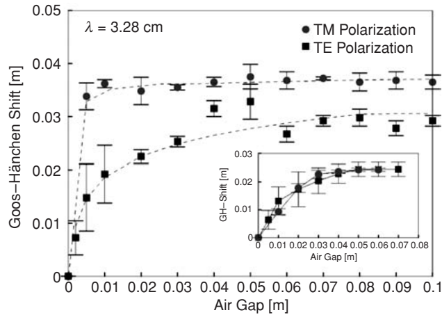
Fig. 10.2 The Goos-Hänchen shift versus air gap width for TE and TM polarizations. The beam aperture is 80 mm. The insert shows the shift for a TM- and a TE-polarized beam for a larger aperture 190 mm [3].
