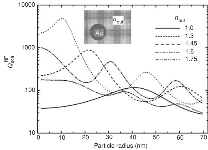
Fig. 11.4 Near-field scattering cross-section of a single silver particle depending on its radius for different values of ambient refractive index n_{\text{out}} . Wavelength is 400 nm. Adapted from [11].
