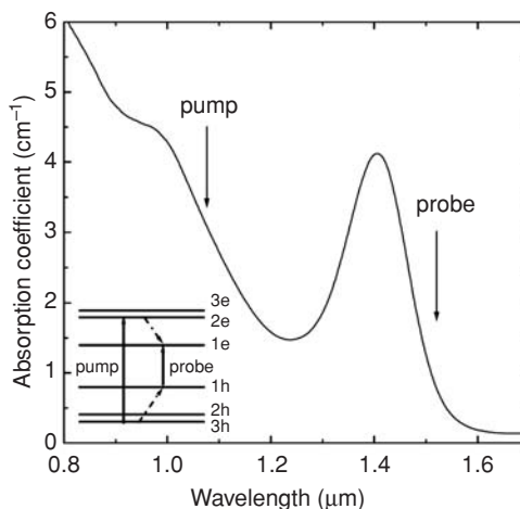
Fig. 5.31 Room-temperature absorption spectrum of silicate glass doped with PbS QDs. Inset is the energy-level diagram for PbS QDs. Reprinted with permission from [87]. Copyright Elsevier Ltd.
