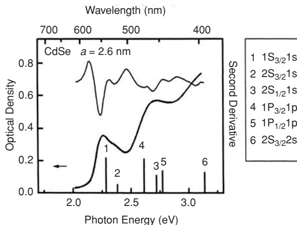
Fig. 5.17 Optical absorption spectrum of CdSe nanocrystals in a silicate glass matrix ( T = 300\text{ K} ), its second derivative (upper curve) and calculated energy positions and relative weights of the transitions shown by vertical lines. The assignment of the transitions is shown where 1S, 2S, and 1P labels stand for mixed hole states and 1s, 2s, and 1p labels stand for electron states in a spherical potential well [8, 50].
