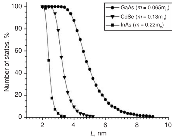
Fig. 5.26 Number of delocalized electron states versus average interdot spacing L in an ensemble of randomly arranged spherical potential wells with radius 1 nm. Electron effective mass of GaAs (circles), CdSe (triangles) and InAs (squares) was used in calculations. Courtesy of A. I. Bibik [78].
