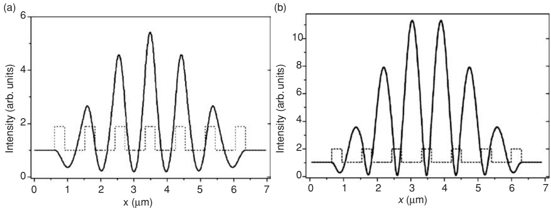
Fig. 7.4 Spatial intensity profile in a finite periodic multilayer structure for transmission bands in the close vicinity to band gap edges (a) \omega_1 and (b) \omega_2 [13]. Dashed lines show the refractive index profiles.
