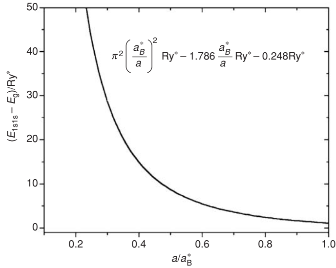
Fig. 5.6 The universal law in terms of dimensionless energy and radius units describing the size dependence of the first optical resonance in a quantum dot (Eq. 5.11).
