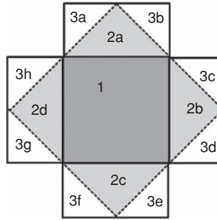
Fig. 4.3 The first three Brillouin zones (BZ) of a simple two-dimensional square lattice. The first BZ is a square with the side equal to 2\pi/a . The second BZ consists of four triangles. The third BZ consists of eight triangles. Every BZ has a square equal to (2\pi/a)^2 .
