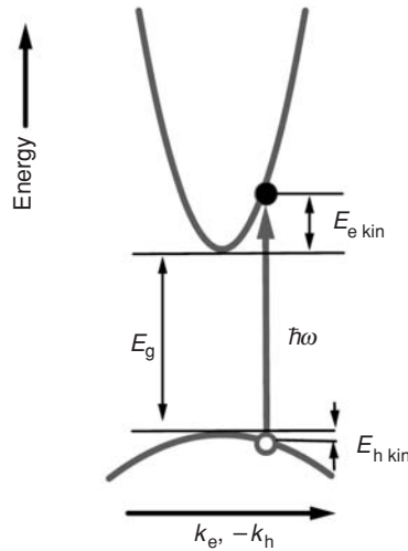
Fig. 4.7 A process of photon absorption resulting in creation of one electron-hole pair. In a diagram including dispersion curves for conduction and valence bands this event can be shown as a vertical transition exhibiting simultaneous energy and momentum conservation.
