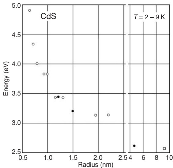
Fig. 5.9 Energy of the first absorption maximum measured for CdS nanocrystals and clusters at temperature 2–9 K in different matrices. Adapted from [12].
