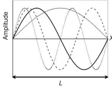
Fig. 2.2 Normal modes inside a cube. The first four modes are shown with wave numbers k = \pi/L, 2\pi/L, 3\pi/L, 4\pi/L .
