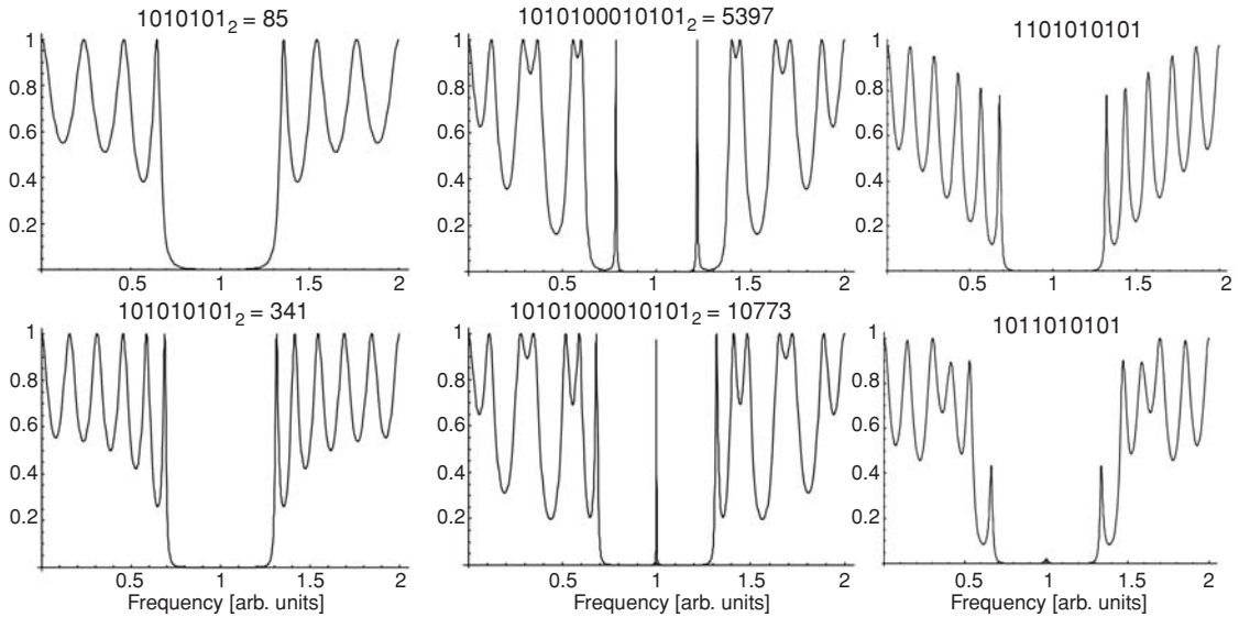
Spectral portraits of different numbers [57].
