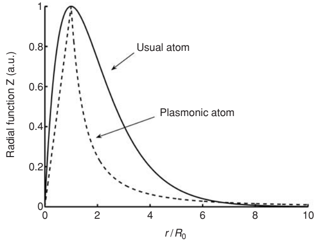
Fig. 6.12 Radial wave functions Z of a hydrogen ( 2p -state of an electron) and a plasmonic atom versus normalized distance from the centre. The parameter R_0 = \sqrt{2}a_B for a hydrogen atom ( a_B is the Bohr radius). For a metal nanoparticle the parameter R_0 equals the particle radius. The solid line corresponds to a usual atom and the dashed line corresponds to the plasmonic atom. Reprinted with permission from [23]. Copyright 2007 Springer.
