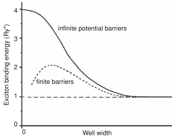
Fig. 4.17 Evolution of the exciton binding energy for a quantum well width tending to zero. For the case of unrealistic infinite potential barriers confining electron and hole motion, exciton binding energy tends to 4Ry^* , predicted for the pure two-dimensional Schrödinger problem with Coulomb potential. For realistic finite barriers inherent in heterostructures, the exciton binding energy increases with decreasing well width, but eventually drops back to the Ry^* value at vanishing well width.
