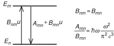
Fig. 13.1 A pair of energy levels of a quantum system and relations between Einstein coefficients A , B . u is the radiation energy density as in Eq. (13.6).
