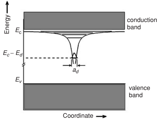
Fig. 4.10 The Coulomb potential of a donor impurity superimposed with conduction and valence bands, showing the electron energy spectrum and wave function of the lowest impurity state.
