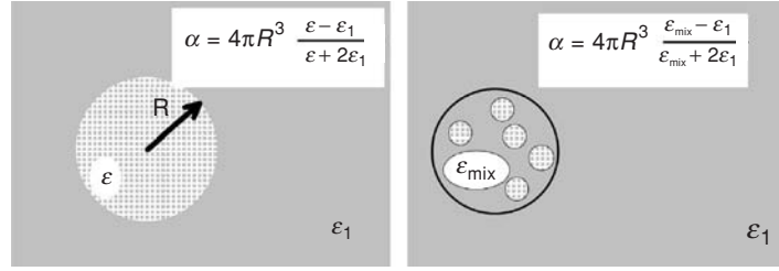
Fig. 6.9 Application of Eq. (6.53) to (left) a homogeneous and (right) a composite particle in a host medium.
