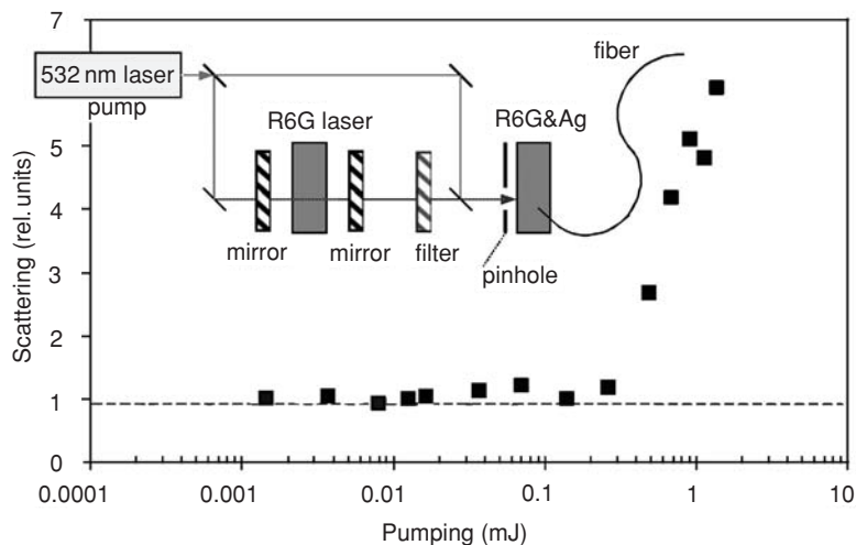
Fig. 11.10 Relative intensity of Rayleigh scattering as a function of the pumping energy for a solution of Rhodamine 6G dye with Ag nanoparticles. Adapted from [32]. Inset: experimental setup. Copyright 2007 Elsevier Ltd.
