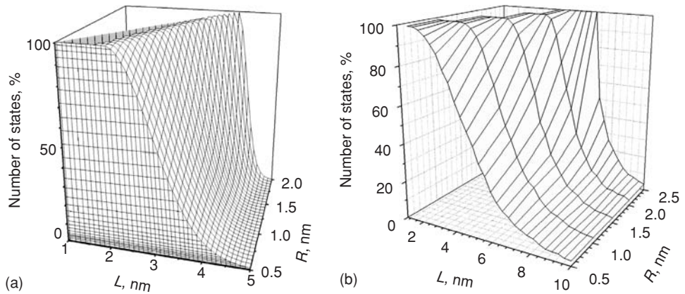
Fig. 5.25 Number of calculated delocalized electron states versus average interdot spacing L for several values of dot radius R . Electron effective mass is 0.13m_0 (CdSe, left) and 0.065m_0 (GaAs, right) [78].
