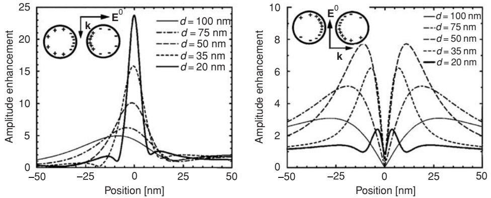
Fig. 11.2 Electric field amplitude enhancement for coupled silver cylinders. Diameter d for the two different orientations of the incident field E^0 and wave vector k . The separation between the cylinders is scaled with d and equals 0.2d . Adapted from [12].
