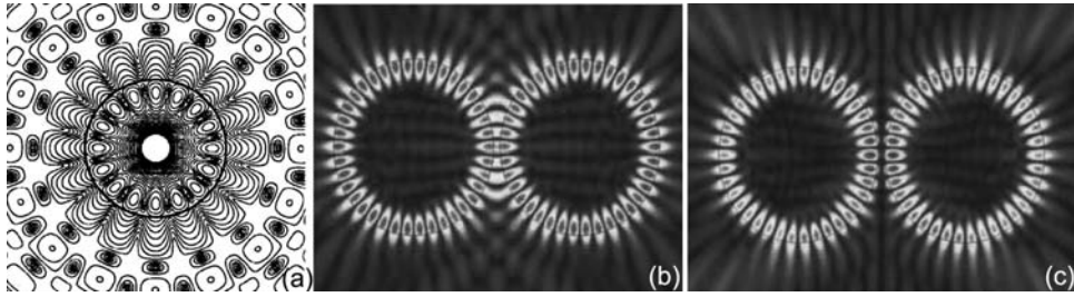
Fig. 9.10 Light intensity distribution (a) in a single microdisk [42] and (b), (c) in coupled microspheres [43]. See text for detail.
