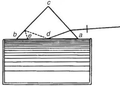
Fig. 3.17 The elegant performance providing visualization of an evanescent wave under the condition of frustrated total reflection. A glass prism borders a solution of fluorescent dye (L. Mandelstam, 1914 [17])
