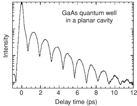
Fig. 15.3 Vacuum Rabi oscillations observed for an excitonic emission band in a GaAs quantum well inside a planar Fabry–Perot \lambda/2 cavity formed by a pair of multilayer semiconductor Bragg reflectors [10].
