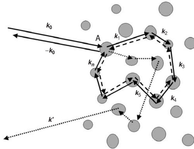
Fig. 8.4 Multiple scattering in a turbid medium with random scatterers indicating constructive interference at point A resulting in enhanced backward scattering.
