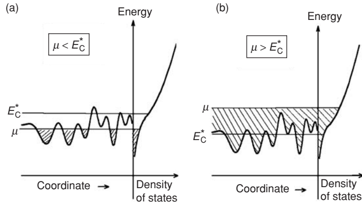
Fig. 4.12 A sketch of electron energy and density of states in a random potential for the case (a) of the Anderson dielectric and (b) of metallic conductivity.
