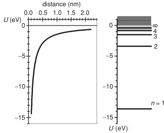
Fig. 2.8 The Coulomb potential -e^2/r (left) and energy levels of an electron. For E < 0 the energy spectrum consists of discrete levels E_n = -E^0/n^2 , E^0 = 13.60 eV, each level being n^2 -degenerate. For E > 0 a particle exhibits an infinite motion with a continuous energy spectrum.
