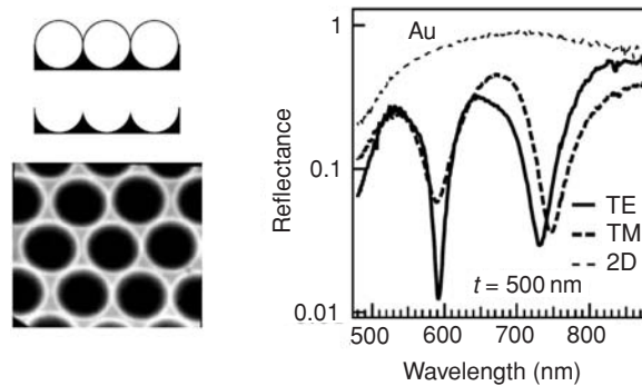
Fig. 11.6 A metal structure with hemispherical voids: (left) synthesis, and (right) reflectance spectra for a 500-nm-thick graded sample [21]. Void radius is 350 nm. Solid line corresponds to TE- and dashes correspond to TM-polarized incident light for an angle of incidence equal to 45^\circ . The dotted curve is the reflectance of a reference unpatterned film electrodeposited under the same conditions.
