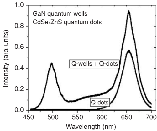
Fig. 5.44 White light emission spectrum of a hybrid system consisting of GaN quantum well + CdSe/ZnS core-shell quantum dots. Adapted from [112].
