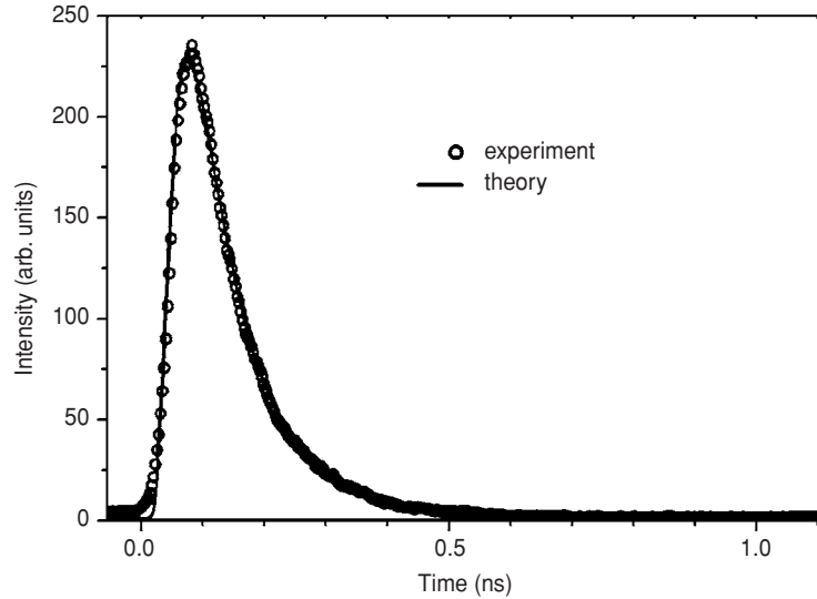
Fig. 8.3 Time-resolved transmission through a slab of porous silica, infiltrated with the liquid crystal 8CB (adapted from [3]). Pore size is 100 nm, volume fraction of the pores is 38%, sample thickness is 2 mm. Circles are experimental data, the solid line is a fit from the diffusion theory using Eq. (8.12). The resulting diffusion constant is D = 4.2 \cdot 10^3 \text{ m}^2/\text{s} with 10% accuracy. Ten first terms in the sum in Eq. (8.13) were found to be enough to get convergence in the series.
