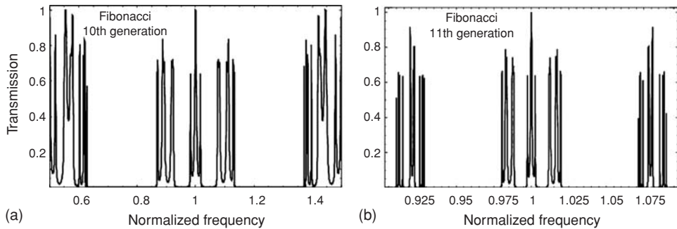
Fig. 8.23 Scalability of transmission spectra of Fibonacci multilayer structures [31]. (a) The central portion of the spectrum for the 10th generation; (b) the central portion of the spectrum for the 11th generation with 5.11-fold stretching of the frequency axis.
