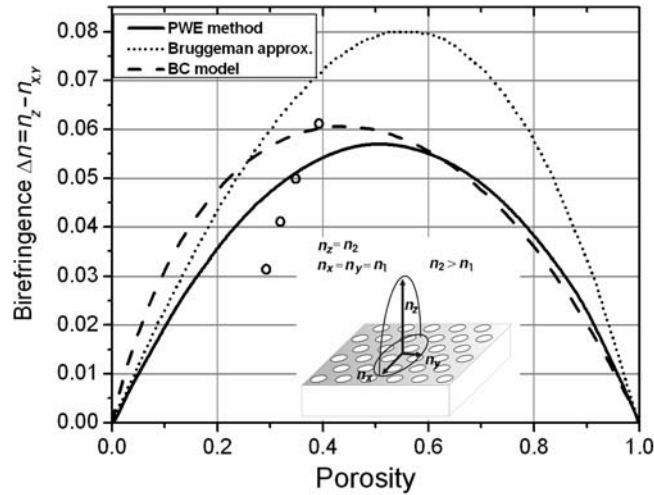
Fig. 7.29 Modelling of birefringence in nanoporous alumina depending on the porosity (lines) and experimental values of the birefringence (circles) [52]. PWE stands for plane wave expansion, BC stands for boundary conditions. The inset shows an explanation of refractive indices used to define birefringence.
