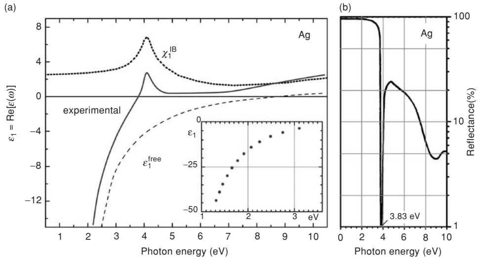
Fig. 6.3 Optical properties of silver (adapted from [8]). (a) Experimentally observed real part \varepsilon_1 of the dielectric function of bulk solid silver (solid line) and its decomposition into free electron gas contribution \varepsilon_1^{\text{free}} (long dashes) and interband transitions contribution \chi_1^{\text{IB}} (short dashes). The insert shows experimental data in a wider range. (b) Experimentally observed reflectance spectrum.
