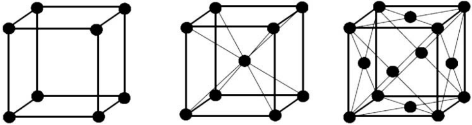
Fig. 4.4 Elementary cells of cubic lattices (from left to right): simple, body-centered, and face-centered.
