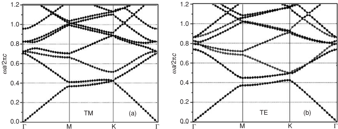
Fig. 7.19 The photonic band structure of a two-dimensional triangular lattice of air cylinders with radius R(\varepsilon = 1) in alumina ( \varepsilon = 2.72 ) for R/a = 0.3 [52]. (a) TM-modes; (b) TE-modes.
