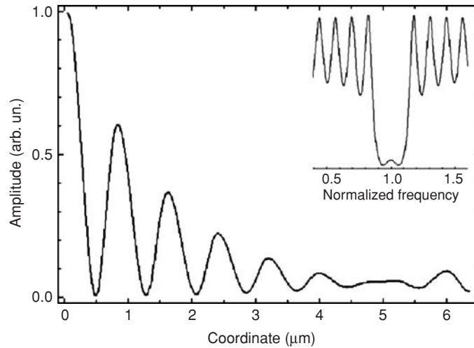
Fig. 8.28 Development of a localized state within the band gap of a seven-period quarter-wave multilayer structure bordering at 6 \mu\text{m} a dielectric medium with very high dielectric constant [55]. The plot shows the electric field amplitude profile at the mid-gap frequency (normalized frequency = 1). The insert shows the central portion of the transmission spectrum.
