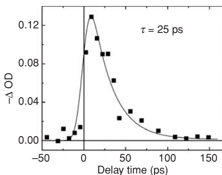
Fig. 5.32 Kinetics of bleaching relaxation for PbS-doped glass at 1.524 \mu\text{m} after the pump at 1.08 \mu\text{m} (squares) and result of the best fit (line). Reprinted with permission from [87]. Copyright Elsevier Ltd.
