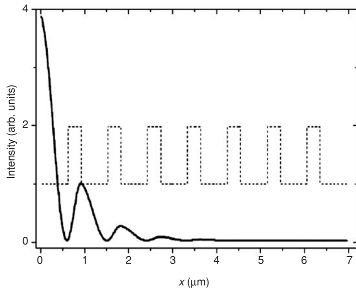
Fig. 7.5 The spatial intensity profile in a finite periodic multilayer structure for the frequency value in the center of the band gap \omega_0 [13]. The dashed line shows refractive index profile.
