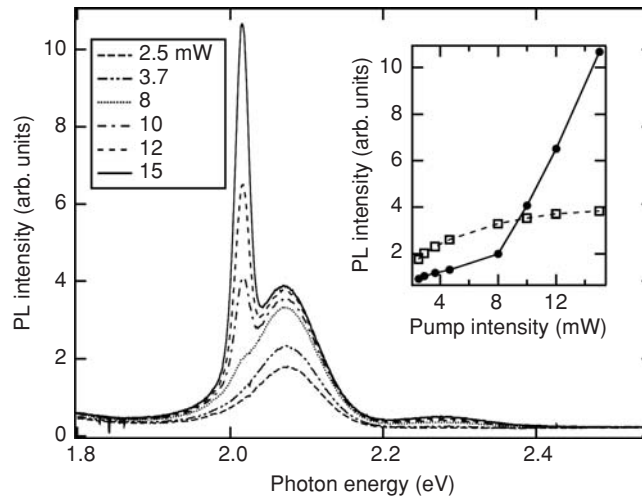
Fig. 5.36 Development of a sharp stimulated emission band as a function of pump intensity in photoluminescence spectra of films ( T = 80 K) fabricated from TOPO-capped CdSe nanocrystals with radius 2.1 nm [97]. The inset shows superlinear intensity dependence of the stimulated emission (circles) with a clear threshold compared to the sublinear dependence of the PL intensity outside the sharp stimulated emission peak (squares). Reprinted with permission from AAAS.
