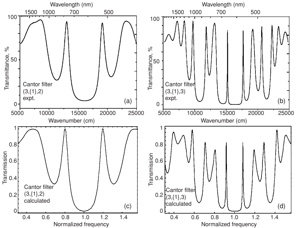
Fig. 8.15 Transmission spectra of triadic Cantor filters of the second (9 layers) and the third (27 layers) generations consisting of ZnSe and \text{Na}_3\text{AlF}_6 [28]. (a) N = 2 , experiment; (b) N = 3 , experiment; (c) N = 2 , calculations, (d) N = 3 , calculations.
