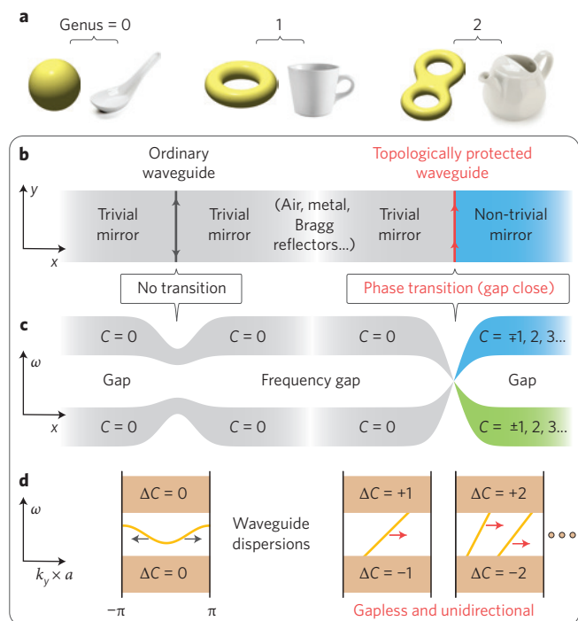
Figure 1 | Topological phase transition. a , Six objects of different geometries can be grouped into three pairs of topologies. Each pair has the same topological invariant, known as its genus. b , Two waveguides formed by mirrors of different (right) and same (left) topologies. c , Frequency bands of different topologies cannot transition into each other without closing the frequency gap. A topological phase transition takes place on the right, but not on the left. d , Interfacial states have different connectivity with the bulk bands, depending on the band topologies of the bulk mirrors. Here, a is the period of the waveguide propagating along y , and \Delta C is the change in Chern number between the corresponding bulk bands on the right and left of the waveguide. The magnitude of \Delta C equals the number of gapless interfacial modes and the sign of \Delta C indicates the direction of propagation.
