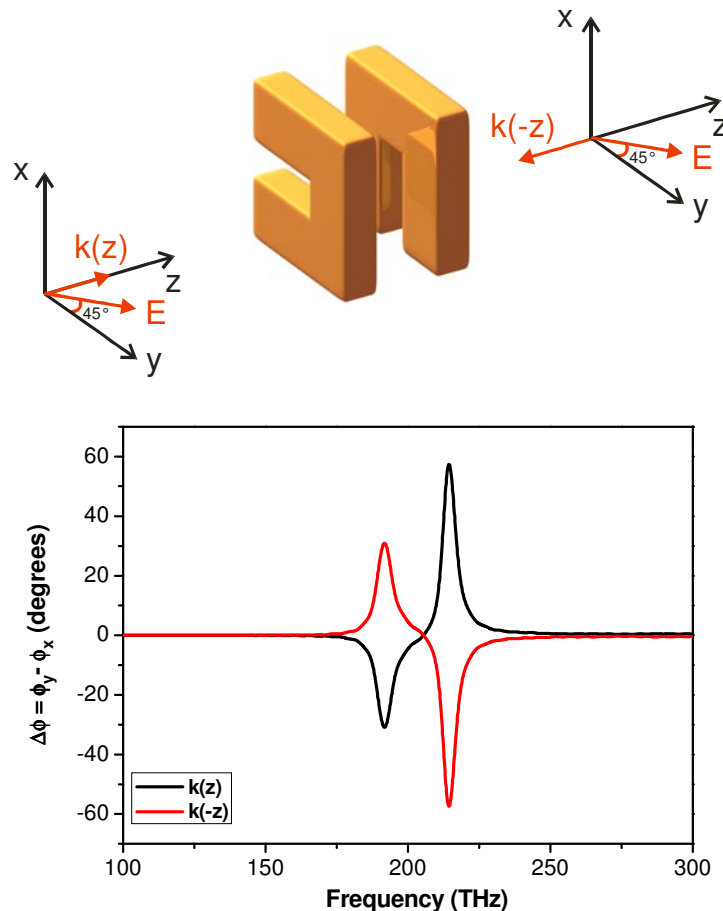
Fig. S1. The phase difference of the two components of the transmitted wave \Delta\phi = \phi_y - \phi_x for two opposite propagation directions for the 90^\circ twisted SRR dimer. The vertical distance between the two SRRs is 100 nm. The incident electric field E is at 45^\circ between the x and y axes. When the wave vector k(z) changes to the opposite direction k(-z) , \Delta\phi alters its sign accordingly, i.e., \Delta\phi(-z) = -\phi(z) .
