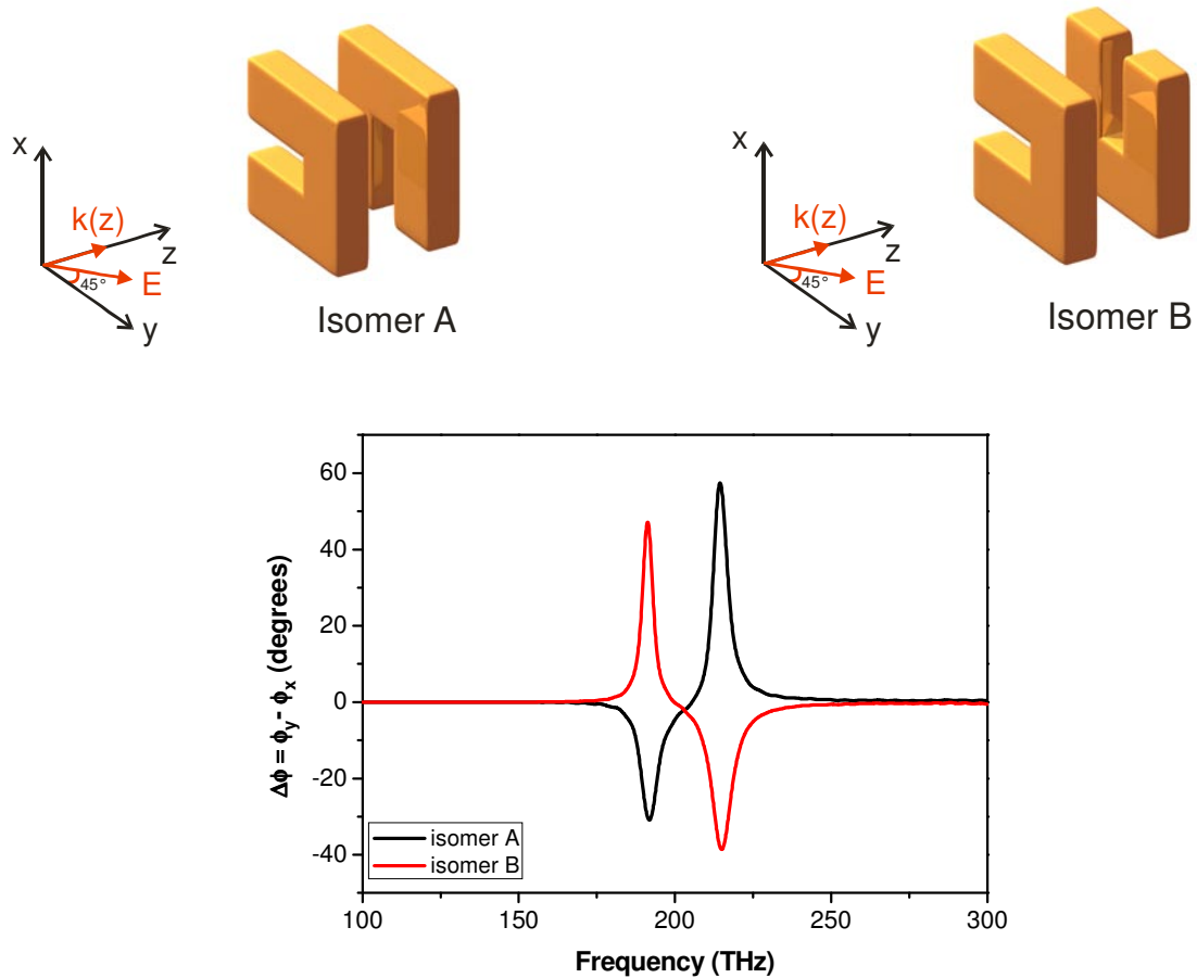
Fig. S2. The phase difference of the two components of the transmitted wave \Delta\phi = \phi_y - \phi_x for two isomers with opposite twist angles. The vertical distance between the two SRRs is 100 nm. The incident electric field E is at 45° between the x and y axes. The phase difference \Delta\phi shows quite different behavior for the two isomers.
