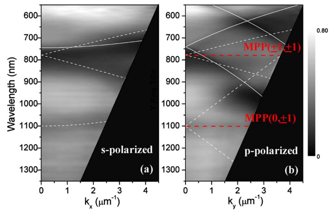
FIG. 5. (Color online) Measured transmission maps for sample E in (a) s-polarization and (b) p-polarization, in which solid curves are the dispersion of diffracted light and dashed curves are the calculated MPP modes by Eq. (2), and the red dashed line are calculated by Eq. (3).
