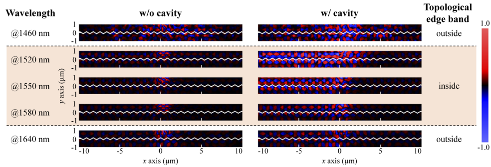
Fig. 3. Calculated mode distribution of propagating light at typical wavelengths shown in Fig. 2(a). The white line is the interface between trivial and topological PhCs.
