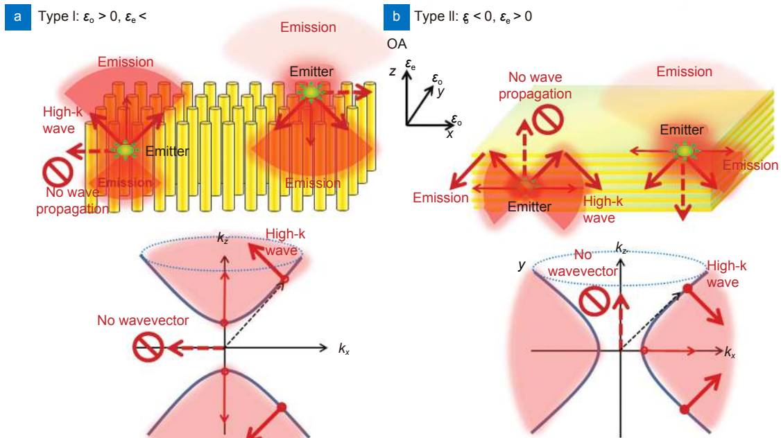
Fig. 1 | Schematic illustration of hyperbolic metamaterials and metasurfaces. (a) Type I hyperbolic metamaterials ( \epsilon_o > 0 and \epsilon_e < 0 ) in metallic nanorod or nanowire configuration and their representative dispersion in the wavevector space (k-space). (b) Type II hyperbolic metamaterials ( \epsilon_o < 0 and \epsilon_e > 0 ) in metal-dielectric multilayer configuration and their dispersion in the wavevector space.
