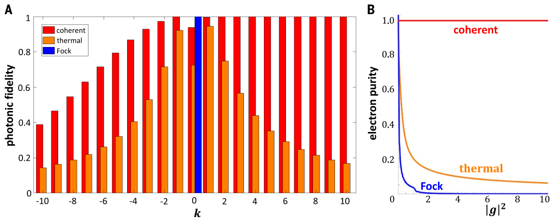
Fig. 4. Photonic fidelity and electron purity after a free-electron-quantum-light interaction. (A) Calculated fidelities between the photonic state before and after its interaction with a free electron, which subsequently undergoes a projective measurement. The fidelity is plotted as a function of the energy state |E_0 - \hbar\omega k\rangle in which the electron is detected. We present the fidelity for different states of light, all with an average photon number \langle n \rangle = 100 and quantum coupling g_q = 0.1 . The fidelity is high for a coherent state, indicating that for small-enough g_q , the electron can serve as a probe of quantum weak measurement. For the thermal state, the fidelity is much lower, indicating a
