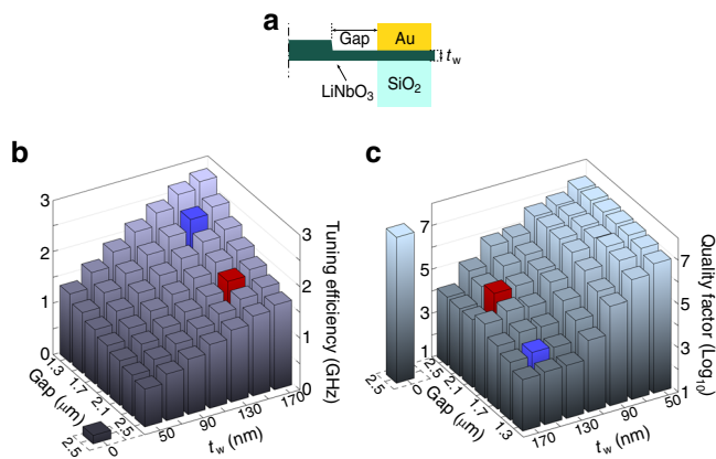
Fig. 8 Numerical modeling of electro-optic coupling. a Schematic of half of the cross-section of the EOM structure. “Gap” denotes the spacing between the gold electrode and the LN cavity, and “t w ” denotes the thickness of the waveguide wing layer. b , c Electro-optic tuning efficiency and optical quality factor of the device as a function of Gap and t w , simulated by the FEM method. The red column represents the parameter design used for the EOMs demonstrated in the main text. The blue column shows another design with broader bandwidth and enhanced electro-optic coupling. The individual column at the left of each plot indicates the case when t w = 0 μm and gap = 2.5 μm, for a device with full surrounding air cladding.
