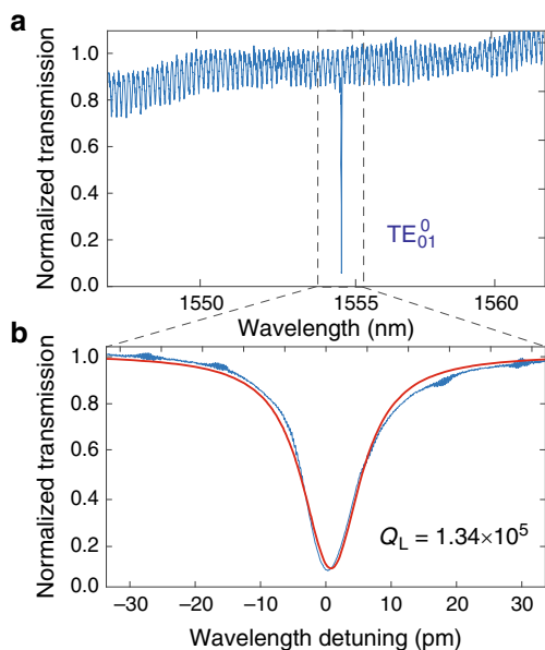
Fig. 4 Linear optical property of a fabricated LN photonic-crystal EOM.
