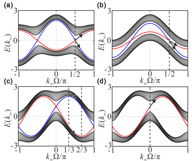
Fig. 3. Sliced band structures at k_x = 0.85\pi/\sqrt{a} of the “zz” lattice for (a)–(c) and the “zb” lattice for (d). (a) and (b) denote the P -broken case and (c) and (d) are the T -broken cases. The black curves denote the bulk bands, and the red (blue) curves denote the surface states with the black arrows denoting the group velocities.
