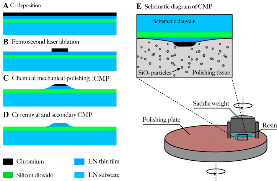
Figure 4: A standard fabrication process of chemical mechanical polishing (CMP). (A) Cr thin film is first deposited on a LNOI wafer and is ablated by femtosecond laser (B) to define the pattern. Then, CMP is implemented (C) to polish lithium niobate thin film. Finally, Cr mask is removed by wet etching and secondary CMP is implemented for a smoother surface (D). (E) shows a schematic diagram for the CMP process. Reprinted with permission from Wu et al. [57].
