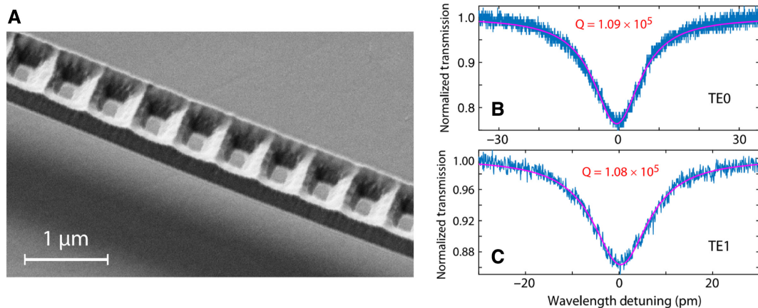
Figure 12: LNOI photonic crystal nanocavities.
