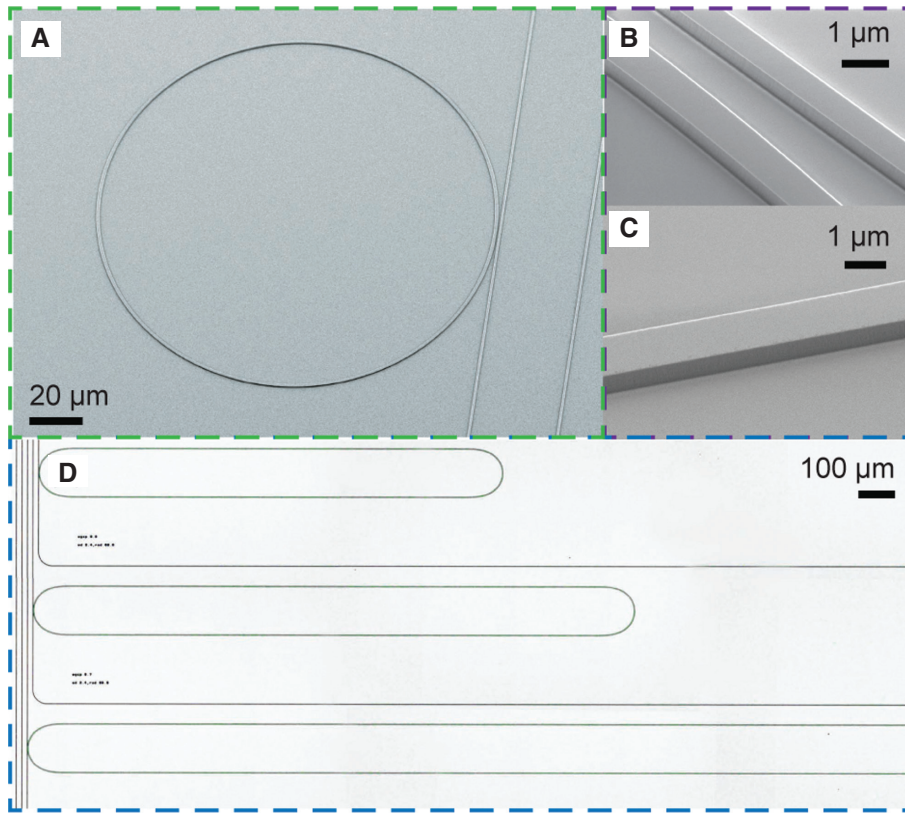
Figure 11: Several typical LNOI microring resonators.
