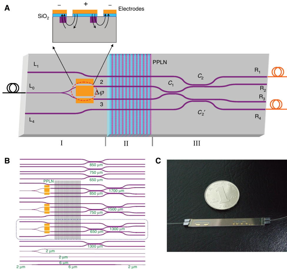
Figure 24: The photonic chip for generating and manipulating entangled photons.
