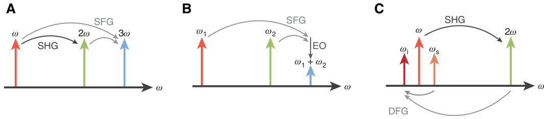
Figure 22: Cascaded nonlinear processes based on integrated LNOI photonics.
