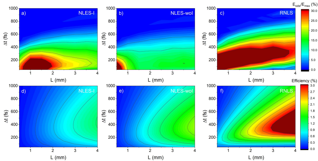
Fig. 3. (a)–(c) Ratio of the side peak to the main peak of the THz pulse and (d)–(f) the efficiency of the THz generation as a function of the pump pulse duration and the crystal thickness, for (a), (d) NLES-I, (b), (e) NLES-wol, and (c), (f) RNLS cases.
