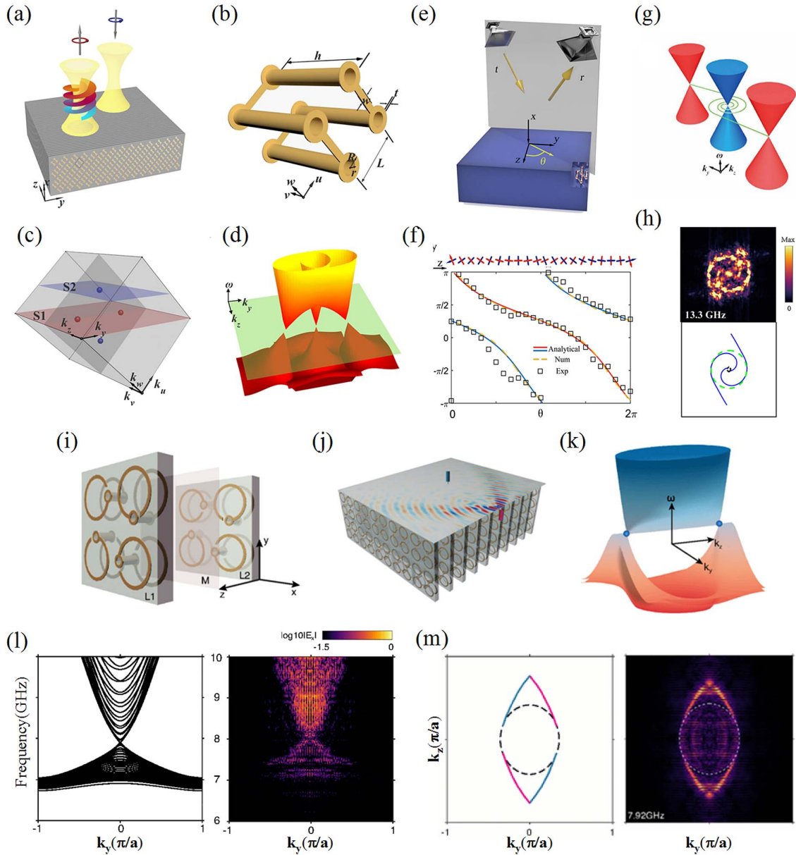
Fig. 3. (a) Schematic of the vortical mirror in Weyl metamaterial. (b) The Weyl metamaterial composed of the metallic saddle-shaped structure. (c) The distribution of ideal Weyl points in Brillouin zone. (d) The overlapped band structures of S_1 and S_2 planes showing ideal Weyl points. (e) Schematic of the reflection measurement setup in microwave. (f) Reflection phases of the Weyl metamaterial. (g) Schematic of spiraling Fermi arcs. (h) Simulation and experiment of the spiraling Fermi arc at 13.3 GHz. (i) Schematic of 3D photonic Dirac metamaterial. (j) Sample configuration for the experimental measurement. (k) The full wave simulation of 3D photonic Dirac point. (l) Experiment (right) and simulation (left) results of 3D photonic Dirac points along the k_y direction. (m) Experiment (right) and simulation (left) results of surface-state arcs at the frequency of Dirac point.
