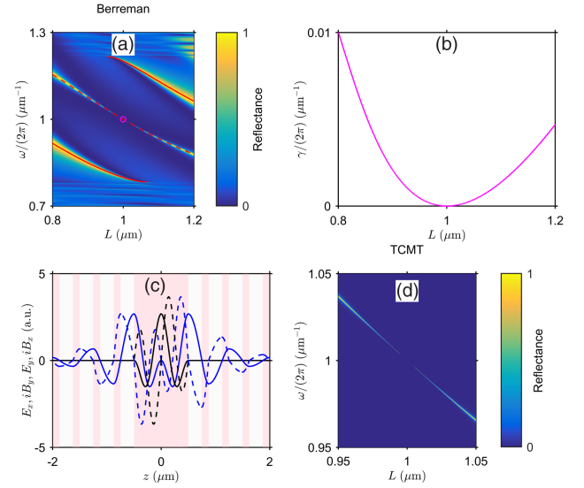
Fig. 3. (a) Zoomed-in reflectance spectrum from Fig. 2(c). Solid red lines show the real part of solution to Eqs. (13) and (14) in the antisymmetric case. The dashed line demonstrates the symmetric solution obtained from Eqs. (13) and (15). The magenta circle shows the position of the BIC from Eq. (20). (b) Imaginary part of solution (13), (15). (c) BIC field profile (21)–(23). All parameters are identical to those in the Fig. 2(c) caption. The normalization condition is used (24) to yield A = \sqrt{2\pi/7} . (d) Reflectance spectrum obtained by temporal coupled-mode theory (TCMT), Eq. (26).
