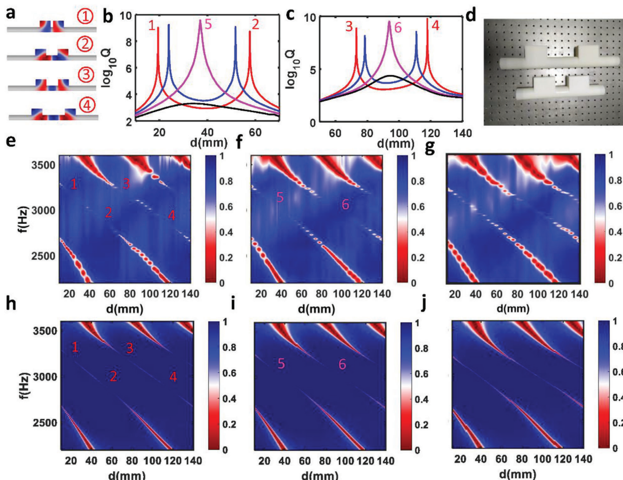
Figure 5. Experimental demonstration of merged BICs in 3D coupled resonator system. a) Pressure field distribution for two antibonding BICs (#1–2) and two bonding BICs (#3–4). b) Q -factor for antibonding mode as a function of distance between two resonators for width L = 61 mm (red), 61.6 mm (blue), 62.212 mm (magenta), and 63 mm (black). The diameter of circular waveguide is 29 mm. c) Q -factor for bonding mode as a function of distance between two resonators for width L = 61 mm (red), 61.6 mm (blue), 62.212 mm (magenta), 63 mm (black). d) Optical image of 3D coupled resonator system fabricated by 3D-printing. e–g) Measured reflection spectrum mapping versus distance between two resonators for the resonator's width e) L = 61 mm, f) L = 62.2 mm, and g) L = 63 mm. h–j) Simulated reflection spectrum mapping versus distance between two resonators for the resonator's width h) L = 61 mm, i) L = 62.2 mm, and j) L = 63 mm.
