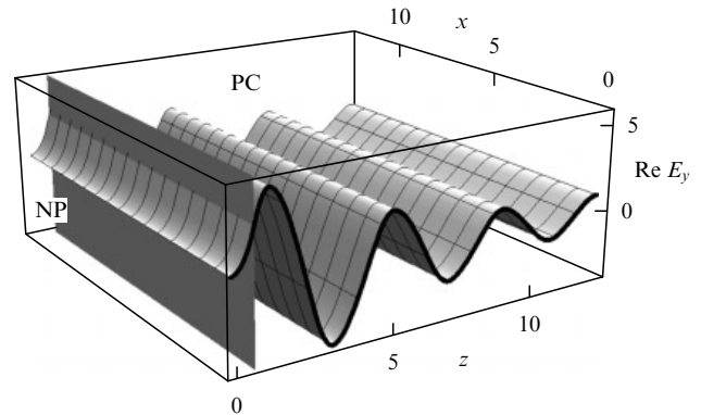
Figure 7. Tamm state at the interface between a PC (for which \varepsilon_1 = 2 , \varepsilon_2 = 1 , d_1 = d_2 = 100 nm, k_0 = 0.0132 nm -1 is the frequency of the Tamm state, and the cell is symmetric \{(\varepsilon_1, d_1/2), (\varepsilon_2, d_2), (\varepsilon_1, d_1/2)\} ) and a medium with \varepsilon_{\text{SNG}} = -3 . The tangential component of the wave is vector k_x = 0 .
