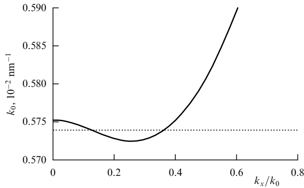
Figure 6. Dispersion curve for a TM-polarized surface state from the first forbidden band of a PC with the cell \{(\varepsilon_1, d_1), (\varepsilon_2, d_2)\} where \varepsilon_1 = 2 , \varepsilon_2 = 10 , d_1 = 200 nm, and d_2 = 100 nm, which has an interface with an NP medium with \varepsilon = -0.1 . The negative slope of the dispersion curve corresponds to a backward wave.
