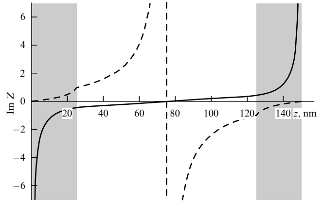
Figure 3. Coordinate dependence of the imaginary part of the impedance within one elementary PC cell of the form \{(e_1, d_1/2), (e_2, d_2), (e_1, d_1/2)\} for the lower (solid curve, frequency k_0 = 0.00807 \text{ nm}^{-1} ) and upper (dashed curve, frequency k_0 = 0.0159 \text{ nm}^{-1} ) edges of the first forbidden band for k_x = 0 . The higher-permittivity layer is shown in dark color. The real part of the impedance is equal to zero because there is no energy transfer. The parameters are \epsilon_1 = 10 , \epsilon_2 = 1 , d_1 = 50 \text{ nm} , d_2 = 100 \text{ nm} .
