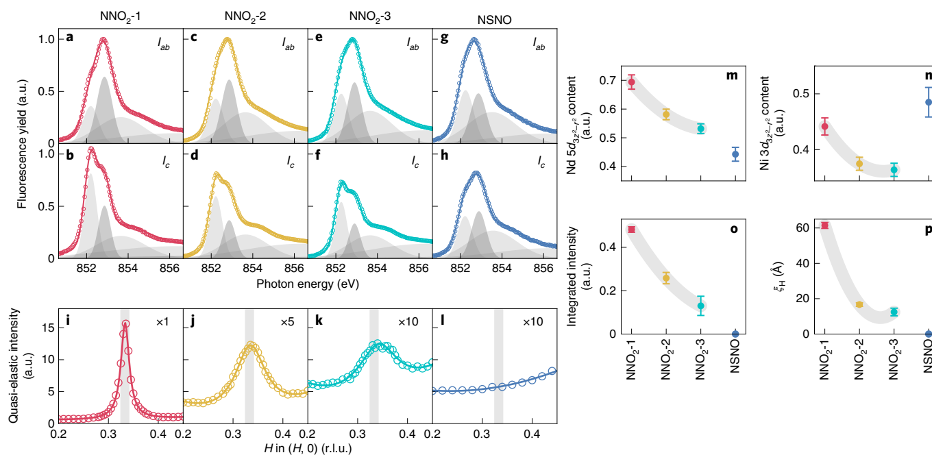
Fig. 2 | Nd 5 d -Ni 3 d orbital hybridization and CDW in NdNiO 2 and superconducting Nd 0.8 Sr 0.2 NiO 2 . a-h , XAS projected in (out of) the NiO 2 planes, I_{ab} ( a,c,e,g ) ( I_c ) ( b,d,f,h ), of NNO 2 -1 ( a,b ), NNO 2 -2 ( c,d ), NNO 2 -3 ( e,f ) and NSNO ( g,h ). The fit components visible in this energy range are plotted in different shades of grey (fitting details provided in Methods). i-l , Quasi-elastic peak intensity showing a CDW plotted in the three NdNiO 2 films with y axis scaled \times 1 , ( i ), \times 5 ( j ) and \times 10 ( k ), with no evidence of CDW in NSNO ( l ). The Nd 5 d 3z 2 -r 2 orbital content ( m ), Ni 3 d 3z 2 -r 2 orbital content ( n ), CDW integrated intensity ( o ) and CDW in-plane correlation length ( p ) show similar trends for the NdNiO 2 samples. Error bars are from least-squares fitting.
