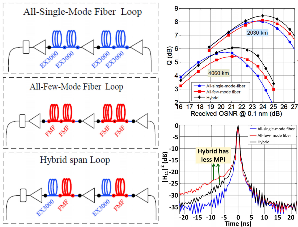
FIG. 4. Experimental demonstration of QSM. 47 Reproduced with permission from Yaman et al. , in Optical Fiber Communication Conference (2015), p. Th5C.7. Copyright 2015 Optical Society of America.
