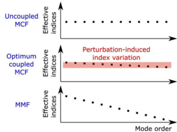
FIG. 1. Illustration of the effective indices for the modes supported by uncoupled MCF, coupled MCF, and MMF.
