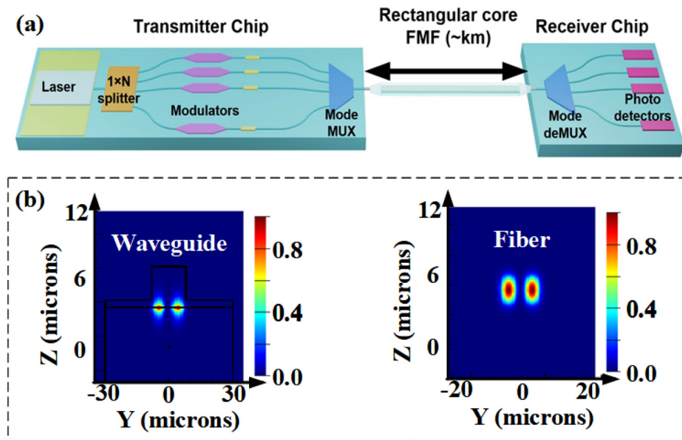
FIG. 3. (a) Schematic configuration of a possible short reach MDM link with fully integrated MUX and deMUX components. (b) Simulated electric field distributions monitored at the edge of an integrated waveguide and an RCF.
