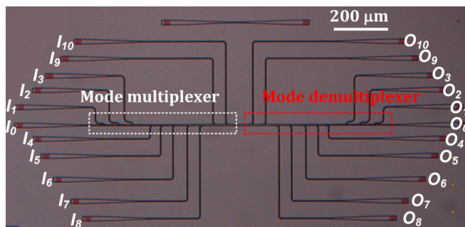
FIG. 2. Microscope image of the 11-channel MDM device. 35 Reproduced with permission from He et al., J. Light. Technol. 36 , 24 (2018). Copyright 2018 IEEE.
