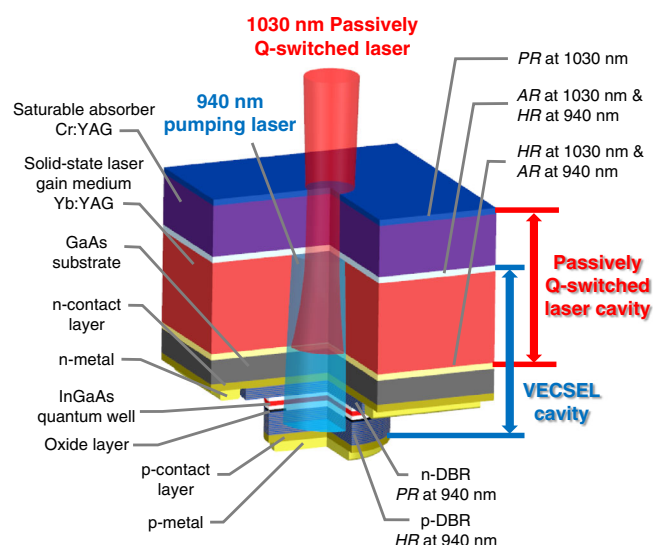
Fig. 1 | Schematic of chip-scale semiconductor/solid-state vertically integrated laser. The VECSEL cavity and the passively Q-switched laser cavity are optically coupled at the solid-state gain medium of Yb:YAG.
