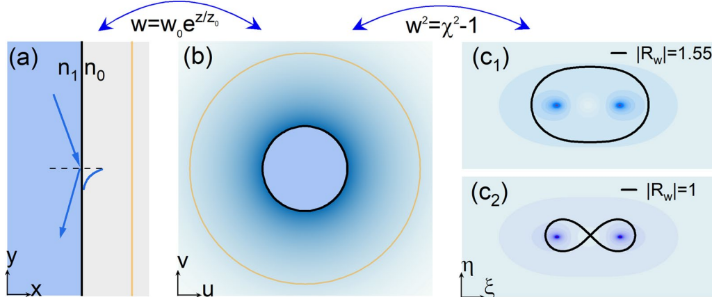
Fig. 1 Conformal transformation for optical black hole (OBH) cavity. Mapping the homogeneous refractive index distribution in the original straight space (a) to a circular OBH cavity (b) with gradient index. The black and orange straight lines in (a) are transformed into the interior and exterior circle. The core region of OBH cavity is truncated as homogeneous index. The quadrupole cavity (c 1 ) and peanut-like cavity (c 2 ) are transformed from the circular OBH cavity under different structural parameters, R_w = \sqrt{u^2 + v^2} . The black curve is the cavity boundary
