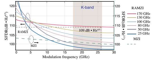
Fig. 5. Simulated SFDR values as functions of modulation frequency for RAMZIs with different FSRs (solid lines), as well as MZI (green dashed line). The 170 GHz RAMZI shows nearly 10 dB improvement over MZI even at a high frequency of 26 GHz, covering the entire microwave K band.
