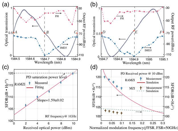
Fig. 4. Detuning and power dependence of the RAMZI modulator. (a), (b) Measured FH (red) and IMD3 (blue) powers at various detuning wavelengths within one FSR when the MZI is biased at (a) \Delta\phi_{\text{mzi}} = \pi/2 and (b) \Delta\phi_{\text{mzi}} = 3\pi/2 , at a fixed input RF power of 15 dBm. Strong suppression of the IMD3 products could be observed at the off-resonance points (B and E). (c) Measured SFDRs at 1 GHz as a function of the received optical powers, with a fitted slope of 1.59 \pm 0.02 in log-log scale. The highest SFDR is measured at a received power of 10 dBm, limited by the PD saturation power (black dash line). (d) Measured and simulated SFDRs at different RF frequencies (normalized by the resonator FSR) for the RAMZI and the reference MZI.
