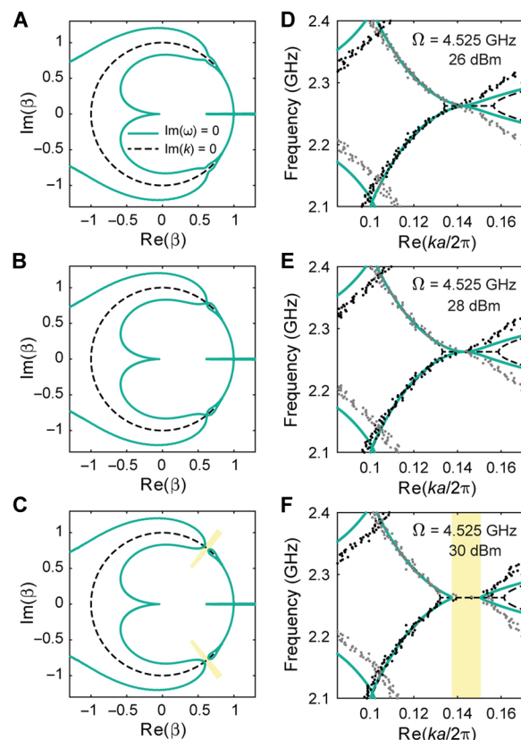
Fig. 5. Comparison between non-Bloch and Bloch-Floquet band structures.
