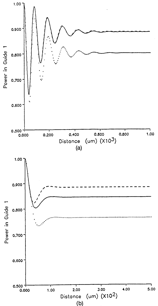
Fig. 15. Guided power in guide 1 as a function of propagation distance L . The parameters are n_1 = n_2 = 3.1 , n_0 = 3.0 , w_1 = 0.8 \mu\text{m} , and w_2 = 0.6 \mu\text{m} . x_{01} = 0.55 \mu\text{m} , and x_{02} = 0.45 \mu\text{m} . The wavelength is \lambda = 1.5 \mu\text{m} . (a) \theta = 0.1^\circ , (b) \theta = 0.5^\circ . Solid curves, nonorthogonal CMT with tapering effect; dashed curves, nonorthogonal CMT that neglects N_{sa} ; dotted curves, nonorthogonal CMT that neglects F_{12} .
