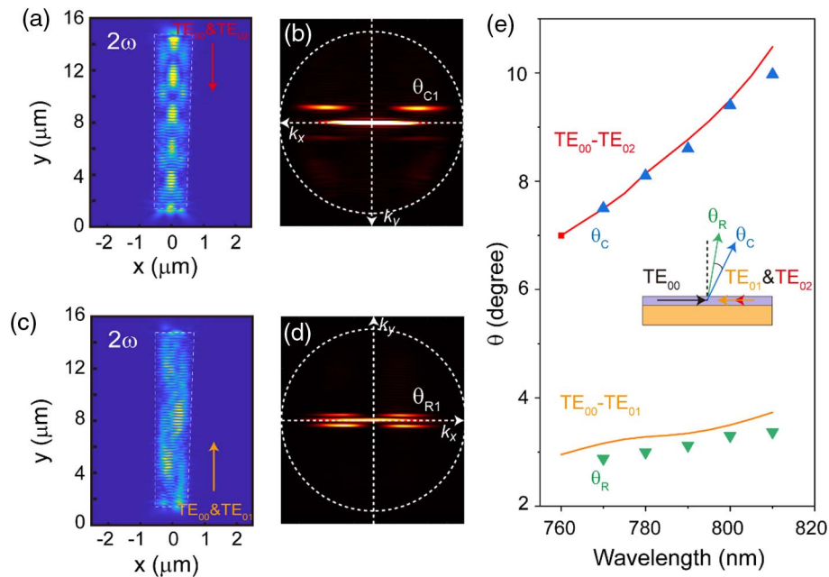
Fig. 4. Steering characters of SHG from the mode-selective excitation. Calculated z -component of the power flux at SH frequency when launching (a) TE_{00} & TE_{02} modes or (c) TE_{00} & TE_{01} modes into the tapered waveguide with a length of 13.4 \mu\text{m} . The distribution of the SH pattern relies on the types of the launched modes. The Fourier images of the SH photons with TE_{00} & TE_{02} modes in (b) and TE_{00} & TE_{01} modes in (d). The outer dashed circle of the Fourier image indicates the collection angle of the objective corresponds to 60^\circ . (e) Measured emission angles of SHG are a function of the fundamental wavelength. \theta_R represents the excitation situation of the fundamental light on the corner of the narrow edge, and \theta_C represents the excitation situation of the fundamental light on the center of the wide edge of the nanobelt. The solid line is the simulated results, and the solid dots are the experiment results.
