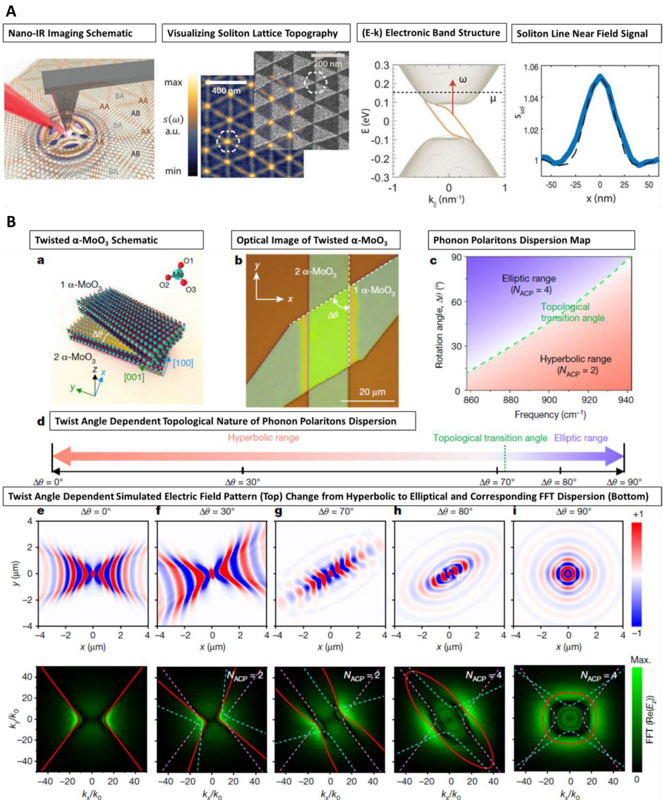
Fig. 6 Photonic superlattices in twisted bilayers. A Nano-light photonic crystal formed by a network of solitons in twisted bilayer graphene. B Rotation-induced topological transition of phonon polaritons in twisted bilayer \alpha -MoO 3 . Reproduced with permission from Refs. [19, 79]
