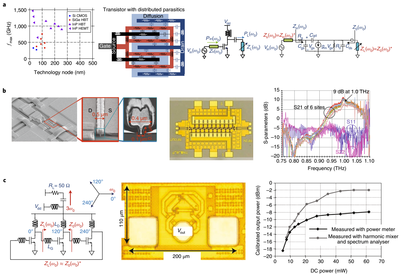
Fig. 2 | High-frequency limits of solid-state devices and THz signal generation. a , The cut-off frequency ( f_{\max} ) of a single device is the frequency at which the optimal power gain falls to unity. f_{\max} of InP HEMT transistors have crossed 1.5 THz, while commercially available silicon THz nodes have crossed 0.5 THz. In the figure, P_{\text{in}}(\omega_0) ( P_{\text{L}}(\omega_0) ), V_{\text{in}}(\omega_0) ( V_{\text{L}}(\omega_0) ) and Z_{\text{in}}(\omega_0) ( Z_0(\omega_0) ) represent the input (output) power, voltage and impedance, respectively. These parameters are related through the small-signal operation of the transistor as depicted in the figure. b , The first solid-state amplifier above 1 THz with InP-based HEMTs with f_{\max} of 1.5 THz (ref. 66 ). c , Fully integrated oscillators operating close to f_{\max} and allowing optimal harmonic power generation beyond f_{\max} in the THz range. The example shows 150 \mu\text{W} of power generation at 0.48 THz with the third harmonic of the fundamental signal in a CMOS technology with f_{\max} of \sim 0.17 THz (ref. 81 ). Panels adapted from: b , ref. 66 , IEEE; c , ref. 81 , IEEE.
