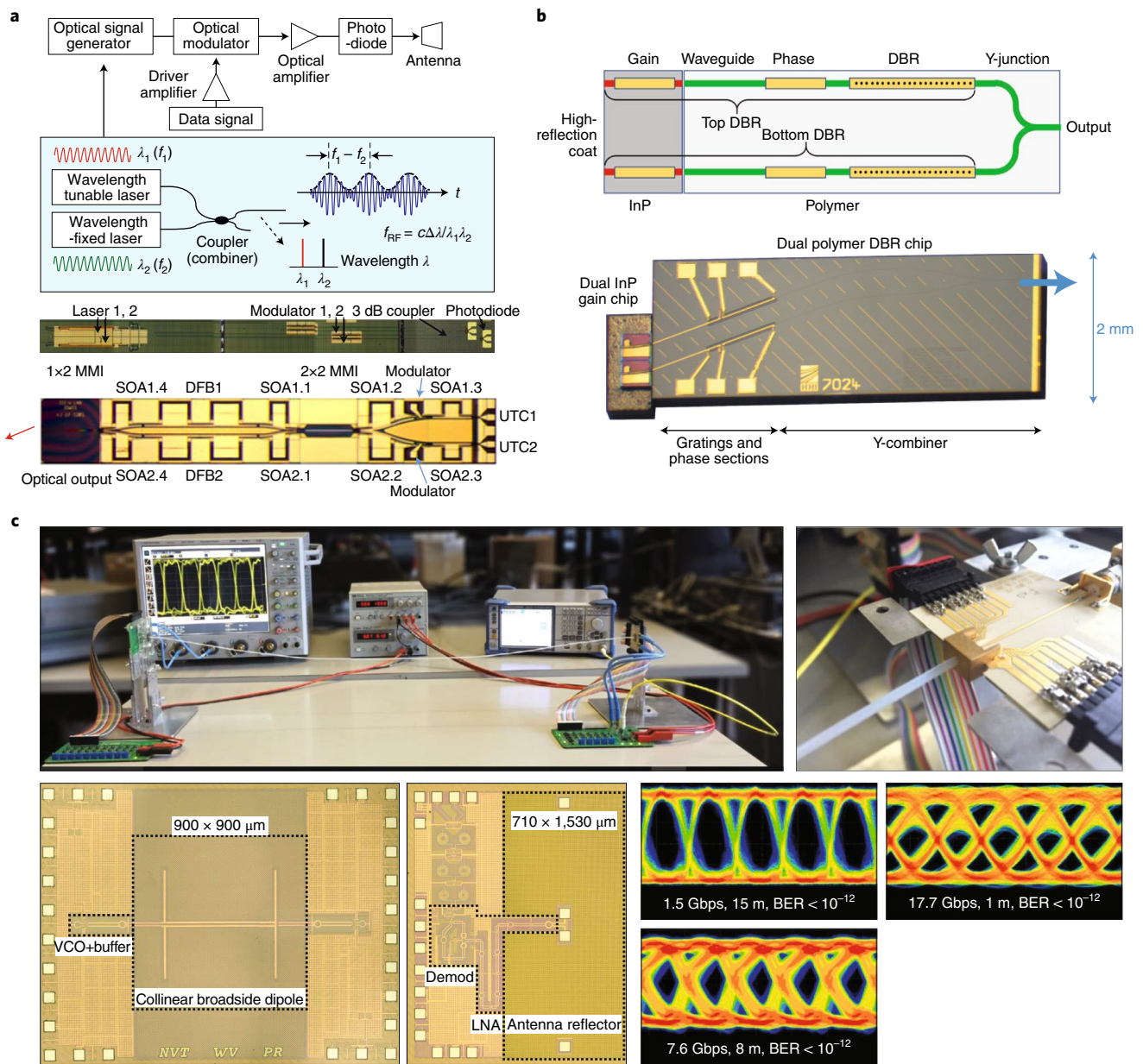
Fig. 6 | Electronic-photonic hybrid THz systems. a , Photonics-based transmitter for THz wireless communications. The chip photographs show a fully integrated microwave and THz signal generator on heterogeneous silicon/III-V (ref. 142 ) and on InP substrates 143 . MMI, multimode interference reflectors; SOA, semiconductor optical amplifier. b , Dual wavelength source chip with hybrid integration. The figure shows the gain sections on InP and various elements on the polymer substrate such as passive waveguides, phase shifters and DBR sections. The photograph shows the dual hybrid InP/polymer DBR 145 . c , Fully integrated CMOS chipsets operating at 0.12 THz with THz plastic waveguides establishing connectivity of 17.7 Gbps over 1 m and 1.5 Gbps over 15 m distance 146,147 . VCO, voltage-controlled oscillator; LNA, low-noise amplifier. Panels adapted from: a , upper chip image, ref. 142 , Optical Society; a , lower chip image, ref. 143 , IEEE; b , ref. 145 , Springer Nature Ltd; c , top-left image and two bottom-left images, ref. 146 , IEEE; c , top-right image and three bottom-right images, ref. 147 , IEEE.
