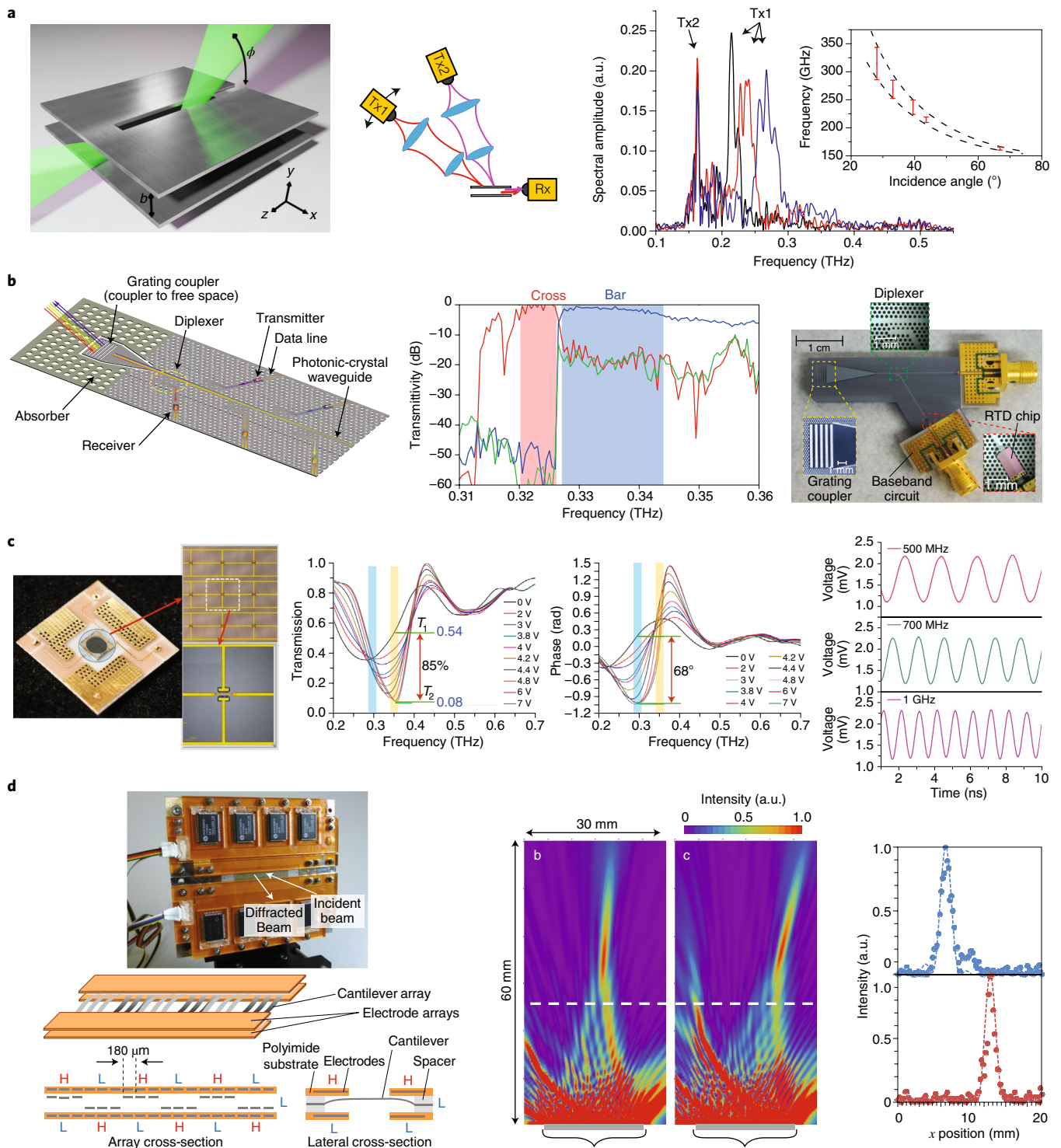
Fig. 5 | Photonics-inspired passive and active THz components. a , Multiplexing of THz signals for distributed signal distribution. Two different transmitters are used to illuminate the waveguide simultaneously with broadband radiation. The multiplexed signal shows two peaks with their centre frequencies determined by the input angles of the two in-coupled beams, respectively 110 . Tx1, transmitter 1; Tx2, transmitter 2; Rx, receiver. b , Photonic-crystal inspired THz diplexer 112 . c , Unit cell of a composite metamaterial-based THz modulator that combines an equivalent collective dipolar array with a double-channel heterostructure for ultrafast and all-electronic THz modulation. The figure also shows frequency-dependent transmission and phase shift of THz time-domain spectroscopy at different voltages and detection of modulated THz waves 126 . d , THz beam forming with a programmable diffraction grating using a linear array of electrostatically actuated cantilevers 29 . H, high; L, low. Panels adapted from: a , ref. 110 , Springer Nature Ltd; b , ref. 112 , Optical Society; c , ref. 126 , American Chemical Society; d , ref. 129 , Optical Society.
