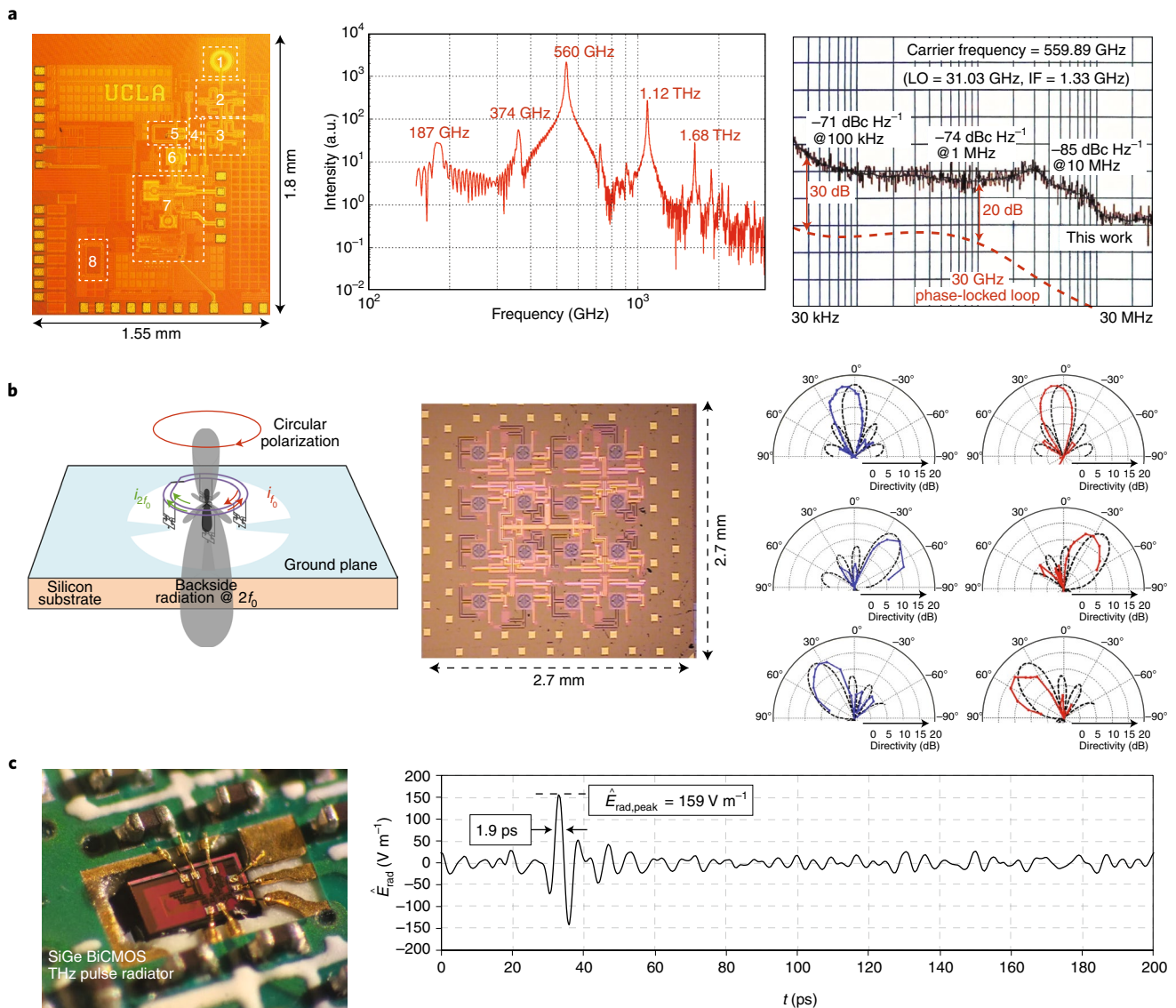
Fig. 3 | THz sources and systems in silicon. a , Fully integrated THz phase-locked loops in CMOS where the fundamental and the harmonic signal (at 0.56 THz) is locked to an external low phase-noise reference 83 . LO, local oscillator; IF, intermediate frequency. b , Multifunctional active electromagnetic structures allowing direct conversion of d.c. power to generation and radiation of filtered THz harmonic signal 76 . i_{f_0} and i_{2f_0} represent the filtered fundamental and radiated second harmonic currents, respectively. A 4x4 array in a single chip demonstrated THz phased array operation at 0.28 THz. In the rightmost panel the dashed and solid lines represent simulated and measured data, respectively. c , THz picosecond pulse generator in silicon that allows direct digital-to-THz impulse conversion and radiation with on-chip antennas 89 . \hat{E}_{\text{rad}} represents the radiated electric field at a distance of 1 cm from the chip. Panels adapted from: a , ref. 83 , IEEE; b , ref. 76 , IEEE; c , ref. 89 , IEEE.
