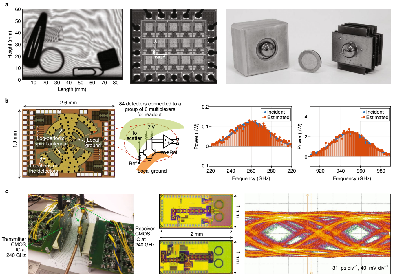
Fig. 4 | THz sensors and receivers in silicon. a , One of the earliest demonstrations of THz imaging in silicon with a 3x5 pixel array in 0.25 \mu\text{m} CMOS operating at 0.65 THz (ref. 97 ). The figure also shows a 1,000 pixel THz camera operating in video mode from 0.7 to 1.0 THz (ref. 78 ). b , Integration of active devices and antennas on the same substrate allows new chip-scale architectures that can exploit deep subwavelength sensing. The figure shows a single-chip THz spectroscopy that extracts incident THz spectral information from spatial sensing of scattered fields with integrated devices. Eliminating all complex THz sources, the chip employs regression analysis to allow source-free spectral estimation across 0.04–0.99 THz (refs. 102,103 ). c , Fully integrated silicon transceivers operating at 0.24 THz with data rates approaching 16 Gbps with phase modulation schemes such as QPSK 105 . Panels adapted from: a , left and middle images, ref. 97 , IEEE; a , right image, ref. 78 , IEEE; b , ref. 103 , Optical Society; c , ref. 105 , IEEE.
