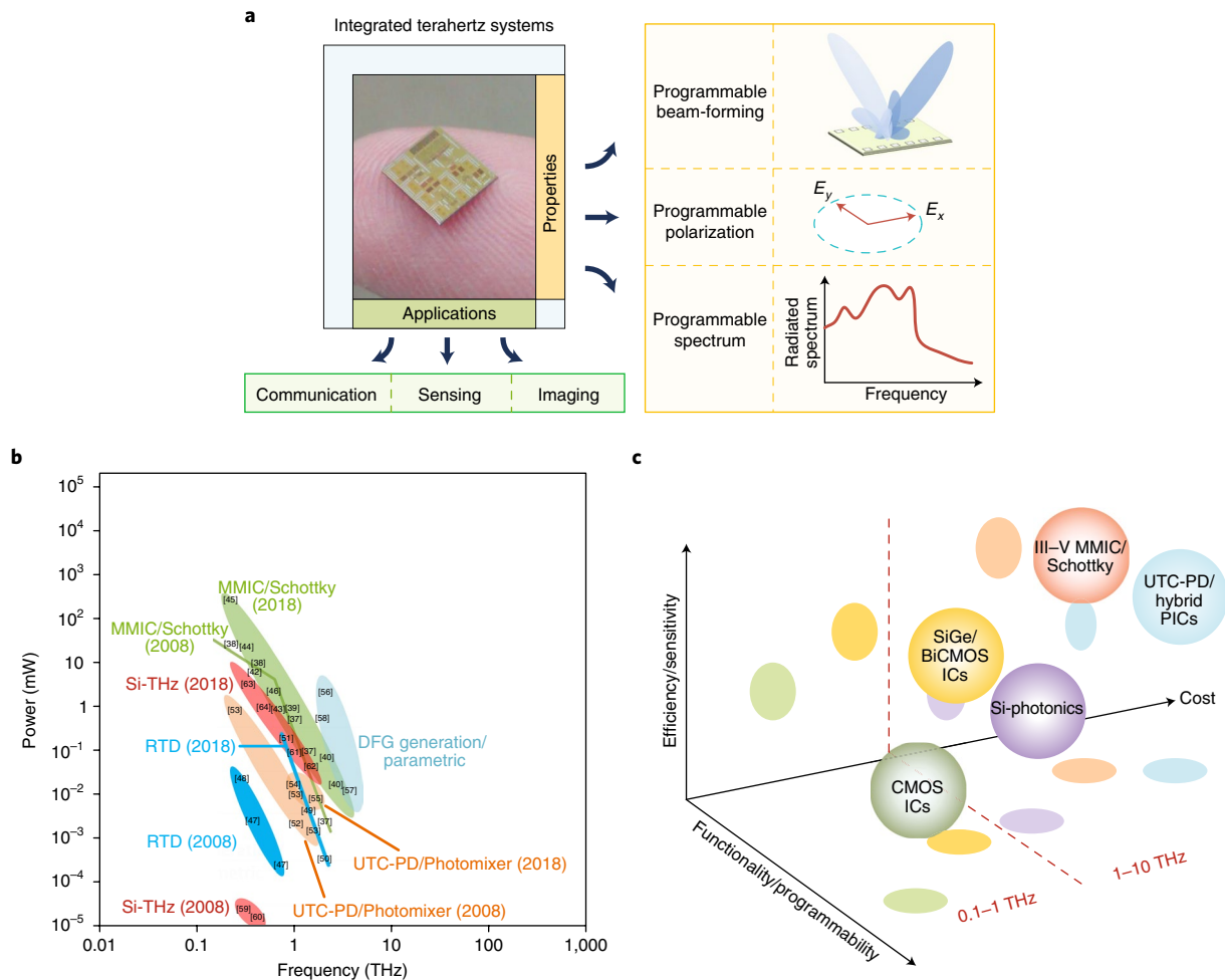
Fig. 1 | Integrated THz systems and the technology landscape. a , Moving the focus from a device-centric approach to enabling complex THz systems that might have moderate efficiency but that are versatile and programmable. This includes properties such as the ability to synthesize or sense THz fields in a reconfigurable manner across spectrum and spatial distribution. Such systems that can be manufactured at low cost and operate at room temperature can be an extremely powerful tool to significantly advance the application space, particularly in imaging and sensing where single modality is often not sufficient. b , Progress of THz sources in the past decade showing how a selected set of integrated THz technology has evolved over the past ten years in its ability to generate continuous-wave THz signals at room temperature. The panel is adapted from ref. 2 , Springer Nature Ltd, which designated the state-of-the-art technology in 2007. MMIC, microwave monolithic integrated circuits; RTD, resonant tunnel diodes; DFG, difference frequency generation. Numbers in square brackets are reference citations. c , While some technologies are better placed than others purely from a signal-generation perspective, there are other considerations that go behind evaluating the optimal THz technology. This includes efficiency, ability to reconfigure the spectrum and field distribution, cost and scalability. A qualitative illustration of technologies in this multidimensional space is captured in the figure. ICs, integrated circuits; UTC-PD, uni-travelling-carrier photodiode; PICs, photonic integrated circuits.
