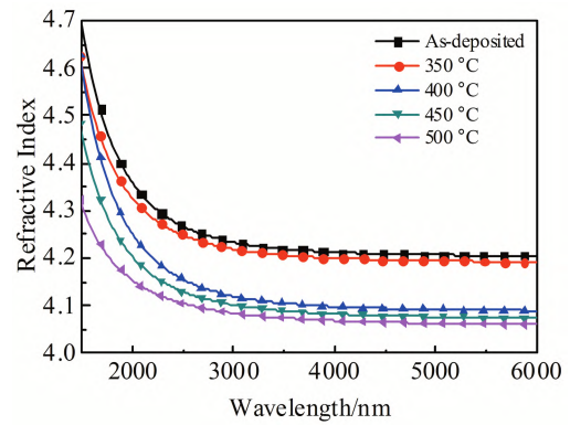
Fig.3 Effect of annealing temperature on refractive index of Ge film
