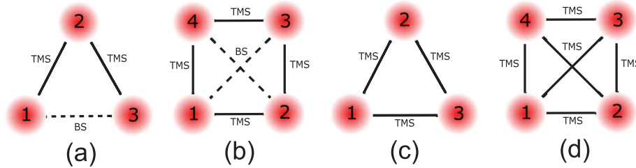
Figure 2. Graph representation for the entangled tripartite and quadripartite systems. Generalized H-graph ( \mathcal{H} -graph) representation of a) bisqueezed tripartite CV entangled state and b) quadripartite CV entangled \mathcal{H} -graph state obtained in our experiments. Vacuum modes (red circles) are connected via two-mode squeezing (TMS, solid lines on graph) and beamsplitter (BS, dashed lines) correlation. Graphs (c,d) represent tri- and quadripartite GHZ states, which can be obtained via introducing an additional pump tone with \Delta_d = 0 in the tripartite case and two additional tones at -\Delta and \Delta in the quadripartite setting. The additional pumps supply missing TMS connections to the entangled states. For details, see Appendix A.6.
