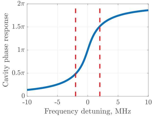
Figure A3. Cavity phase response given by fitted experimental parameters \frac{\Gamma_c}{2\pi} = 4.44 MHz and \frac{\gamma}{2\pi} = 2.30 MHz. Vertical dash lines show center frequencies of first and last modes. Corresponding phase shifts applied to pump tones to reach “symmetric” covariance matrix view on double frequencies are \Delta\varphi_1 = \frac{\pi}{2} - \frac{\pi}{4} = \frac{\pi}{4} and \Delta\varphi_2 = \frac{\pi}{2} + \frac{\pi}{4} = \frac{3\pi}{4} with corresponding phase shift between pump tones \frac{\pi}{2} , given in results (see Figure 4). Half of applied phase shift described by pump tones on double resonance frequencies. Additional phase shift with increase of A relates to modification of phase response curve during pumping.
