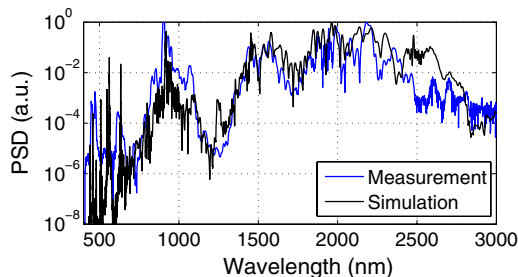
Fig. 3. (Color online) Power spectral density of the PPLN waveguide SC. Measurements above and below 1750 nm were performed with an FTIR and an OSA, respectively.
