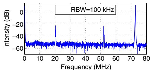
Fig. 4. (Color online) RF spectrum at 796 nm (filtered via a grating spectrometer) measured on a silicon APD, showing f_{\text{CEO}} at 52 MHz and the repetition rate at 72 MHz.
