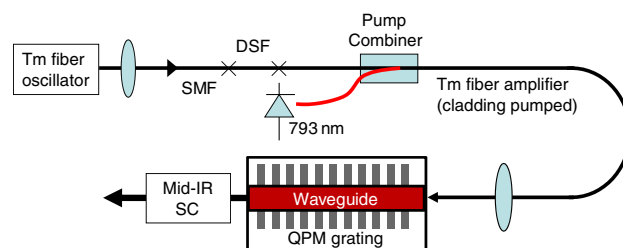
Fig. 1. (Color online) Setup of a self-referenced Tm-doped fiber and PPLN waveguide system. SMF, single-mode fiber; DSF, dispersion-shifted fiber.
