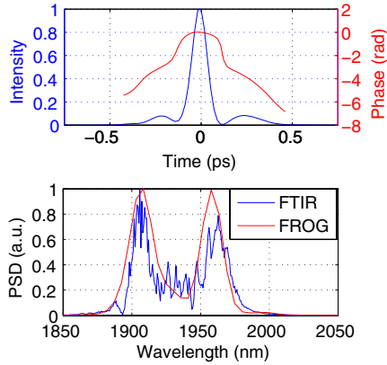
Fig. 2. (Color online) Amplified pulse characterization. (a) Time-domain amplitude and phase profile based on SHG FROG. (b) Pulse spectrum measured with an FTIR (blue) and reconstructed via the FROG algorithm (red).
