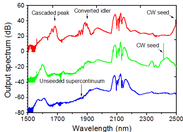
Fig. 4. Measured output spectra obtained while seeding the supercontinuum at a wavelength of 2415 nm (green) and 2496 nm (red), using a CW mid-infrared laser. The blue curve shows the unseeded output spectrum as a reference. The coupled peak power is 12.7 W in all cases. The spectra are vertically offset by multiples of 40 dB for clarity.
