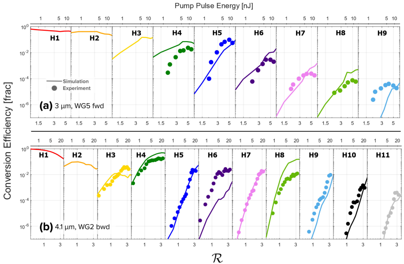
Fig. 6. Harmonic power scaling in terms of both the simulated \mathcal{R} \equiv L_{\text{GVM}}/L_{\text{NL}}^{(2)} (bottom axes, lines) and experimental pump-pulse energy (top axes, dots) for (a) 3 \mu\text{m} , Waveguide 5, forward, and for (b) 4.1 \mu\text{m} , Waveguide 2, backward, with 4.1 \mu\text{m} experimental data from [26]. Both experiments show saturation of harmonics at \mathcal{R} \approx 3 .
