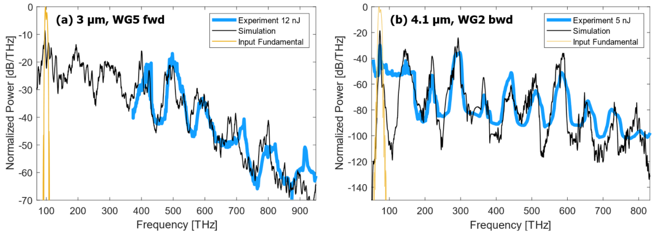
Fig. 5. (a) Overlay of simulated output spectrum (thin black line) and input pump spectrum (thin yellow line) having \mathcal{R} = L_{\text{GVM}}/L_{\text{NL}}^{(2)} = 5.74 with experimental data (thick blue line) for 3 \mu\text{m} , 12 nJ pumping in Waveguide 5, forward. (b) Idem for 4.1 \mu\text{m} pumping in Waveguide 2, backward with \mathcal{R} = 1.57 and 5 nJ experimental pulse energy. Experimental data in (b) is from the study first reported in [26].
