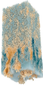
Simulated volumetric rendering of the instantaneous fluid velocity field (blue for upward, orange for downward) produced by the gravitational settling of heavy particles (spheres) in a Rayleigh-Taylor-like setup. [S. Tandurella et al. , Phys. Rev. Lett. 136 , 104003 (2026)]
