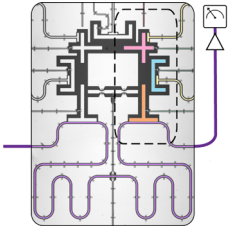
Passive PT dimer experiment using superconducting qubits. [A. Almanakly et al. , Phys. Rev. Lett. 136 , 183601 (2026)]
