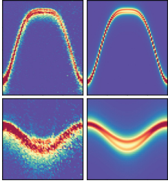
Magnon dispersions in \text{FeF}_2 along two reciprocal-space directions (top and bottom rows), measured by inelastic neutron scattering (left) and reproduced by spin-wave simulations (right). Selected for an Editors' Suggestion. [J. Sears et al. , Phys. Rev. Lett. 136 , 226701 (2026)]
