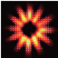
Far-field lasing pattern from the q = -4 microcavity. The overlaid line segments represent polarization vectors. [X. Bi et al. , Phys. Rev. Lett. 137 , 016901 (2026)]
