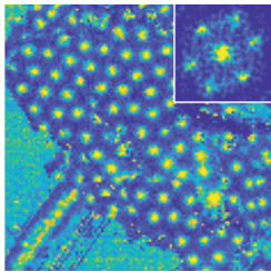
Scanning tunneling conductance map of a superconducting vortex lattice, with its corresponding Fourier transform in the inset. Selected for an Editors' Suggestion. [J. A. Moreno et al. , Phys. Rev. Lett. 137 , 086001 (2026)]
